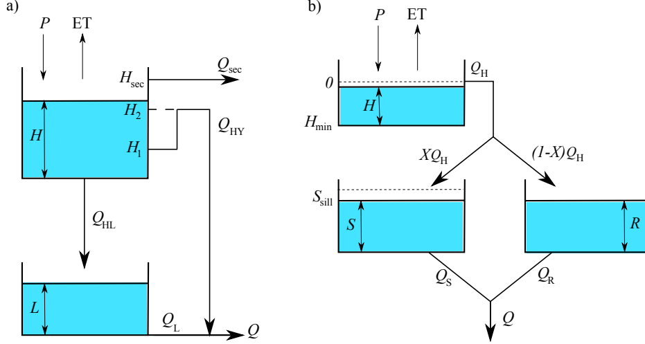
Figure 2.3: Structure and notations for: a) the hysteresis-based model [Tritz et al., 2011], b) the Vensim model [Fleury, 2005].
