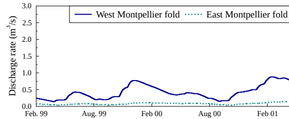
Figure 6.9: Simulation results for the transient state simulation. Discharge rate through the Montpellier fold.
