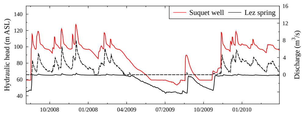
Figure 5.14: Hydrodynamic continuity between the Lez spring and the Lirou subsystem: water levels at the Suquet well and within the Lez karst conduit (solid lines, left y -axis) and Lez spring discharge (dotted line, right y -axis) as a function of time. The Suquet well is drilled directly within the Lirou karst conduit system. A pumping test is performed at the Suquet well during Sept. 2009. See wells location in Figure 5.15.
