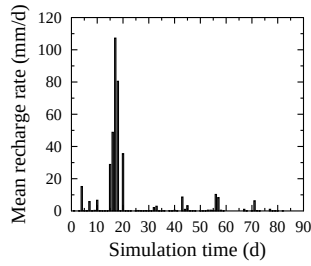
Figure 7.18: Non-parallel, transient mixed confined-unconfined flow. Case of a perturbation in the hydraulic conductivity. Mean daily recharge rate over the Lez aquifer during the simulation period.
