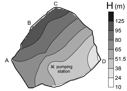
Figure 7.14: Steady state piezometric map of the Lez model.
