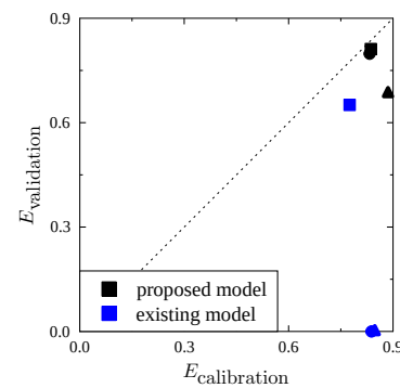
Figure 4.17: Existing model. Split sample test results. Model performance for the calibration ( x -axis) and validation ( y -axis) periods. Calibration on the P_1 , P_2 and P_3 period are denoted by square, triangle and circle markers respectively. See discussion in Sections 4.4.3 (proposed model) and 4.5.2 (existing model).
