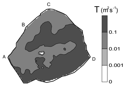
Figure 7.15: Steady state transmissivity map of the Lez model. The zero transmissivity at the centre of the model is due to a zero aquifer thickness.
