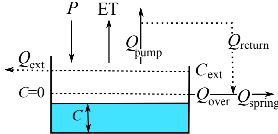
Figure 4.22: Structure and notation for the 1-reservoir, 4-parameters model proposed by Fleury, 2011 (personal comm.).
