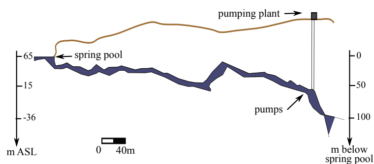
Figure 5.9: Lez spring: Simplified topography. Original topography by P. Rousset (G.E.P.S diving group, 1972).
