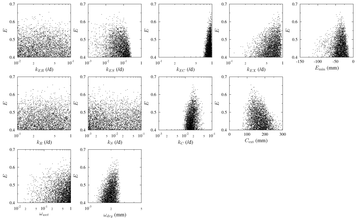
Figure 4.12: Existing model. Dotty plot resulting from model realisations, with the E measure on the y -axis and the parameter values on the x -axis. Calibration against joint discharge and water level data.
