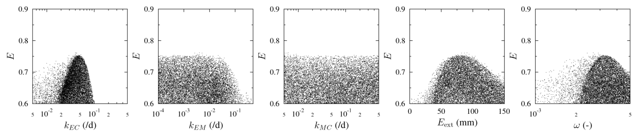
Figure 4.21: Modified version of the proposed model. Dot plot resulting from model realisations, with the E indicator on the y -axis and the parameter values on the x -axis. Calibration against joint discharge and water level data.
