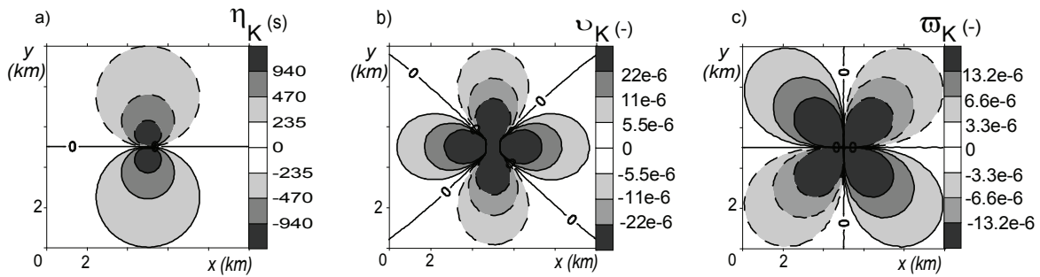
Figure 7.9: Parallel, steady-state confined flow. Case of a perturbation in the hydraulic conductivity : a) sensitivity of the hydraulic head, b) sensitivity of the longitudinal flow velocity, c) sensitivity of the transverse flow velocity. Dashed and solid lines indicate negative and positive values respectively. The simulation parameters are given in Table 7.1 and Table 7.2.
