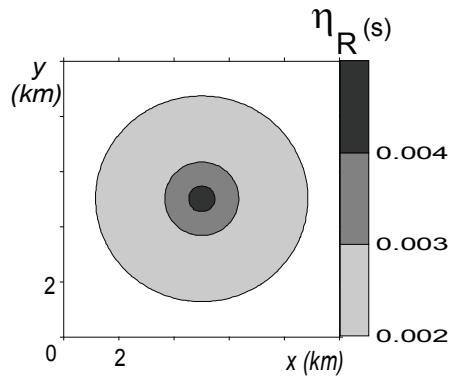
Figure 7.10: Parallel, steady-state confined flow. Case of a perturbation in the recharge rate: hydraulic head sensitivity. The simulation parameters are given in Table 7.1 and Table 7.2.
