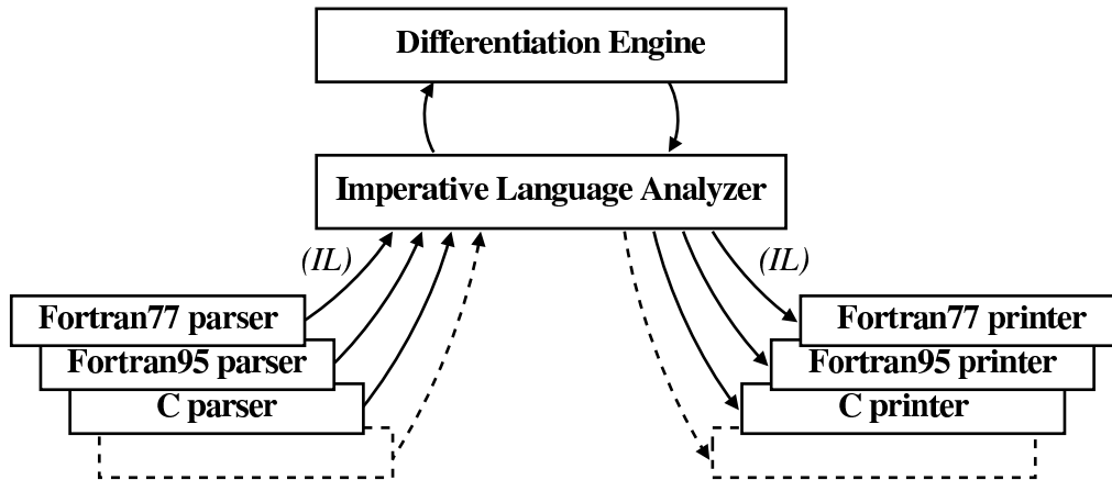
Figure 4.1: Overall Architecture of TAPENADE
