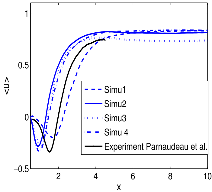
Figure 3.4: Time-averaged streamwise centerlined velocity at Re_\tau = 3900
