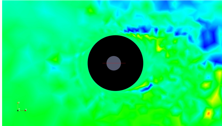
Figure 5.2: Numerical dissipation quantification: (E_0(W_h) - E_1(W_h))
