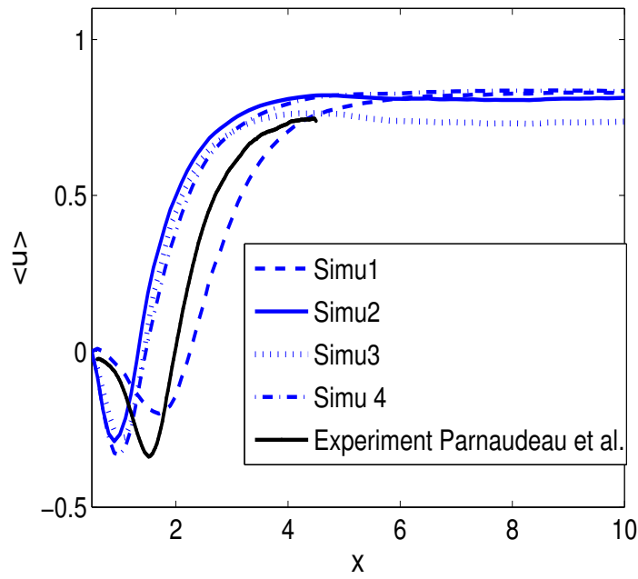
Figure 3.4: Time-averaged streamwise centerlined velocity at Re_\tau = 3900
