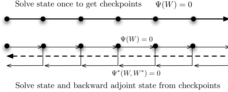
Figure 4.3: Checkpoint algorithm for discrete adjoint state computation
