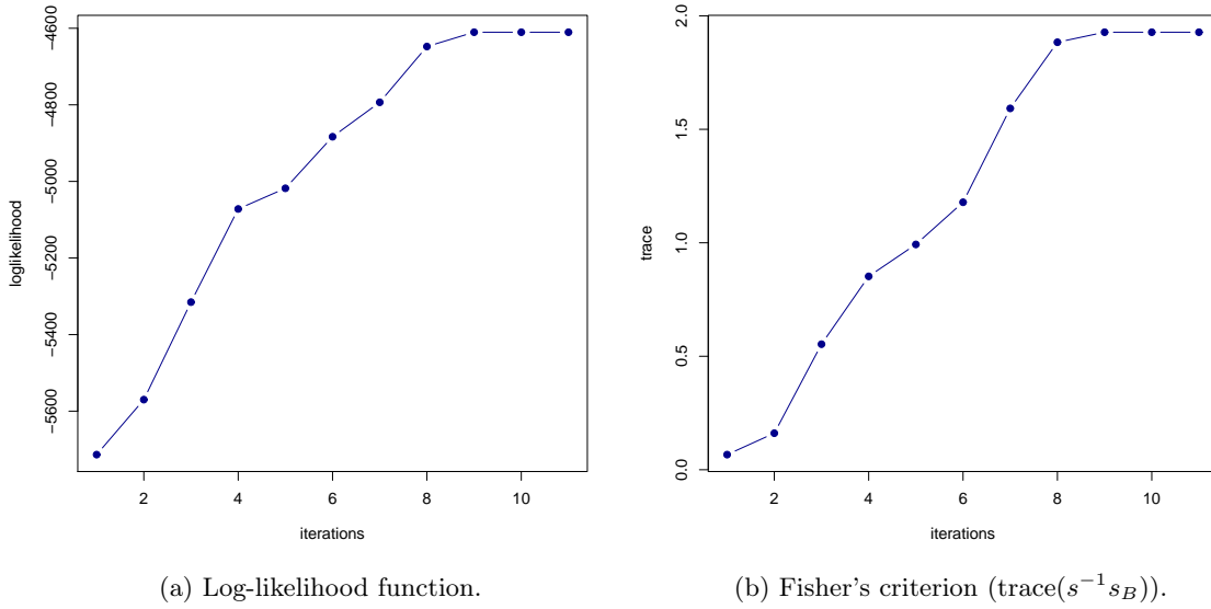
Figure 5.4: Evolution of the loglikelihood function (a) versus Fisher's criterion (trace( s^{-1}s_B )) evaluated in the latent space (b) according to the iterations of the Fisher-EM algorithm.
