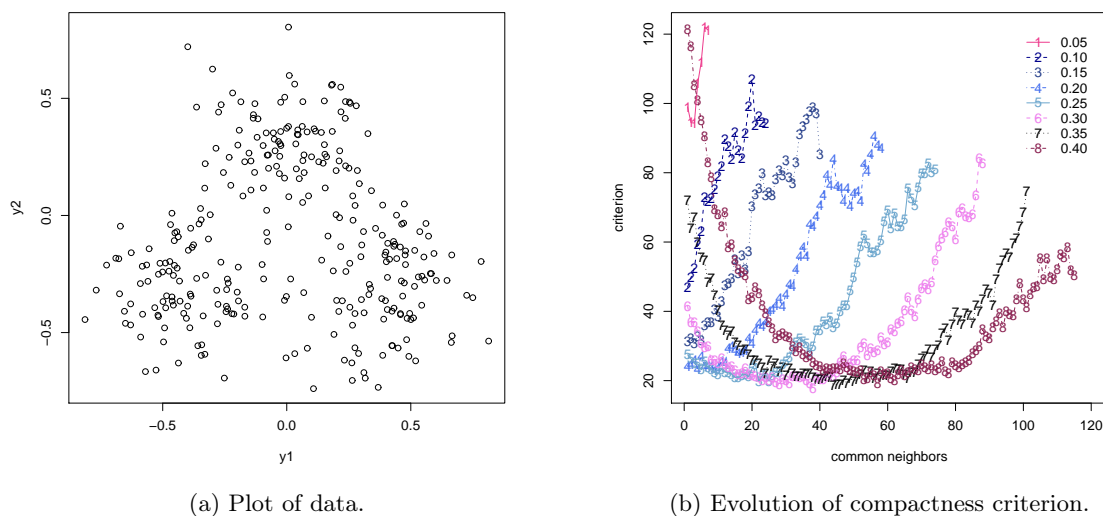
Figure 9.1: (a) Plot of simulated data in their 2-dimensional space and (b) evolution of the behavior of the compactness criterion with respect to the \epsilon -neighborhood and the \lambda -level of common neighbors.
