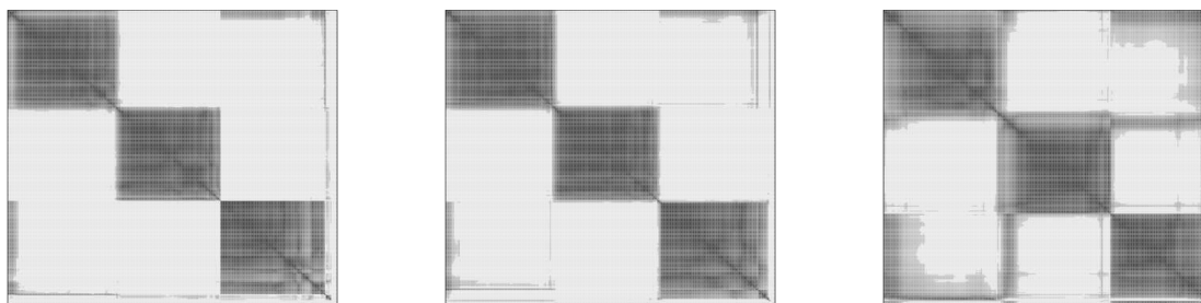
(d) Rearranged \lambda -matrix selected with an \epsilon -neighborhood fixed \epsilon = 0.25 ( \lambda = 25 ). (e) Selected rearranged \lambda -matrix by the compactness criterion ( \epsilon = 0.3, \lambda = 38 ). (f) Rearranged \lambda -matrix with \epsilon = 0.40 selected by the compactness criterion ( \lambda = 57 ).
