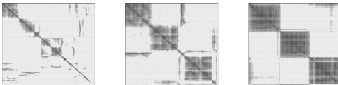
(a) Rearranged \lambda -matrix with \epsilon = 0.05 selected by the compactness criterion ( \lambda = 2 ). (b) Rearranged \lambda -matrix with \epsilon = 0.10 selected by the compactness criterion ( \lambda = 1 ). (c) Rearranged \lambda -matrix with \epsilon = 0.20 selected by the compactness criterion ( \lambda = 10 ).
