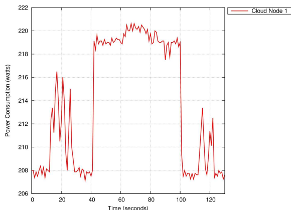
Figure 6.2: Life of a Virtual Machine: boot, run, and halt.
