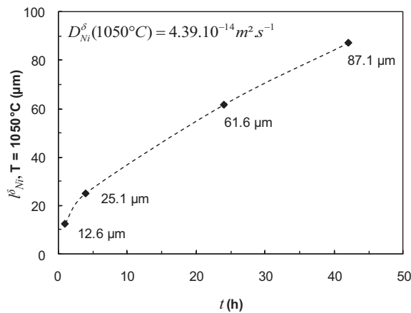
Figure III.28. Evolution of the Ni-diffusion length in the ferrite as a function of time at T = 1050^{\circ}\text{C} .
