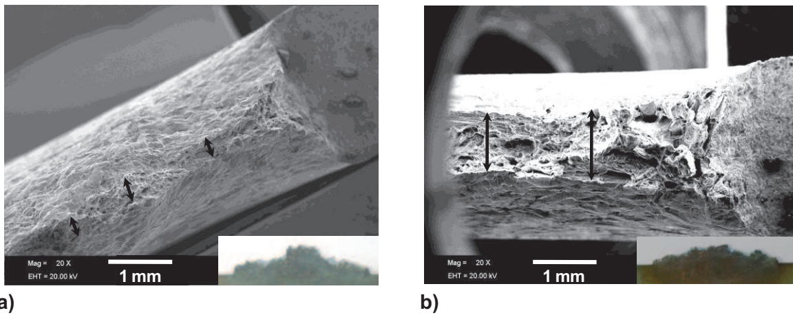
Figure III.33. Fracture micrographs of the broken DENT at 1050°C; a) D1_W ( l_0=35\text{mm} ); b) D2_W ( l_0=37\text{mm} ).
