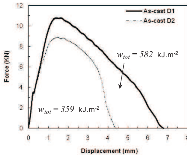
Figure III.11. Typical load-displacement curves at T= 1050°C for each duplex steel grade, for a DENT specimen with ligament length l_0 = 25 mm.
