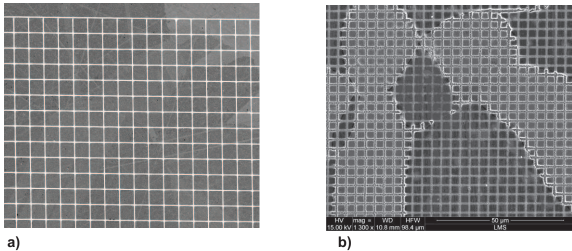
Figure IV.2. 5µm-microgrid patterns [103]; a) processing by micro-lithography; b) engraving by chemical etching from this work.
