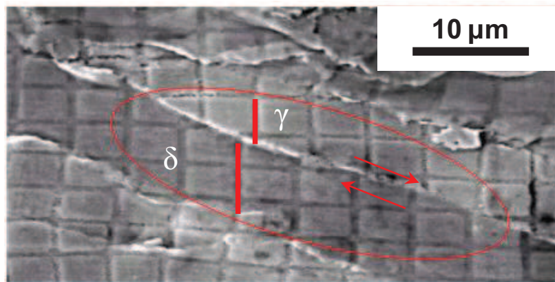
Figure II.4. A clear example of interphase boundary sliding in a 2205 duplex stainless steel deformed to 0.15 at 1050°C and 1s -1 [14].
