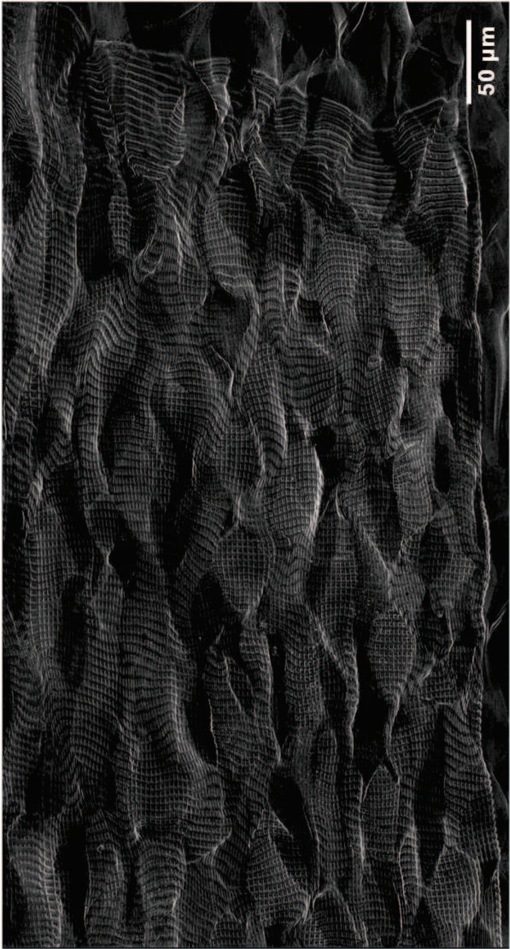
Figure C. 14. Microgrid of the D1_E microstructure from sample B after plane strain compression at 850°C.
