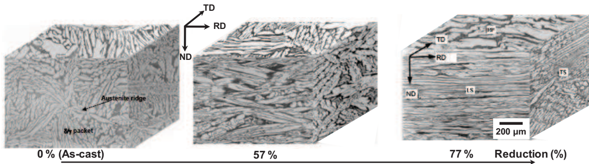
Figure II.2. Evolution in 3D of the as-cast microstructure with the applied rolling reduction of the duplex microstructure; as the deformation proceeds, austenite becomes more and more elongated in the rolling direction (RD) [11].
