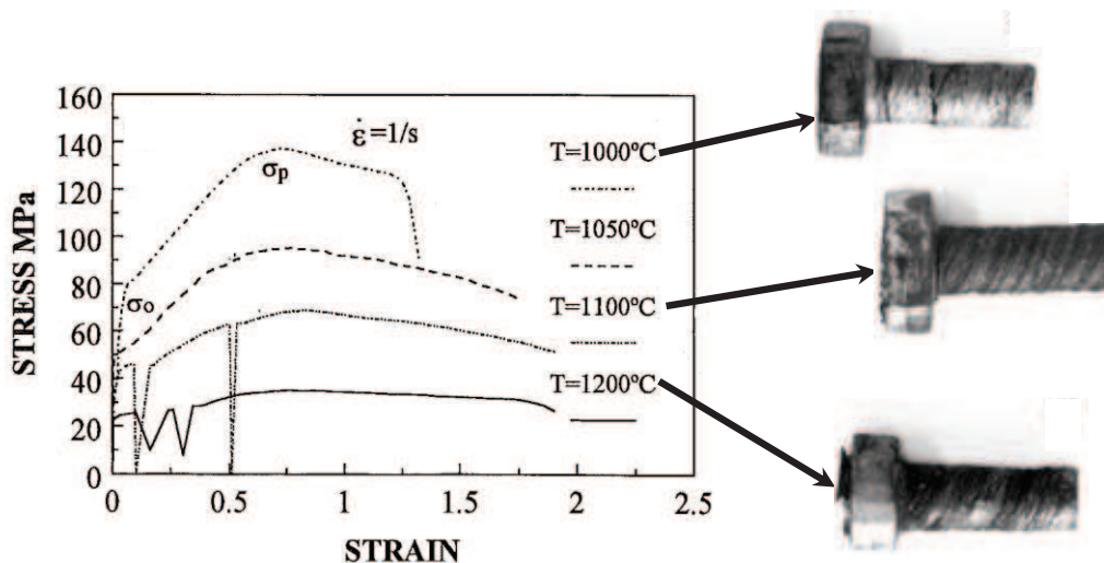
Figure II.23. Stress strain curves of a hot rolled 2304 grade deformed under torsion at different temperatures at 1\text{s}^{-1} and the corresponding deformed specimens showing different levels of damage [25].
