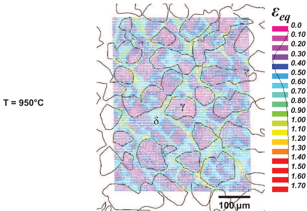
Figure IV.37. Equivalent strain distribution maps of the equiaxed morphology: D1_E at T = 850 and 950°C for a 20% macroscopic thickness reduction; a) strain map at T = 850°C; b) strain map at T = 950°C. The equivalent strain map is superimposed with the undeformed microstructure to clearly present where in the microstructure the strains are distributed. The loading direction corresponds to the vertical axis.
