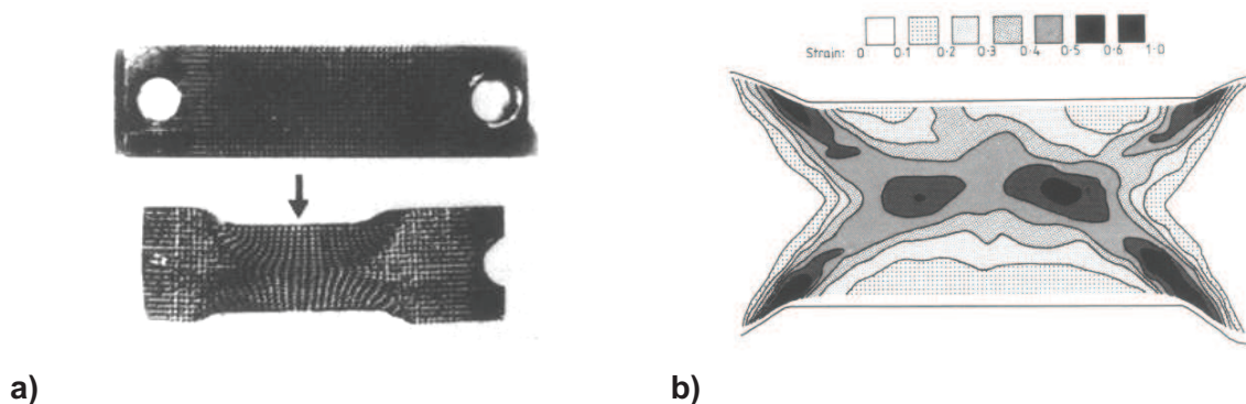
Figure IV.34. Investigation of the strain heterogeneity during plane strain compression test with the engraved grid technique, nominal strain = 0.33 and w/h_0 = 2 ; a) engraved grid before and after deformation; b) average equivalent strain distribution [132].
