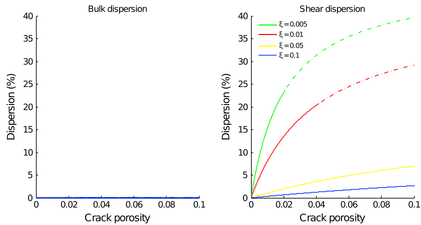
Fig. 4. Numerical results obtained with only cracks added in the EM model. No bulk dispersion is calculated whereas the shear dispersion increases with the crack fraction leading to an asymptotic value. Moreover the smaller aspect ratio, the higher shear frequency dispersion.
