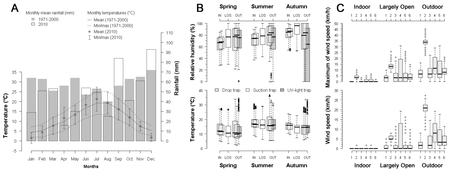
Figure 2: Climatic conditions in the study site: A. Ombrothermic diagram for comparison between 2010 and the 1971-2000 period (data from Météo-France station of Parçay-Meslay); B. Boxplots of temperature (°C) and relative humidity (%) recorded by data loggers at each location during the 15 collection sessions; C. Boxplots of mean and maximum wind speed (km/h) recorded by the local weather station during each of the 6 summer collections.
