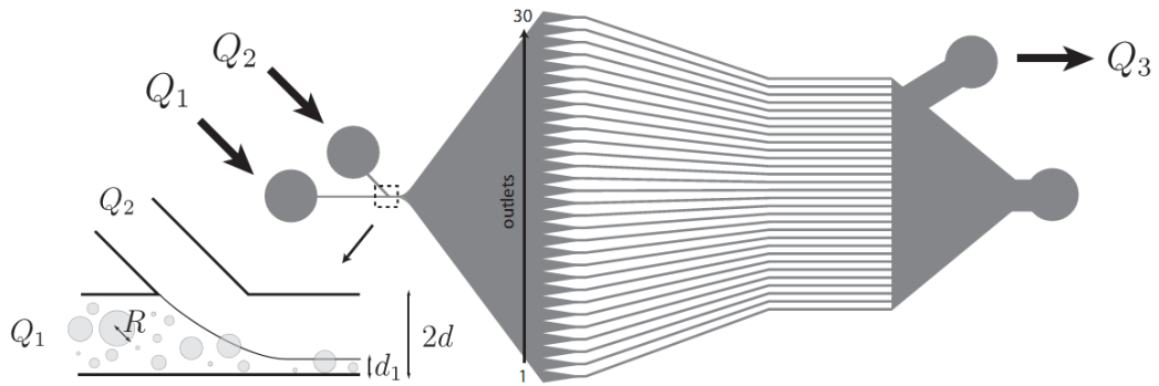
Figure 4.4: Schematic of sorting device
