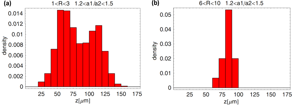
Figure 6.2: Steady distribution of (a) small and (b) large vesicles with no viscosity contrast. z is the distance between two plates that are separated by 180 \mu\text{m} , R is the radius of vesicle and a_1/a_2 aspect ratio [90]
