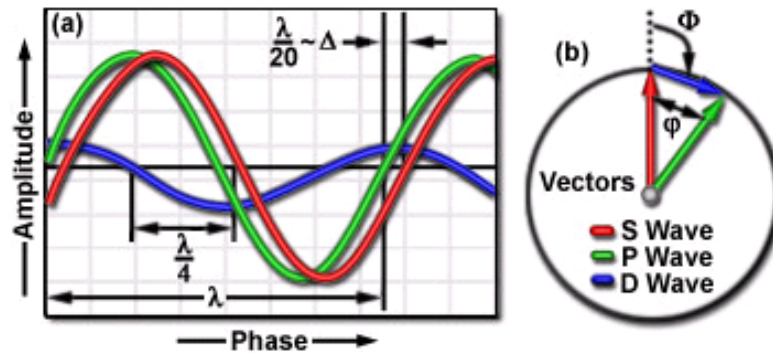
Figure 3.13: Bright field microscope wave phase relationships
