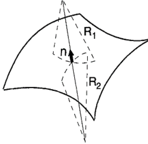
Figure 3.8: Curvature on a 2D surface. The vector \vec{n} denotes the normal vector [5]
