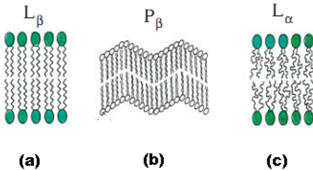
Figure 3.4: (a) Crystalline Phase; (b) Ripple Phase; (c) Liquid-phase
