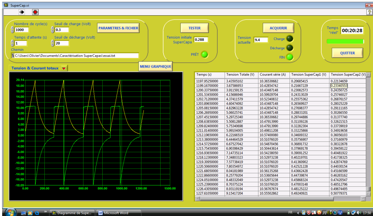
Figure 3.6. – Interface Labview.
