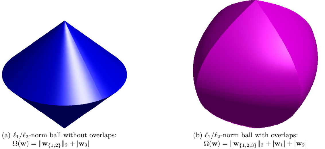
Figure 1.3: Comparison between two mixed \ell_1/\ell_2 -norm balls in three dimensions, without and with overlapping groups of variables, respectively on the left and right figures. The singular points appearing on these balls describe the sparsity-inducing behavior of the underlying norms \Omega .
