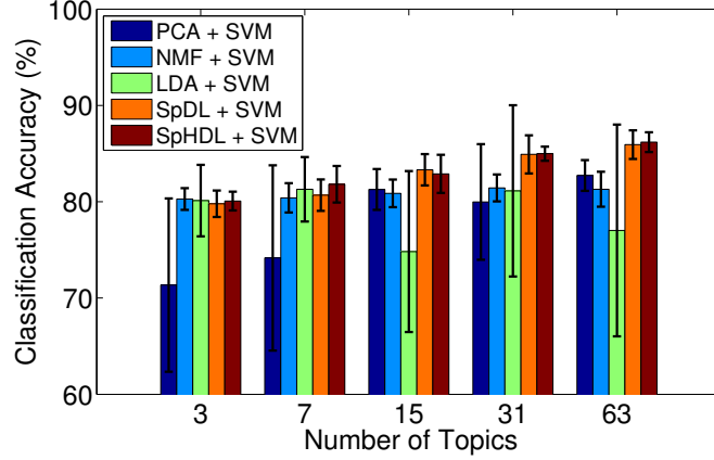
Figure 4.11: Binary classification of two newsgroups: classification accuracy for different dimensionality reduction techniques coupled with a linear SVM classifier. The bars and the errors are respectively the mean and the standard deviation, based on 10 random splits of the dataset. Best seen in color.
