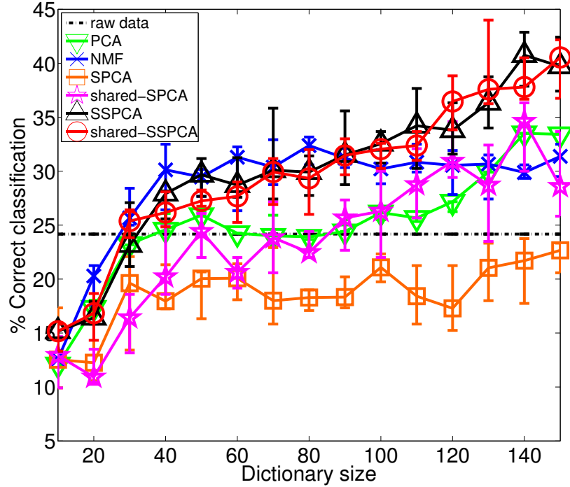
Figure 3.4: Classification accuracy versus dictionary size: each dimensionality reduction technique is used with k-NN to classify occluded faces. SSPCA shows better robustness to occlusions. The points, lower and upper error bars on the curves respectively represent the median, first and third quartile, based on 10 runs.
