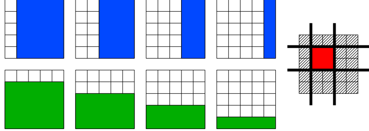
Figure 2.5: Vertical and horizontal groups: (Left) the set of blue and green groups with their (not displayed) complements to penalize in order to select rectangles. (Right) In red, an example of nonzero pattern recovered in this setting, with its corresponding zero pattern (hatched area).
