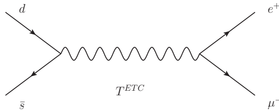
Figure 1.7: Feynman Diagram of the exchange of a quark pair into a lepton pair via an ETC gauge boson leading to a FCNC interaction.
