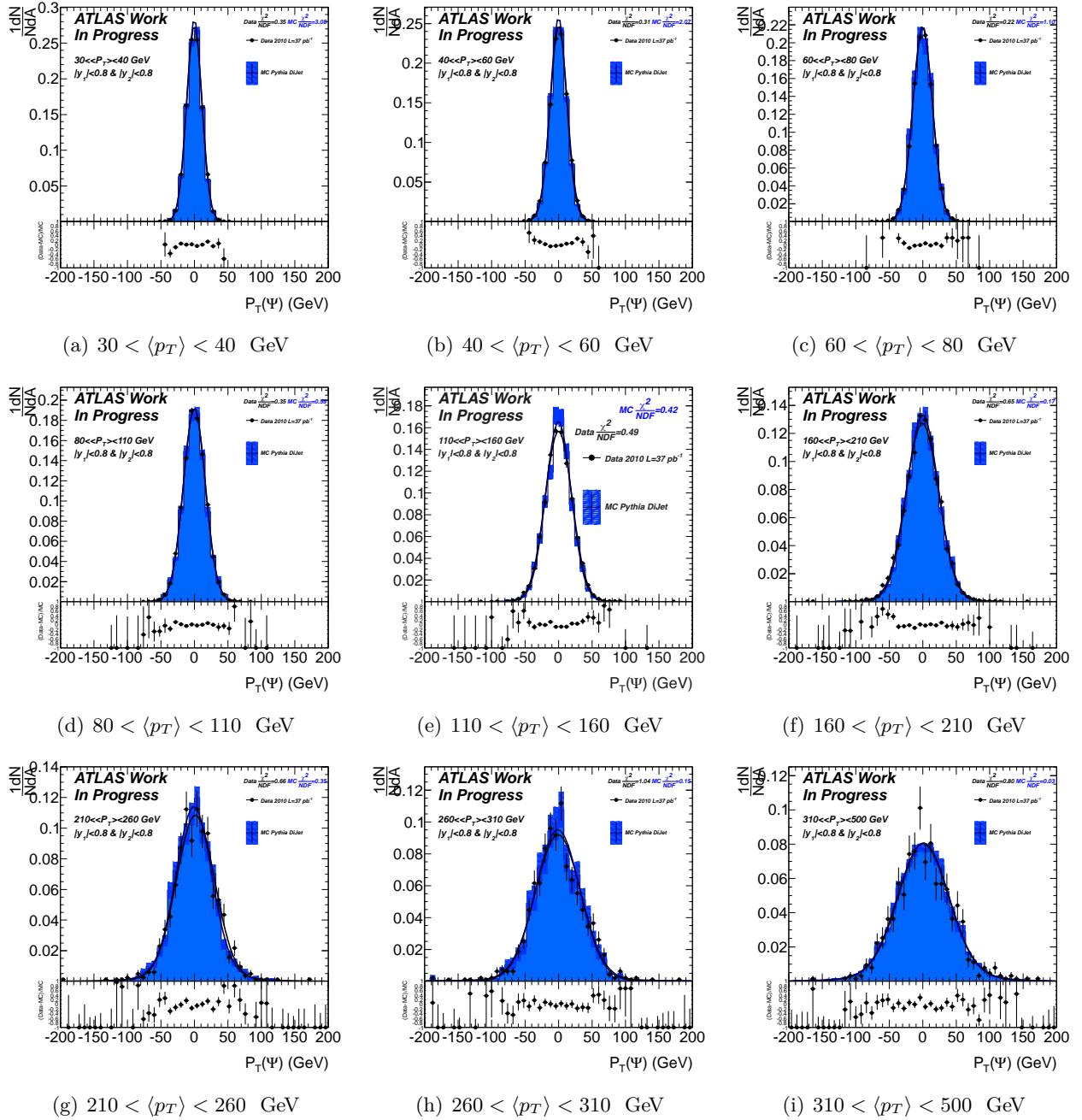
Figure A.12: p_T(\psi) distributions for two jets in |y| < 0.8 . Bisector Technique.
