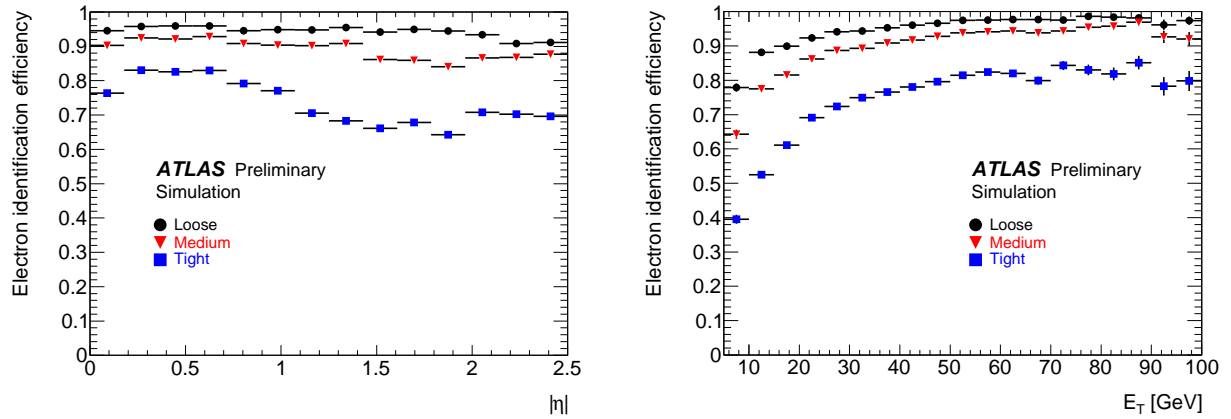
Figure 5.2: Identification of the electrons obtained on Z \rightarrow ee Monte Carlo samples, for the three default set of cuts, Loose, Medium and Tight. As a function of |\eta| (left) and E_T (right) [129].
