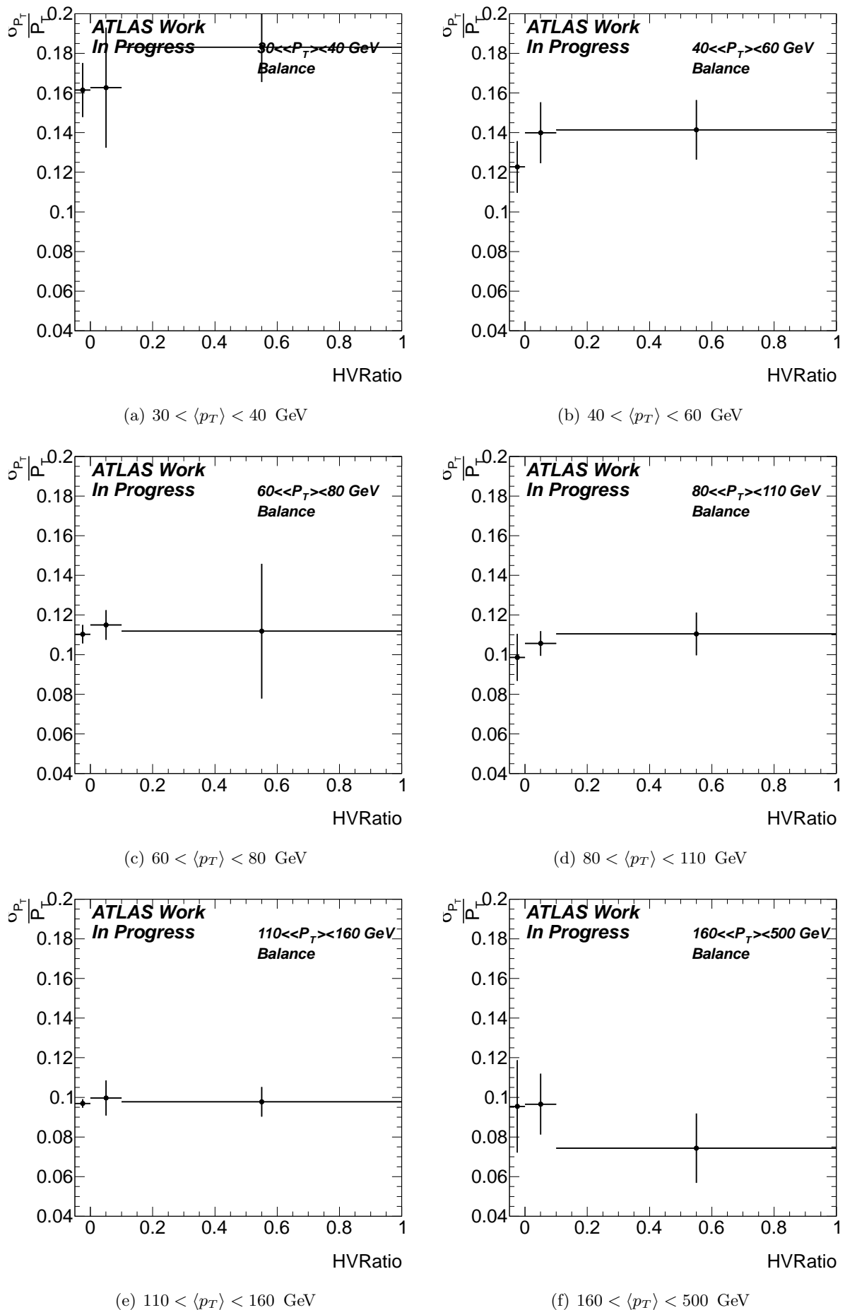
Figure 4.31: Jet fractional transverse momentum resolution measured vs the variable HV Ratio, for different \langle p_T \rangle bins. Results obtained using the balance method.
