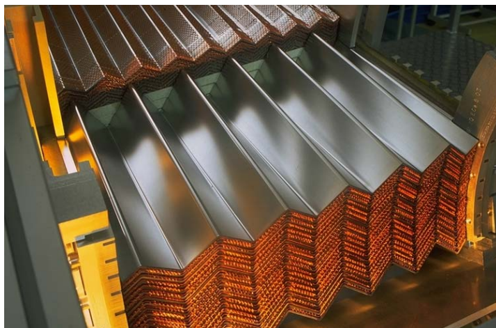
Figure 3.2: Photograph of barrel accordion-shaped electrodes and absorbers [83].
