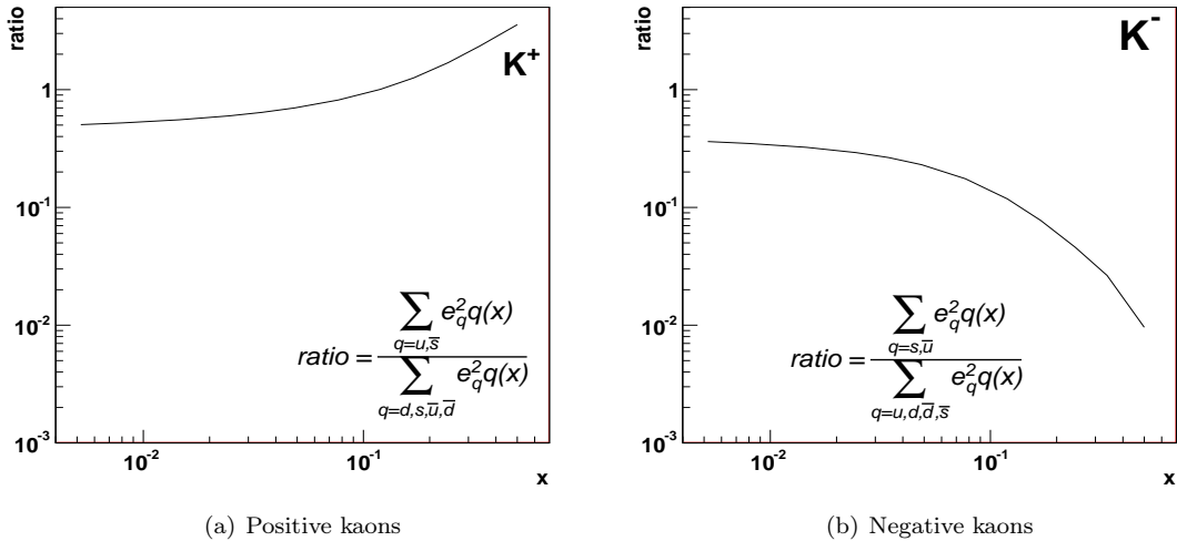
Figure 8.5: Ratio of the weighted sum of PDFs for favored to unfavored quark flavors for K^+ (left) and K^- (right) using the LO MRST 2004 parametrization.
