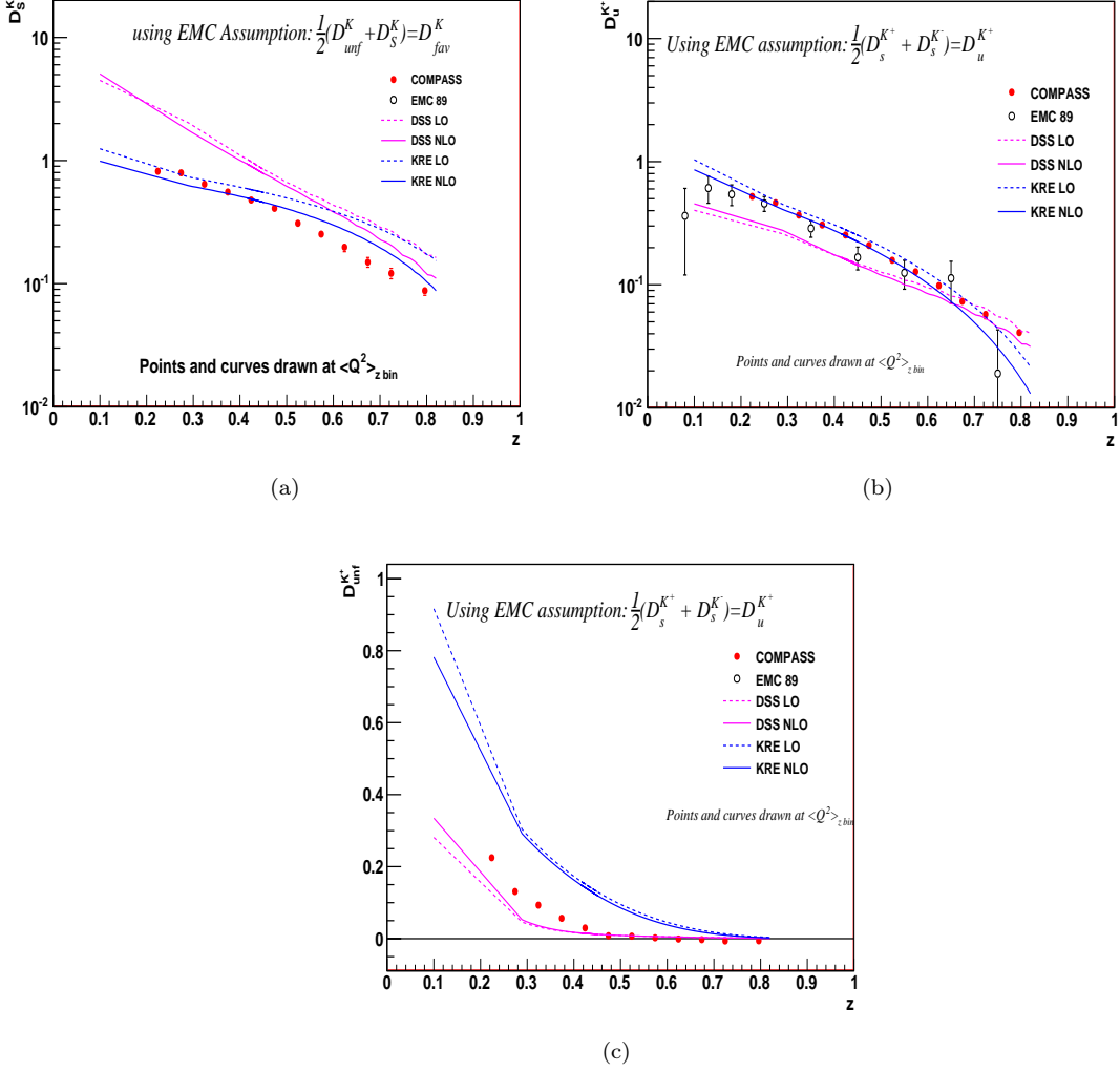
Figure A.2: D_{str}^K , D_{fav}^K and D_{unf}^K obtained using COMPASS kaon multiplicities and EMC assumption for FFs.
