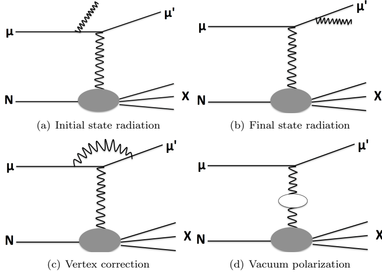
Figure 6: Higher order QED contributions to the DIS process.
