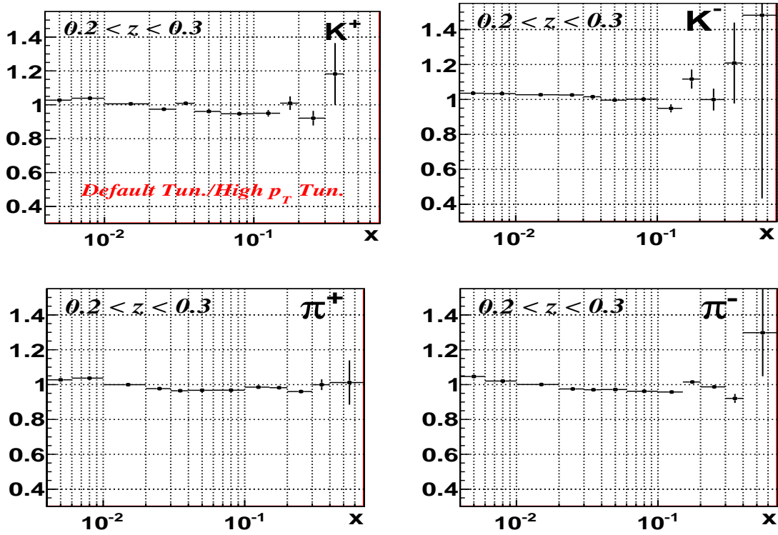
Figure 8.22: Ratio \epsilon_{high p_T} / \epsilon_{default} for pions and kaons as a function of x .
