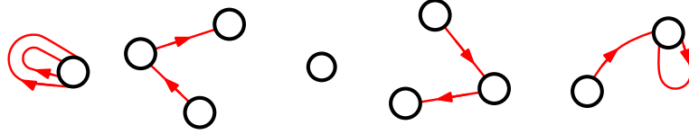
Figure 3.6: The five test graphs in the variable y induced by the test graph of Figure 3.5.
