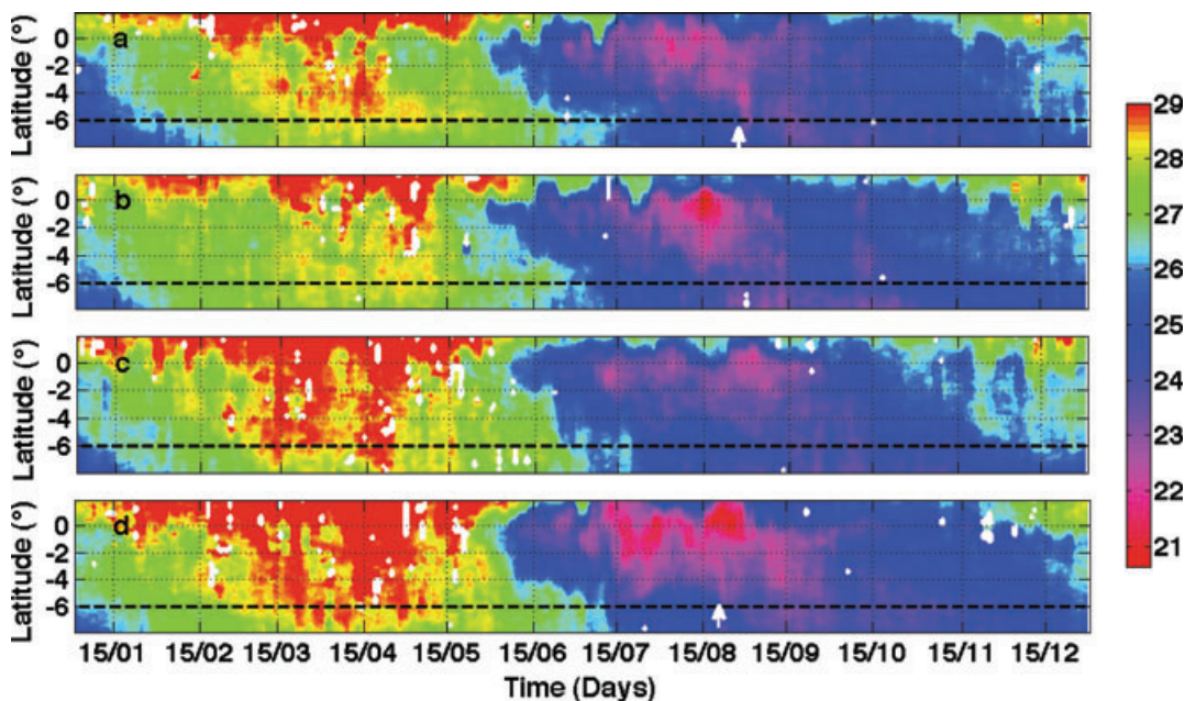
Fig. 2. Hovmöller latitude-time diagrams of TMI SST ( ^\circ\text{C} ) along 10^\circ\text{W} (a) in 2006 (b) in 2007 (c) 2008 (d) 2009. The dashed line corresponds to the latitude of 6^\circ\text{S} . The arrow in (a) indicates the 27 August 2006 and in (d) 25 August 2009. Missing values are indicated in white.
