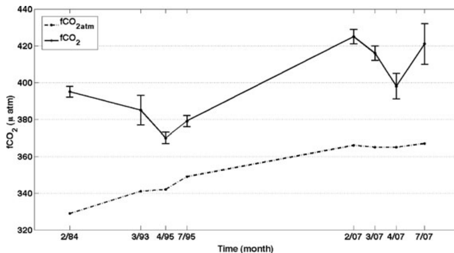
Fig. 6. Mean seawater f\text{CO}_2 corrected to an SST of 27^\circ\text{C} using the relationship of Takahashi et al. (1993) as a function of time (month/year). The data come the FOCAL 6 cruise in 1984 (Andrié et al., 1986), the Cither 1 cruise in 1993 (Oudot et al., 1995), the St Helena cruises in 1995 (Lefèvre et al., 1998) and the 2007 data at 6^\circ\text{S} , 10^\circ\text{W} . The dashed line corresponds to the mean atmospheric f\text{CO}_2 ( f\text{CO}_{2\text{atm}} ) measured during the different cruises.
