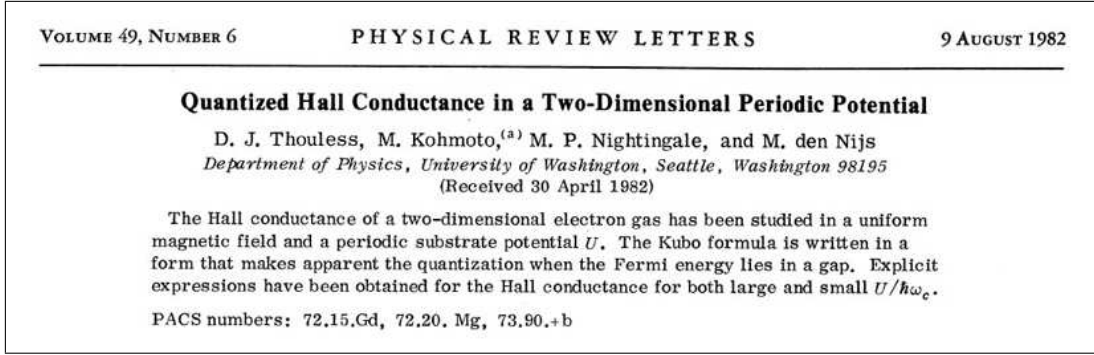
Figure 1.4: Header of the seminal paper of Thouless et al. that contains the first topological explanation for the QHE.
