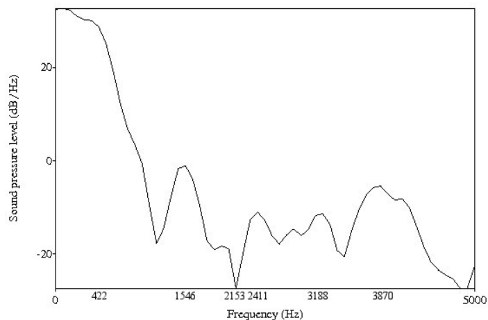
Figure 3: Spectral slice of clear /l/ in the sequence /a'la/ in the speech of a male speaker of Western Lengadocian Occitan. Spectral peaks are visible at 422 Hz, 1546 Hz, 2411 Hz, 3188 Hz, and 3870 Hz. A zero appears at 2153 Hz, just below F 3 .
