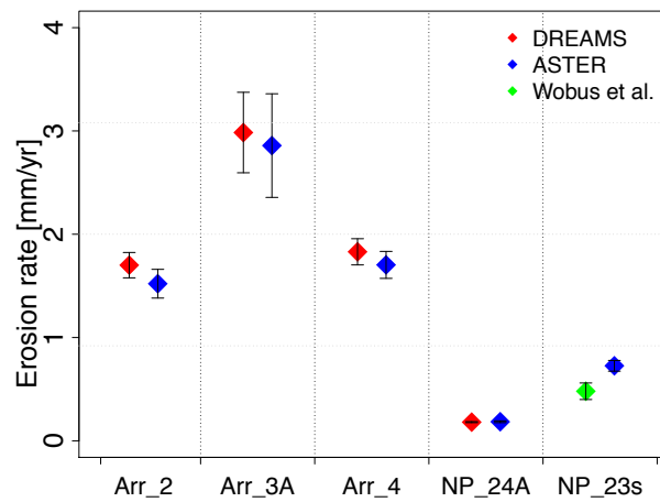
Figure 2: Comparison of cosmogenic nuclide erosion rates measured at different AMS (Accelerated Mass Spectroscopy) facilities. Compared are identical samples measured ones at the DREAMS (DREsden AMS) facility, Dresden/Rosendorf, Germany, and ones at the ASTER (Accelérateur pour les Sciences de la Terre, Environnement, Risques) facility, Aix-en-Provence, France. A fourth sample was compared to the measurement of Wobus et al. [2005]. The two later ones are not the same samples but were sampled at the same location with several years time difference. Our sample NP-23s was collected in November 2009. The sample of Wobus et al. [2005] was collected in 2001 (sample ID 01WBS7).
