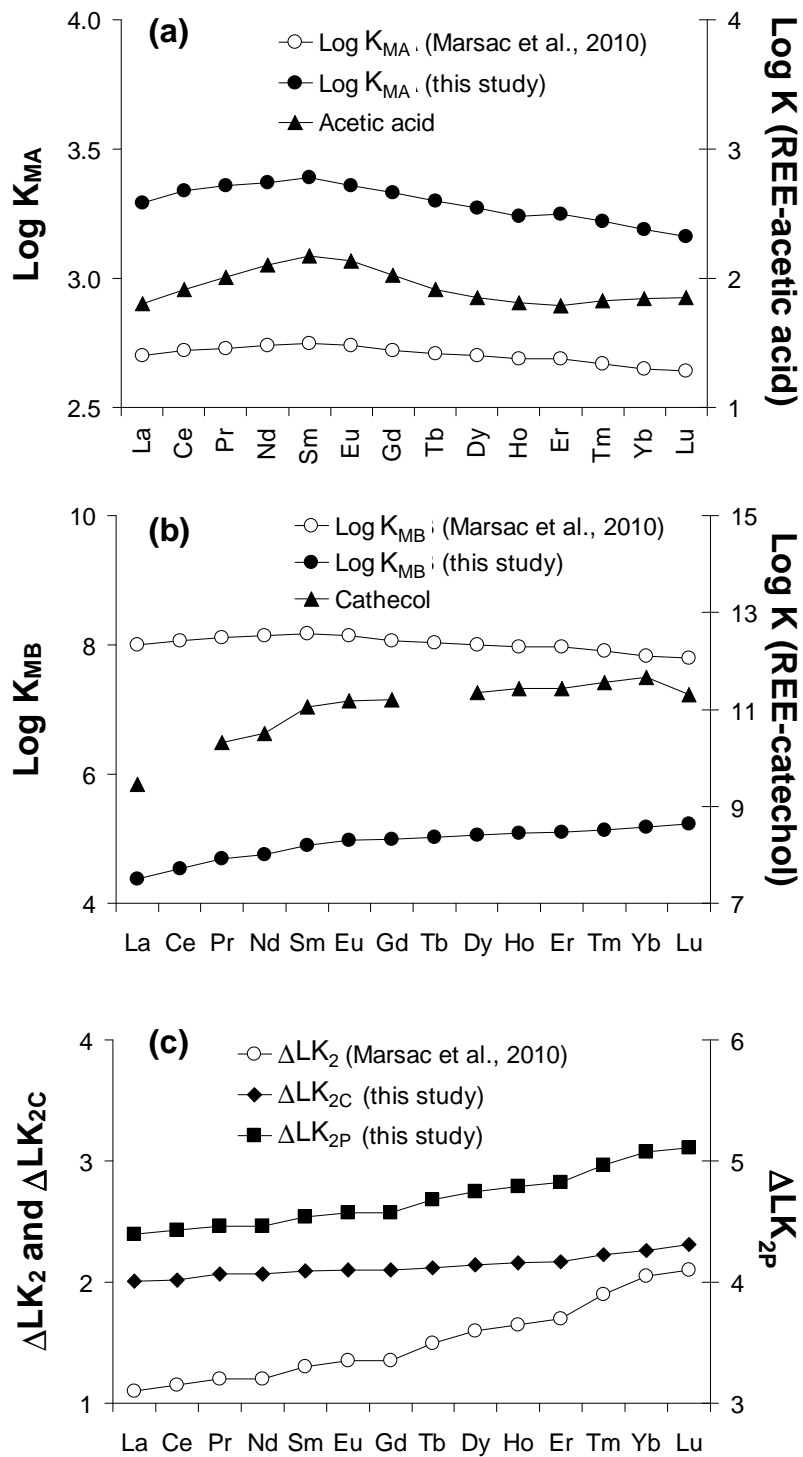
Figure III.1. Comparison of the REE patterns for the HA binding parameters obtained by Marsac et al. (2010) with WHAM 6/Model VI and the patterns obtained with PHREEQC/Model VI: (a) \log K_{MA} compared with \log K (REE-acetic acid), (b) \log K_{MB} compared with \log K (REE-catechol) and (c) \Delta LK_{2C} and \Delta LK_{2P} (this study) compared with \Delta LK_2 (Marsac et al., 2010; \Delta LK_2 = \Delta LK_{2C} = \Delta LK_{2P} ).
