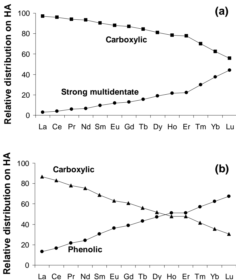
Figure V.1. Relative distribution of REE between the three major HA sites binding REE, at high REE/HA concentration ratio ( \Sigma[\text{REE}] = 10 \mu\text{M} , [\text{DOC}] = 6.7 \text{ mg L}^{-1} ). The dominant sites are (a) carboxylic and strong multidentate sites at pH=3 and (b) carboxylic and phenolic sites at pH=6.
