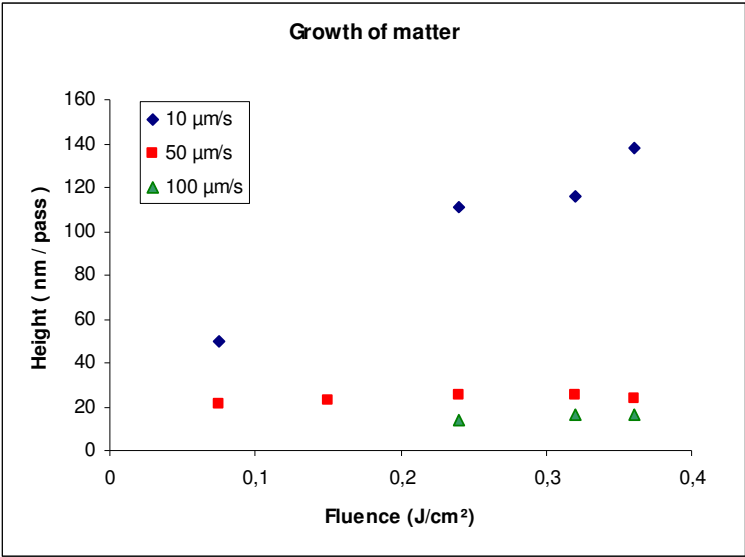
Figure 69 Growth of the matter depending on the fluence for 10, 50 and 100 μm/s, the corresponding number of pulses are 16 \cdot 10^6 , 32 \cdot 10^5 and 16 \cdot 10^5 pulses respectively.
