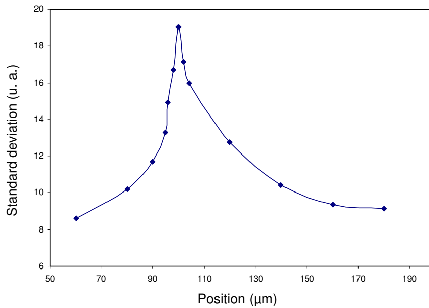
Figure 36 Standard deviation depending on the position of the objective. We see clearly a maximum for the position of 100 \mu\text{m} which corresponds to the focus position.
