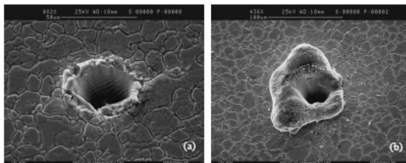
Figure 56 SEM pictures of holes obtained with percussion drilling technique with energy of 30 \mu J at (a) 100 kHz and (b) at 400 kHz[120].
