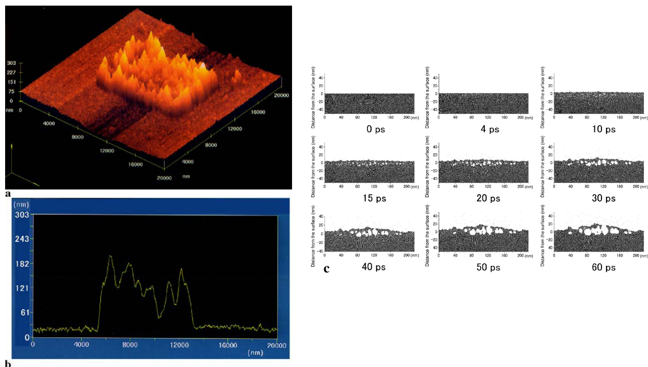
Figure 55 AFM pictures of microcolumns obtained after 500 pulses on 80 nm thick chromium film. (a) 3D profile of microcolumns, (b) line profile. (c) Snap shots from MD simulation of the surface instability. We can clearly see the formation of the porosity [119].
