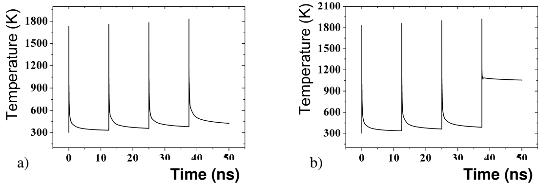
Figure 17 Comparison of the evolution of the temperature at the surface of the material after irradiation of 4 pulses: (a) at 0.25 \text{ J/cm}^2 and (b) at 0.29 \text{ J/cm}^2 .
