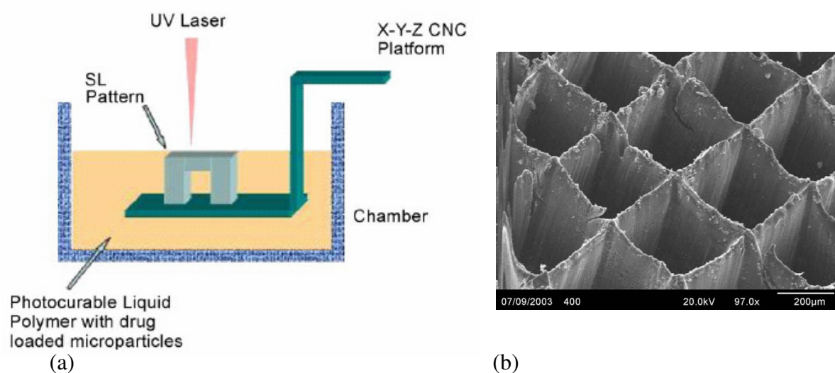
Figure 4 Scheme of a laser stereolithography setup (a). Cellular-type structure made with stereolithography (b) [25][26].
