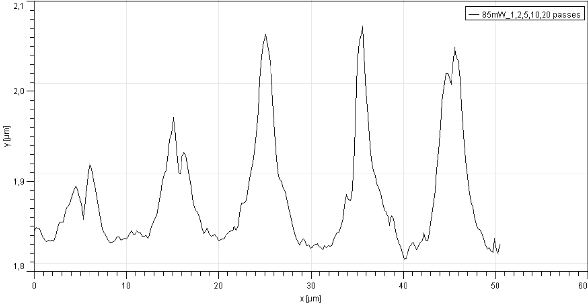
Figure 82 Results on copper at 10µm/s for several fluences 0.36, 0.32, 0.24, 0.15 and 0.075 J/cm 2 , and different number of passes, respectively from the left to right 1, 2, 5, 10, 20 passes.
