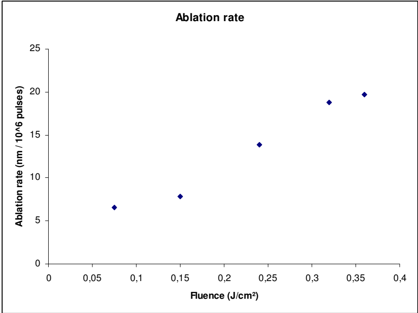
Figure 68 Evolution of the ablation rate expressed in nm/10 6 pulses depending on the fluence.
