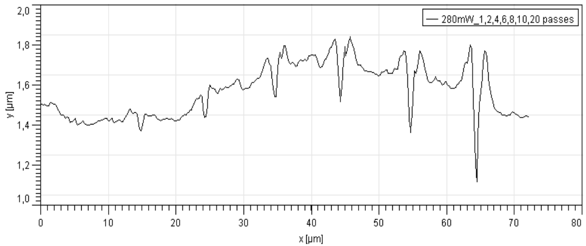
Figure 84 Results on copper at 100µm/s for several fluences 0.36, 0.32 and 0.24 J/cm 2 , and different number of passes, respectively from the left to right 1, 2, 4, 6, 8, 10, 20 passes.
