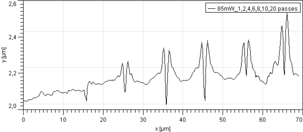
Figure 83 Results on copper at 50µm/s for several fluences 0.36, 0.32, 0.24, 0.15 and 0.075 J/cm 2 , and different number of passes, respectively from the left to right 1, 2, 4, 6, 8, 10, 20 passes.
