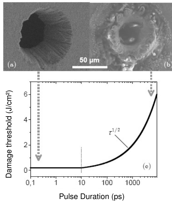
Figure 6 Comparison of impacts on 100 μm thick copper samples between ultrafast pulses (a) of 180 fs, and longer pulses (b) of 8 ns. Both have been done with a fluence of 8 J/cm 2 . The influence of pulse duration seems to follow a law in \tau^{1/2} after ~10 ps (c) [32][33][34].
