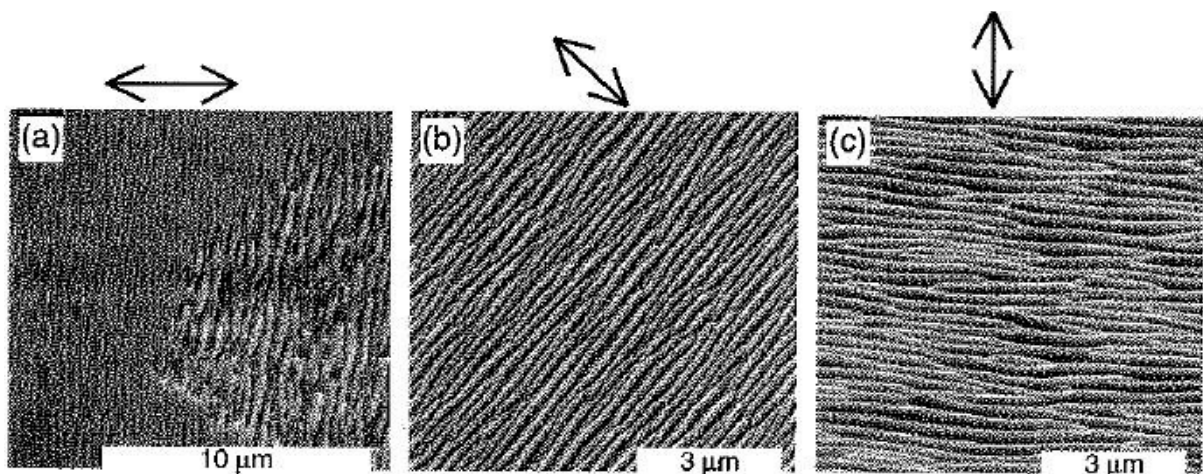
Figure 14 Arrows indicate the polarization's orientation of the beam respectively of 0^\circ (a), 40^\circ (b) and 90^\circ (c). The dependence of the orientation of ripples on the polarization is obvious. Notice that in the picture (a) there are both coarse and fine ripples oriented in the same direction. Fine ripples are on the edge of the crater, coarse ripples are in the center [76].
