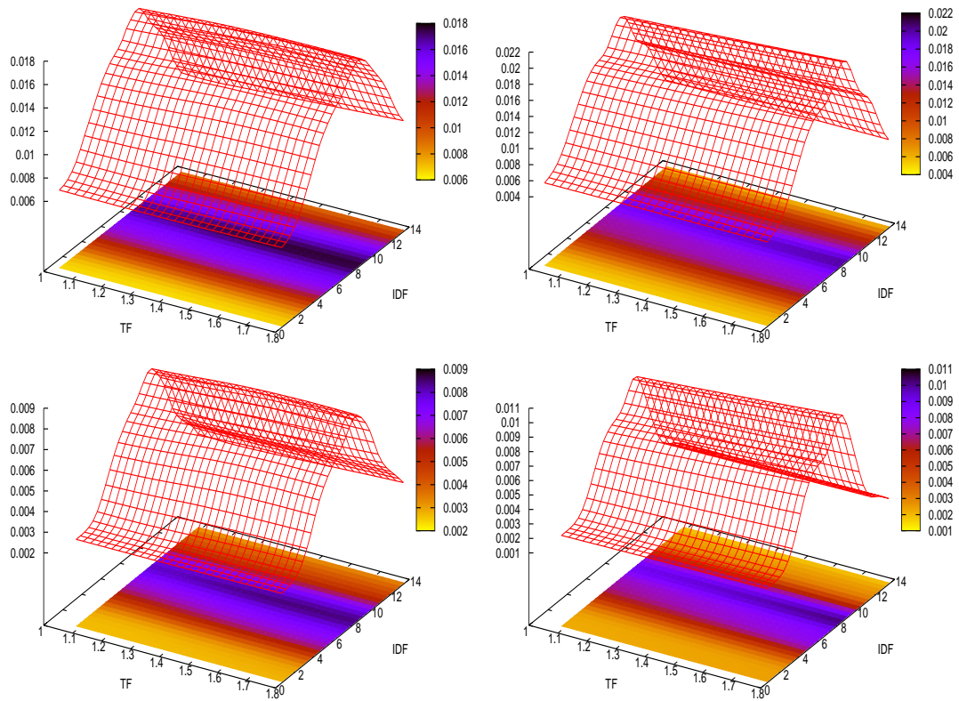
Figure 6.5: True Oracle (TF, IDF) vs \Delta MAP sur TREC-1&2 n = 10 tc = 50 . Exponential (left) and Gaussian (right) Kernel Grid 15 \times 15 . LG(top row) LM(bottom)
