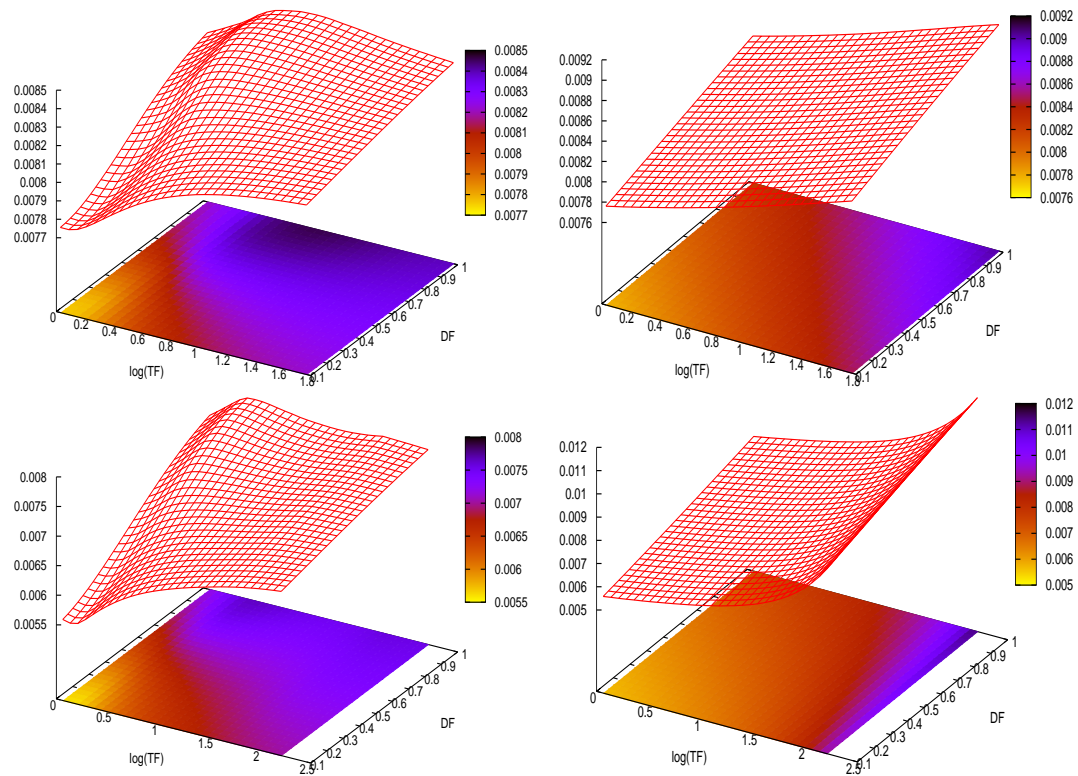
Figure 6.3: (\log(\text{TF}), \text{DF}) vs \Delta MAP on ROBUST; true relevant documents are used with n = 10 , t_c = 50 and exponential (left) and Gaussian (right) kernel grids ( 15 \times 15 ). Top row: log-logistic model; bottom row: language model
