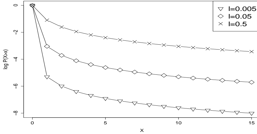
Figure 5.2: \log P(X > x) for \lambda \in \{0.5, 0.05, 0.005\}
