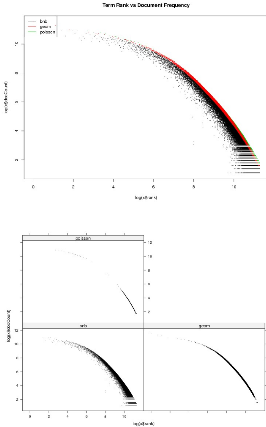
Figure 2.11: CLEF
