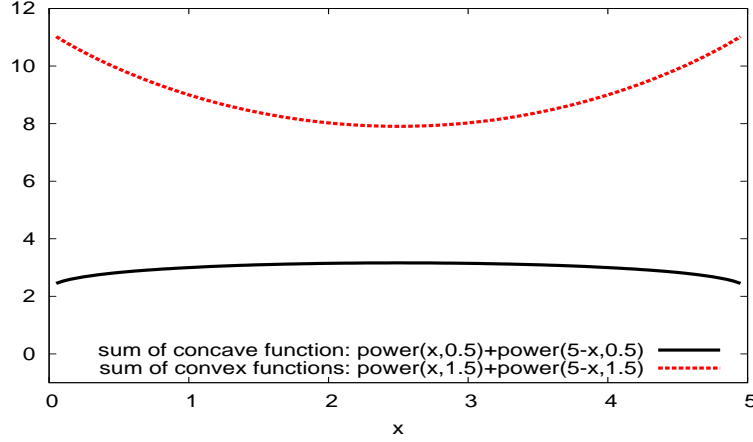
Figure 4.3: Illustration of the equipartition property of concave functions as opposed to convex functions
