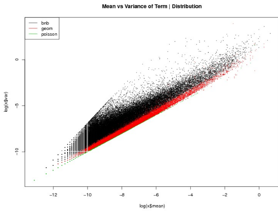
Figure 2.16: TREC-7 ROBUST
