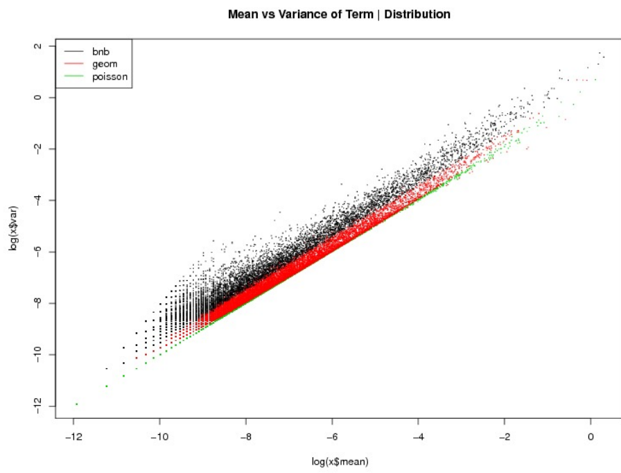
Figure 2.14: GIRT
