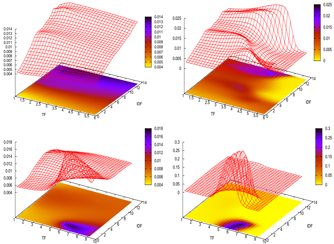
Figure 6.4: True Oracle (TF, IDF) vs \Delta MAP sur ROBUST n = 10 tc = 50 . Exponential (left) and Gaussian (right) Kernel Grid 15 \times 15 . LG(top row) LM(bottom)
