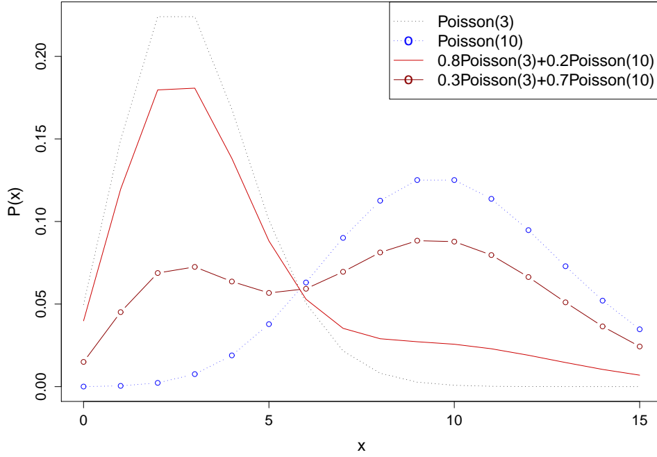
Figure 2.5: 2-Poisson Mixture Model
