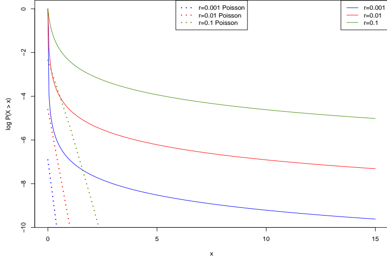
Figure 2.10: \log P(X > x) Poisson( r ) and Log-Logistic( r ) when r \in \{10^{-1}, 10^{-2}, 10^{-3}\}
