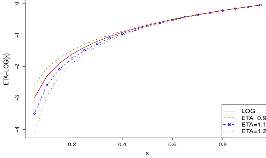
Figure 5.6: \log_\eta for \eta \in \{0.9, 1, 1.1, 1.2\}
