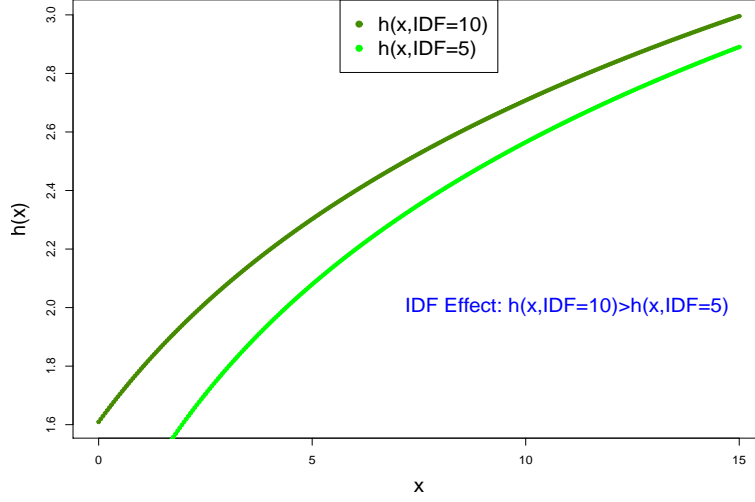
Figure 4.4: Illustration of IDF effect
