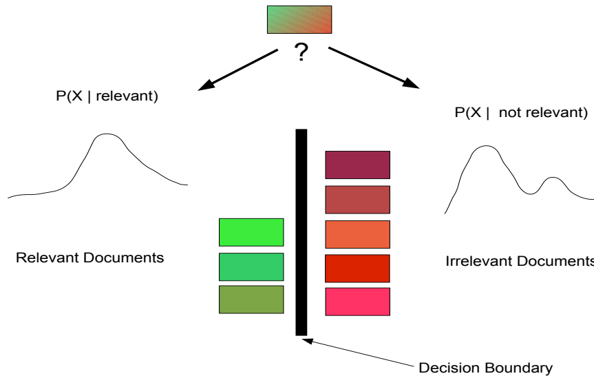
Figure 3.2: The Probability Ranking Principle. Two class of documents exists: relevant and not relevant. For each class, a probability distribution models documents. When a new document comes in, class probabilities are computed in order to decide which class this document belongs to.
