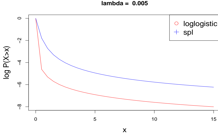
Figure 5.3: Smoothed Power Law distribution vs Log-Logistic distribution with parameter equal to 0.005
