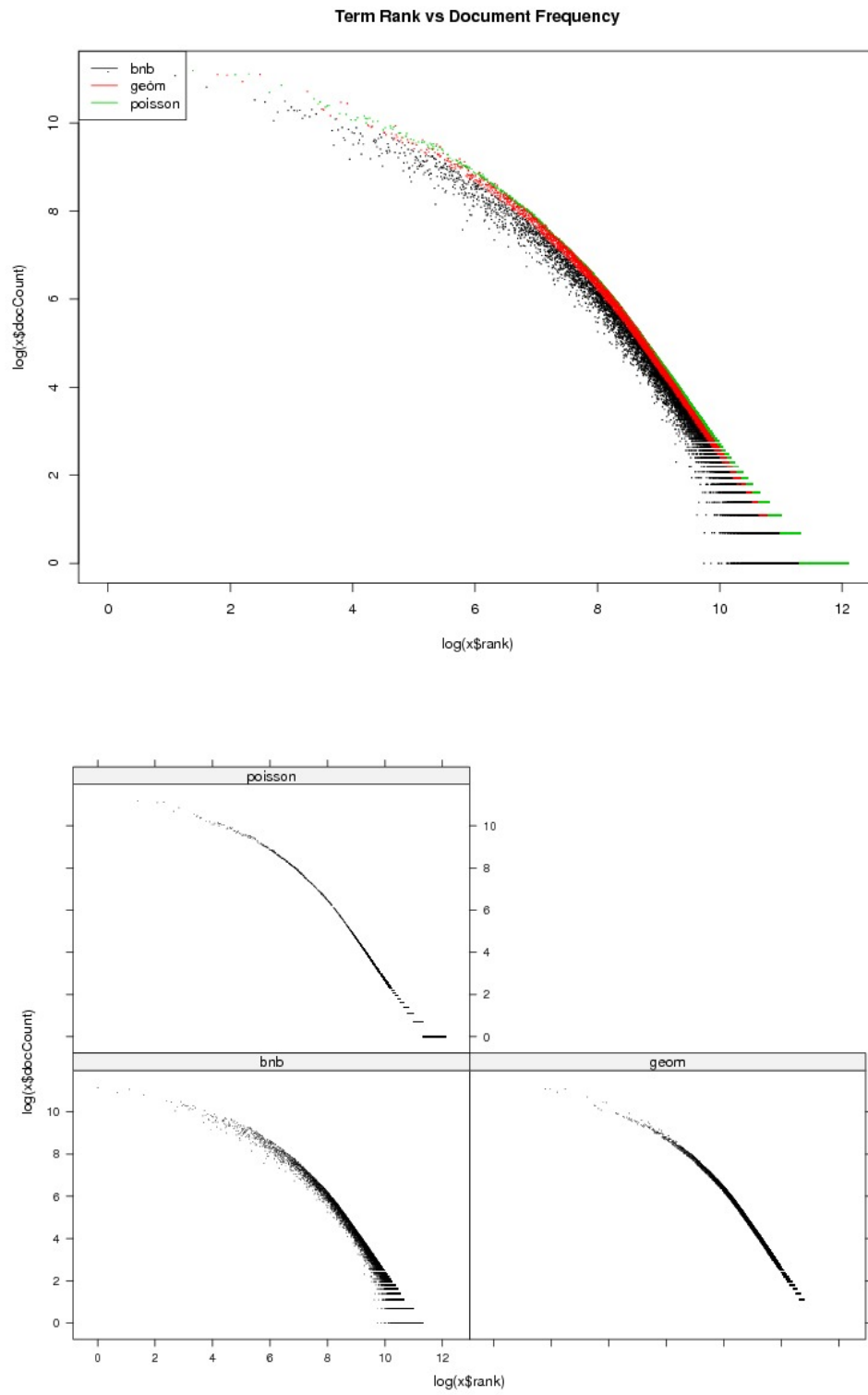
Figure 2.13: GIRT
