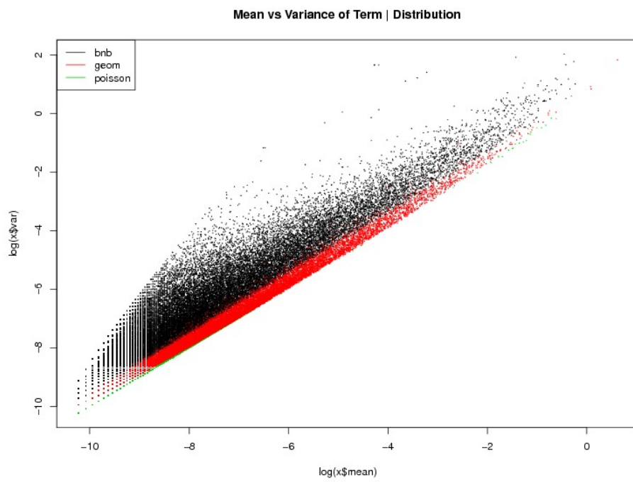
Figure 2.12: CLEF
