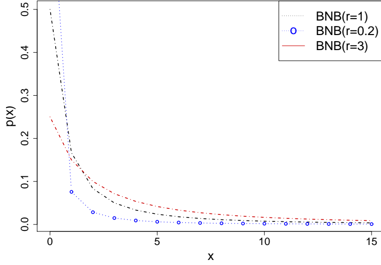
Figure 2.8: Beta Negative Binomial Distribution
