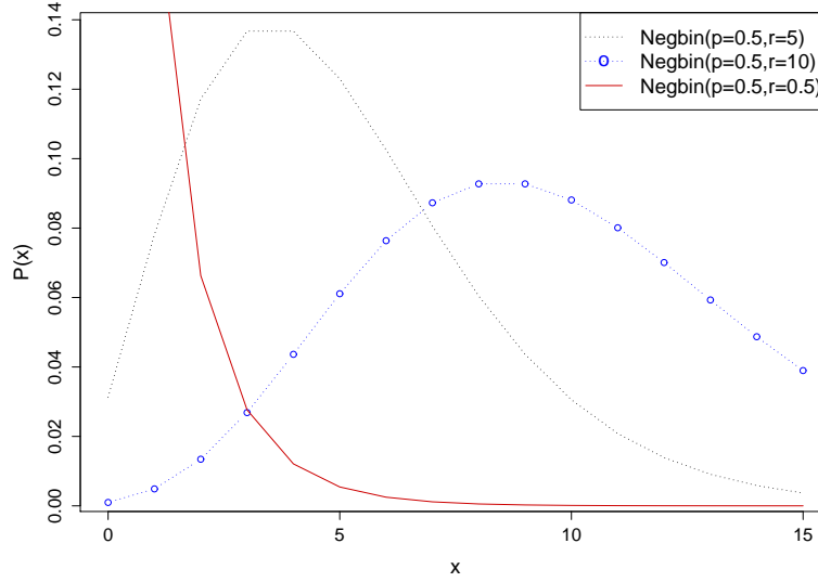
Figure 2.6: Negative Binomial Distribution
