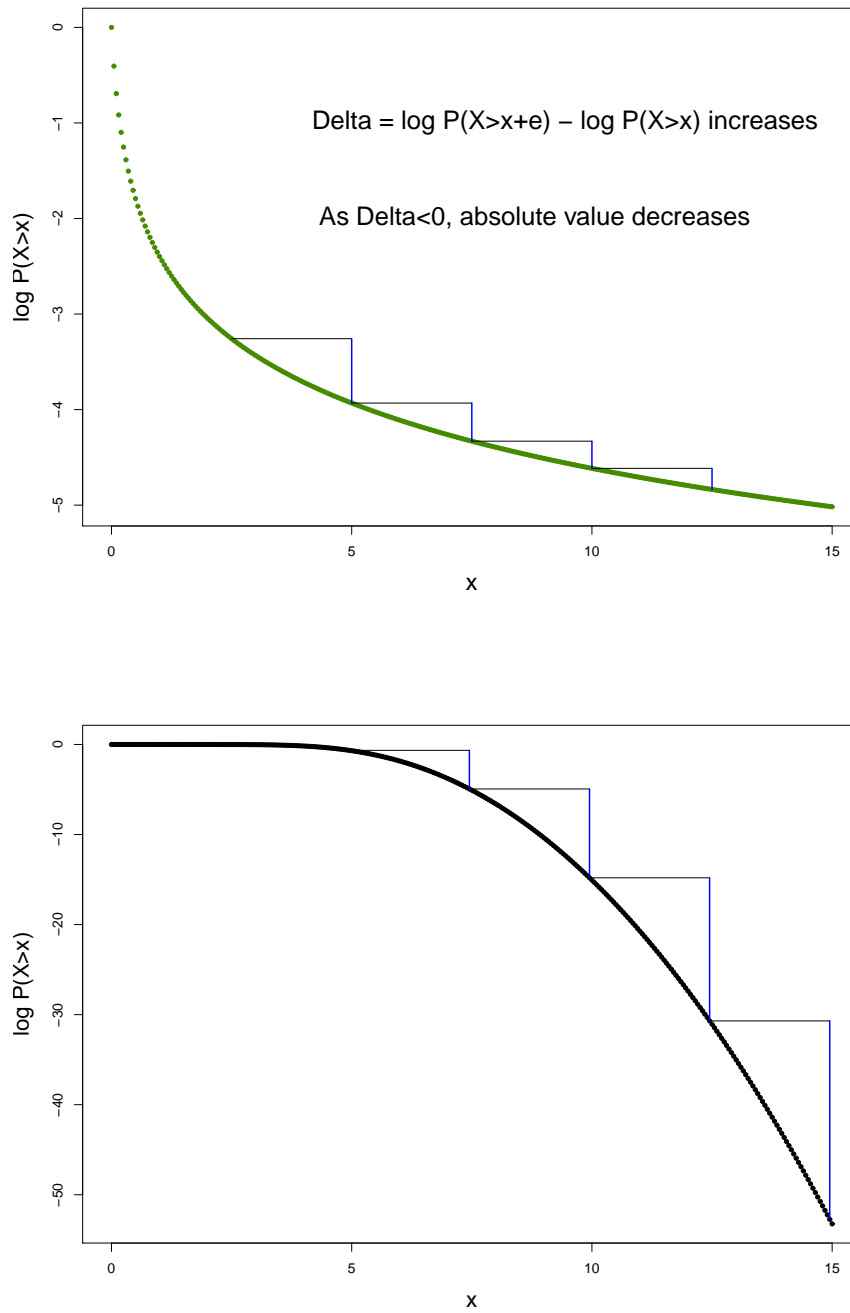
Figure 2.7: Geometrical Interpretation of burstiness: top figure shows a bursty distribution (log-logistic) and bottom figure shows that the Gaussian(mean=5, std=1) is not bursty
