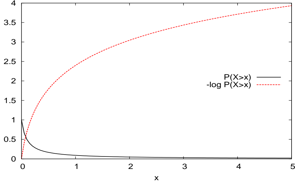
Figure 5.1: Illustration of the Shannon information measure on the Survival function. For small frequencies, then this information is low. On the contrary, for large frequencies, ie a low probability gives a lot of information
