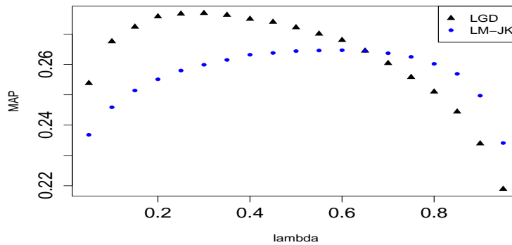
Figure 5.5: MAP against lambda. ROB-t are plot on the top and ROB-d at the bottom
