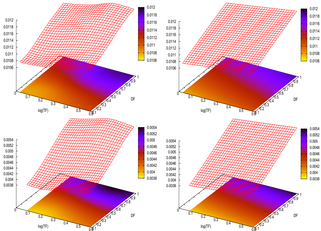
Figure 6.2: (\log(\text{TF}), \text{DF}) vs \Delta \text{MAP} on TREC-12; true relevant documents are used with n = 10 , t_c = 50 and exponential (left) and Gaussian (right) kernel grids ( 15 \times 15 ). Top row: log-logistic model; bottom row: language model
