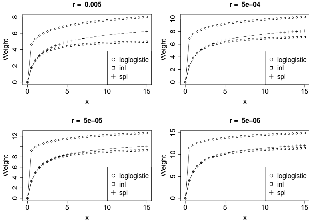
Figure 5.4: Plot of Retrieval Functions with different values of corpus frequencies r_w = \exp(-IDF(w))
