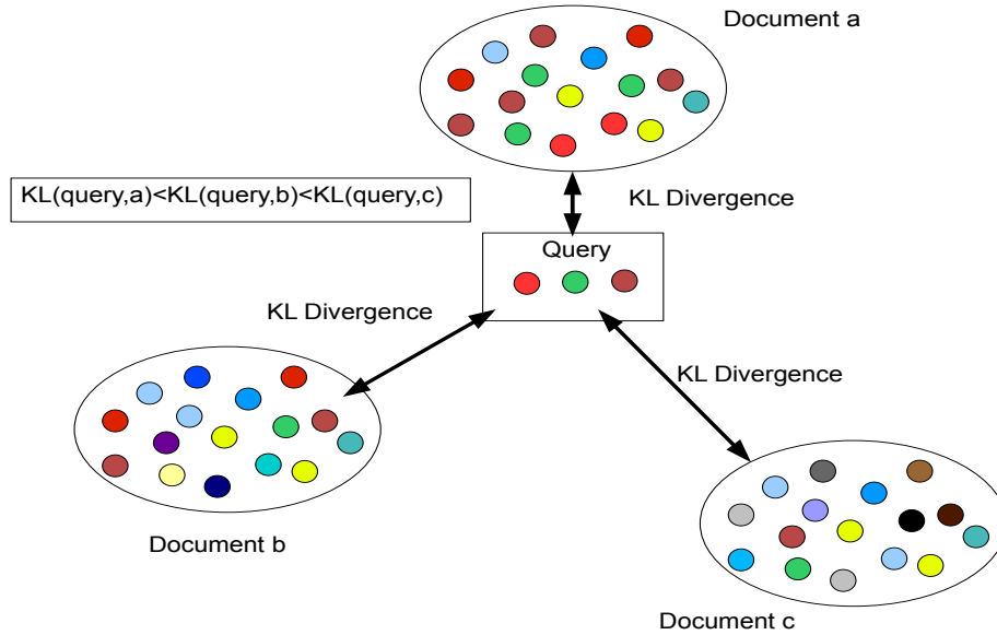
Figure 3.3: The language modeling approach to Information Retrieval. Documents are represented by bag of words, i.e. multinomial distributions. Then, KL-Divergence serves as a distance between queries and documents. In the figure, document a has a lower KL divergence compared to other documents because it contains more query terms.
