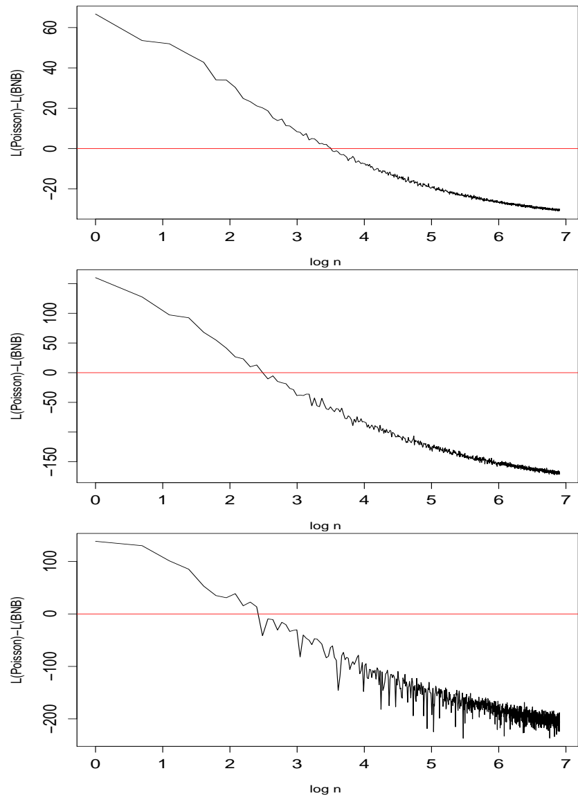
Figure 2.18: Number of Documents n against the difference of Likelihood between BNB and Poisson for the GIRT, CLEF03 and ROBUST collection
