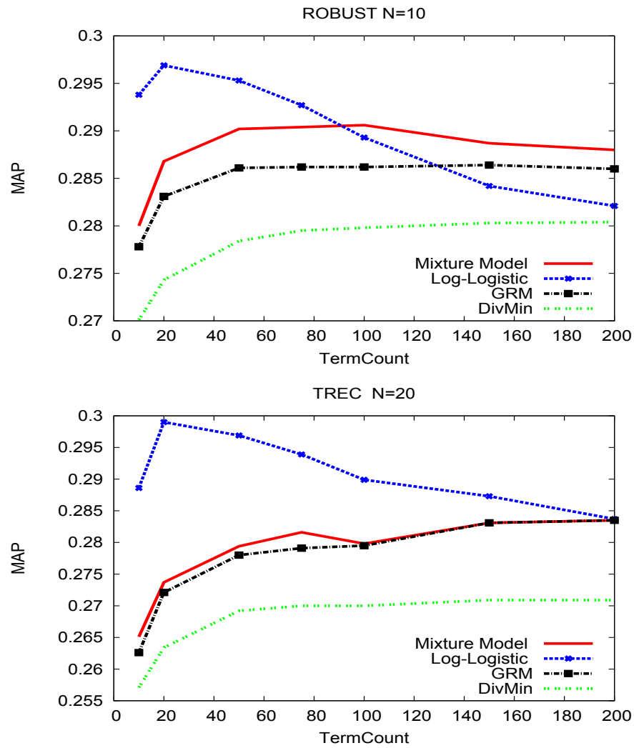
Figure 6.1: MAP on all queries with tc \in \{10, 20, 50, 75, 100, 150, 200\} with best parameters, ROBUS n = 10 top, TREC-1&2 n = 20 bottom
