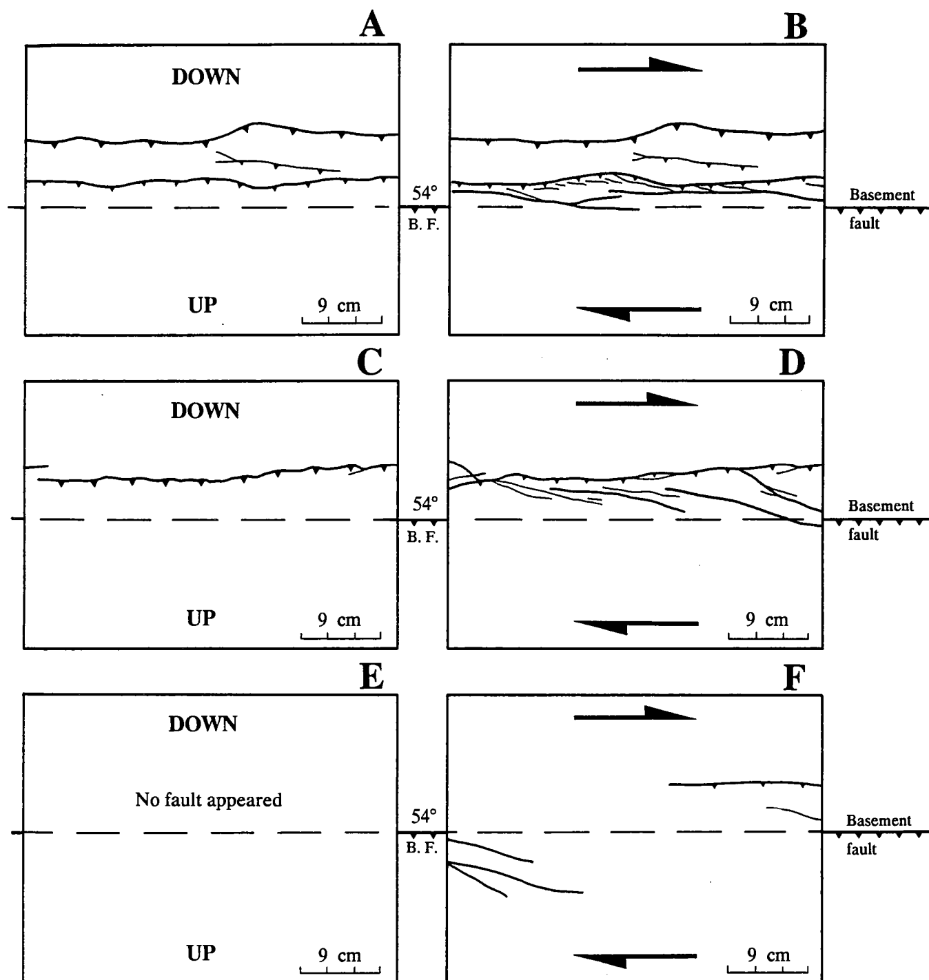
Fig. 5 - 13. Line drawing of faults formed above a reactivated 54^\circ reverse basement fault in pure strike-slip mode, after dip-slip stage (left) and final stage (right), for different rheologies: A,B, pure brittle model; C,D, 5 cm of sand overlying 1 cm of silicone; E,F, 4 cm of sand overlying 2 cm of silicone.
