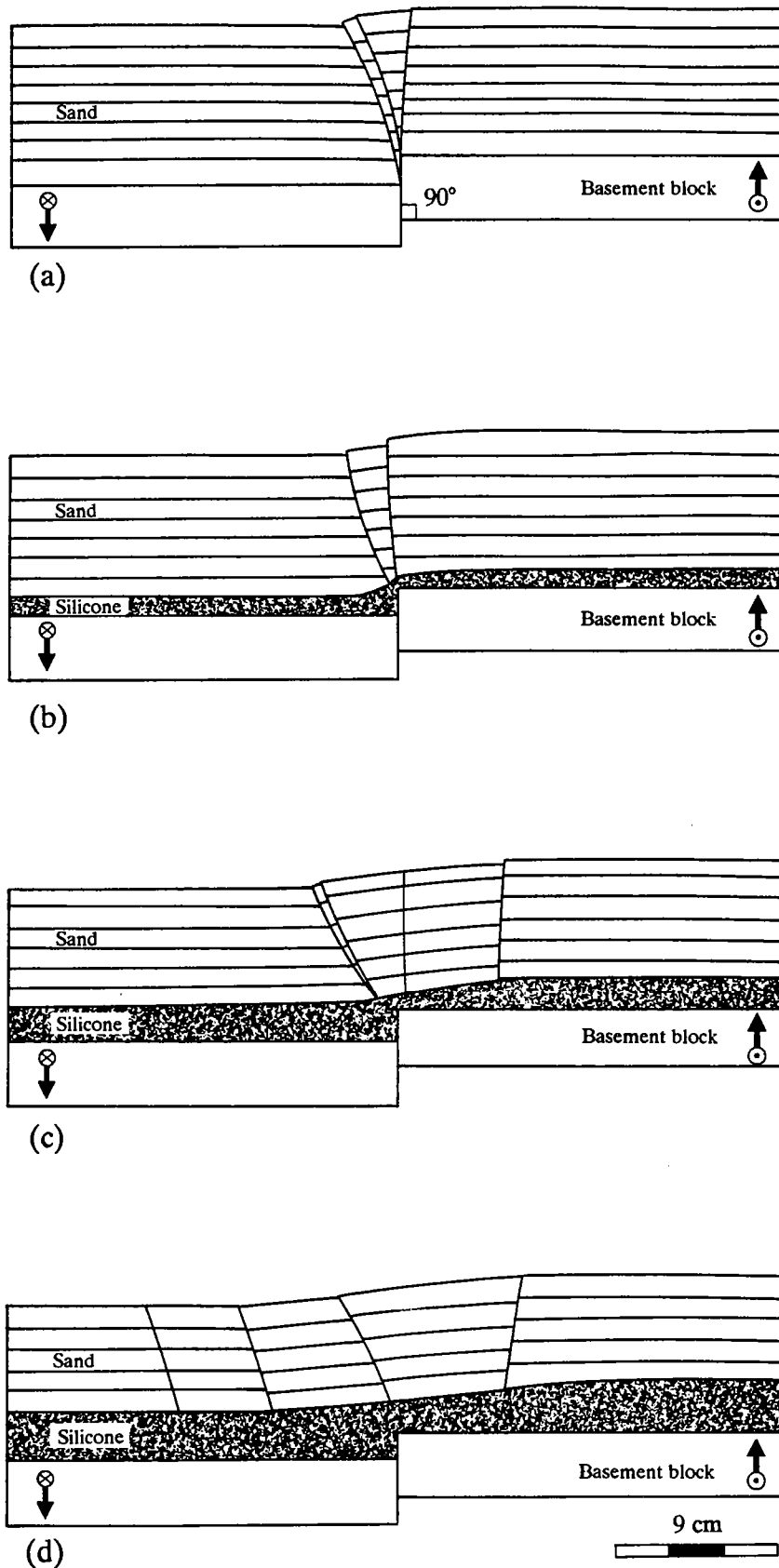
Fig. 4 - 20. Line drawings of cross sections through faulted zones formed above a 90° basement fault with the same dip-slip (5 cm), and the SS/DS ratio ( SS/DS = 3.5 ), with various rheologies. Sections have been located on the Figure 7.
