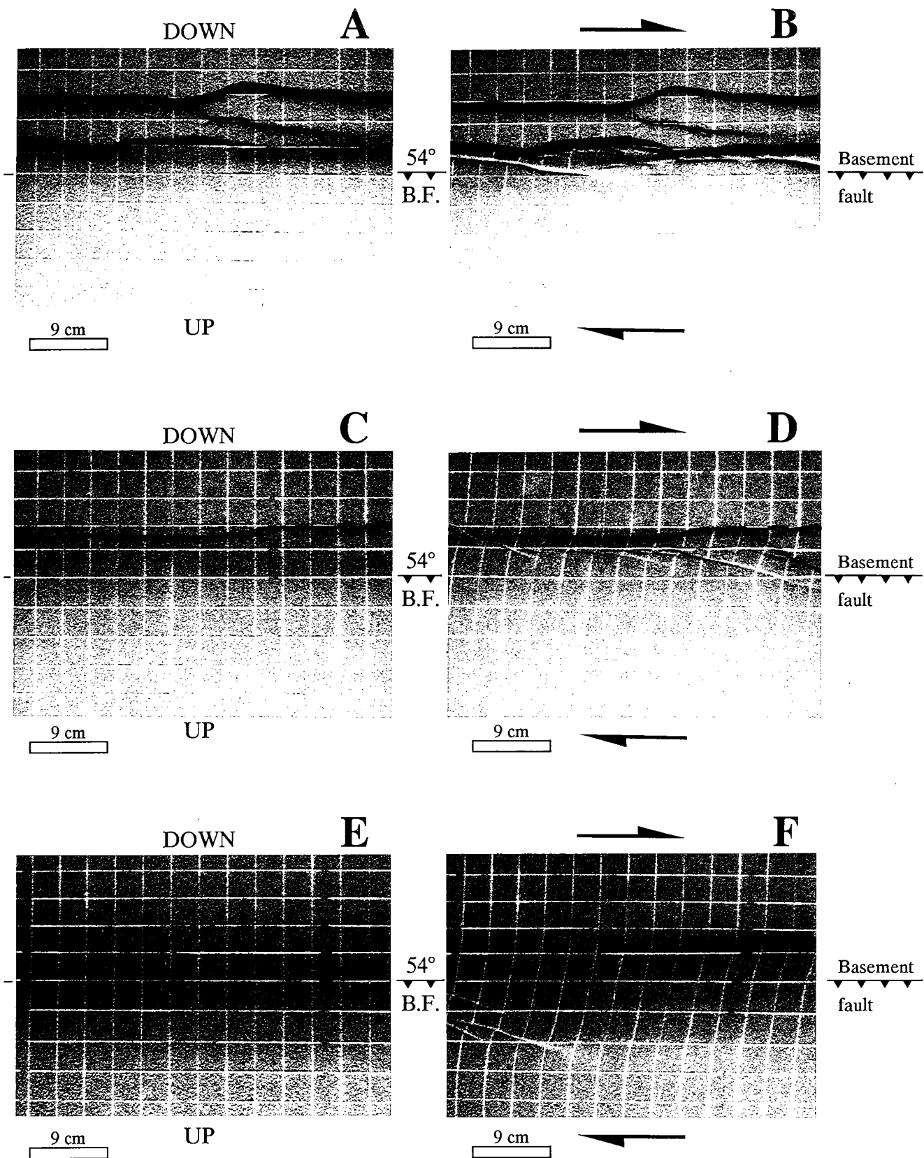
Fig. 5 - 12. Reactivation in pure strike-slip mode of a 54° reverse basement fault. Photographs of top views of experiments after dip-slip stage (left) and final stage (right), for different rheologies: A,B, pure brittle model; C,D, 5 cm of sand overlying 1 cm of silicone; E,F, 4 cm of sand overlying 2 cm of silicone.
