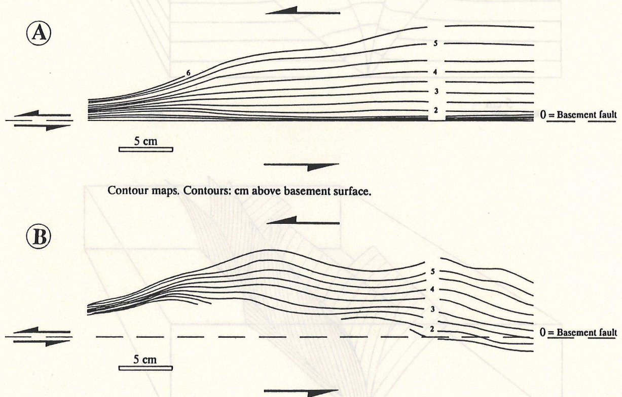
Fig. 6 - 6. Structural contour maps of fault surfaces, reconstructed from serial vertical sections (1 cm apart) through sand model (A) and sand-silicone model (B). Kinematic ratio was R = 1/3 . Contours are labelled for height (cm) above basal plates. For sand model (sand only), fault surface roots into baseplate fault and is convex upward. For sand-silicone model, fault surface is less regular.
