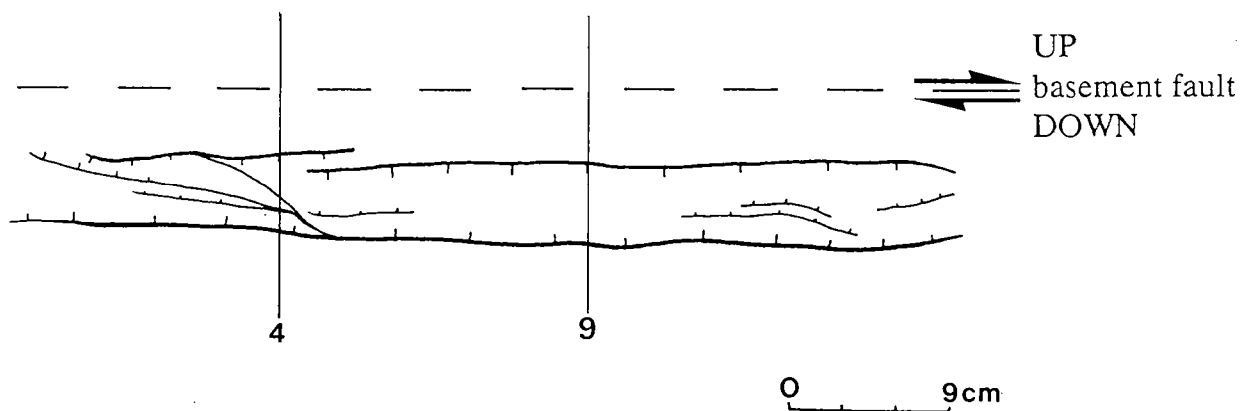
Fig. 5 - 7. Photographs and line drawings of faulted structures formed in an experiment of reactivation of normal faults in a cover sequence overlying a reactivated in reverse oblique-slip mode basement fault. A - intermediate stage. B - final stage.
