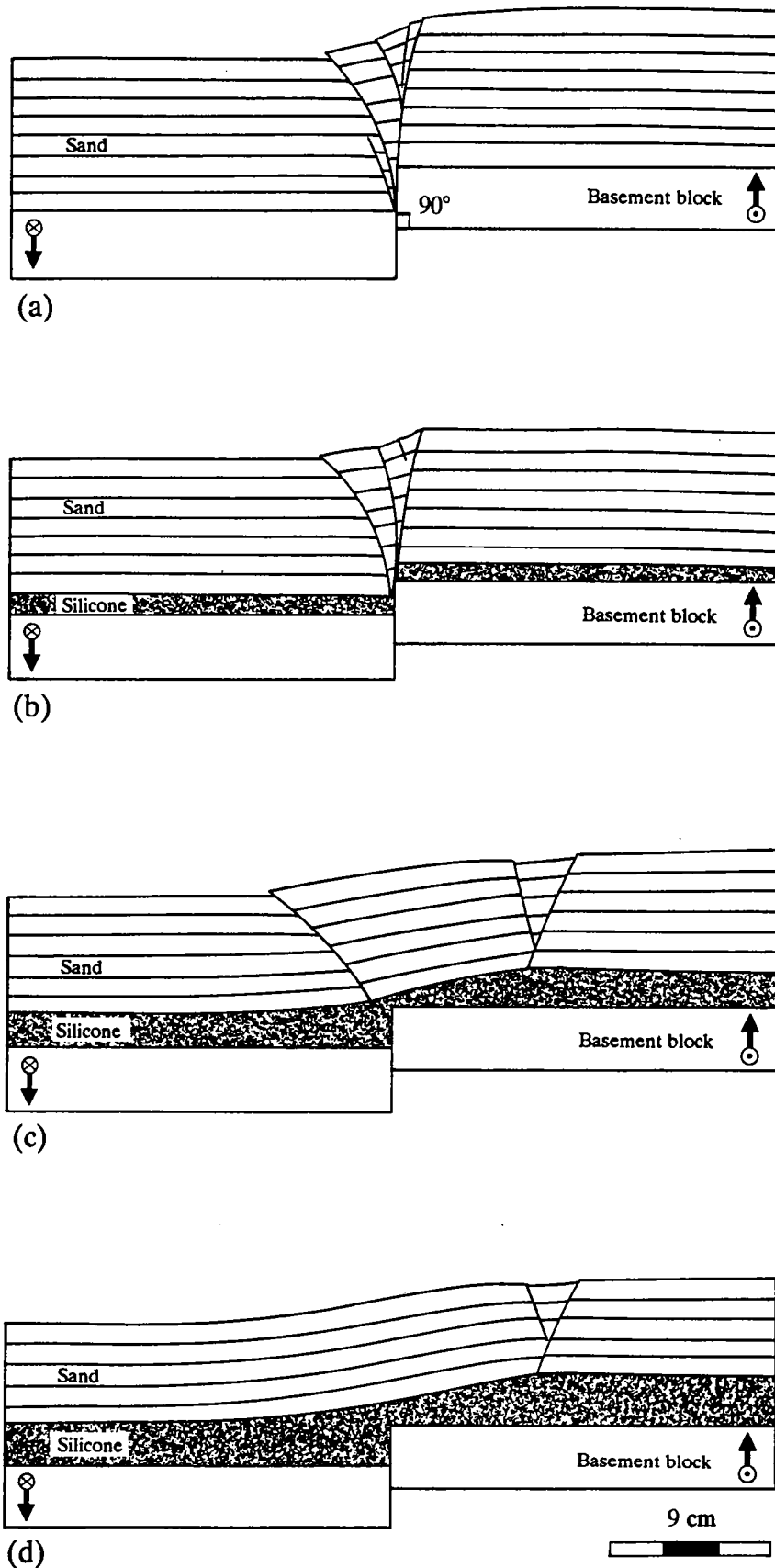
Fig. 4 - 18. Line drawings of cross sections through faulted zones formed above a 90° basement fault with the same dip-slip (3.7 cm), and the SS/DS ratio ( SS/DS = 1 ), with various rheologies. Sections have been located on the Figure 5.
