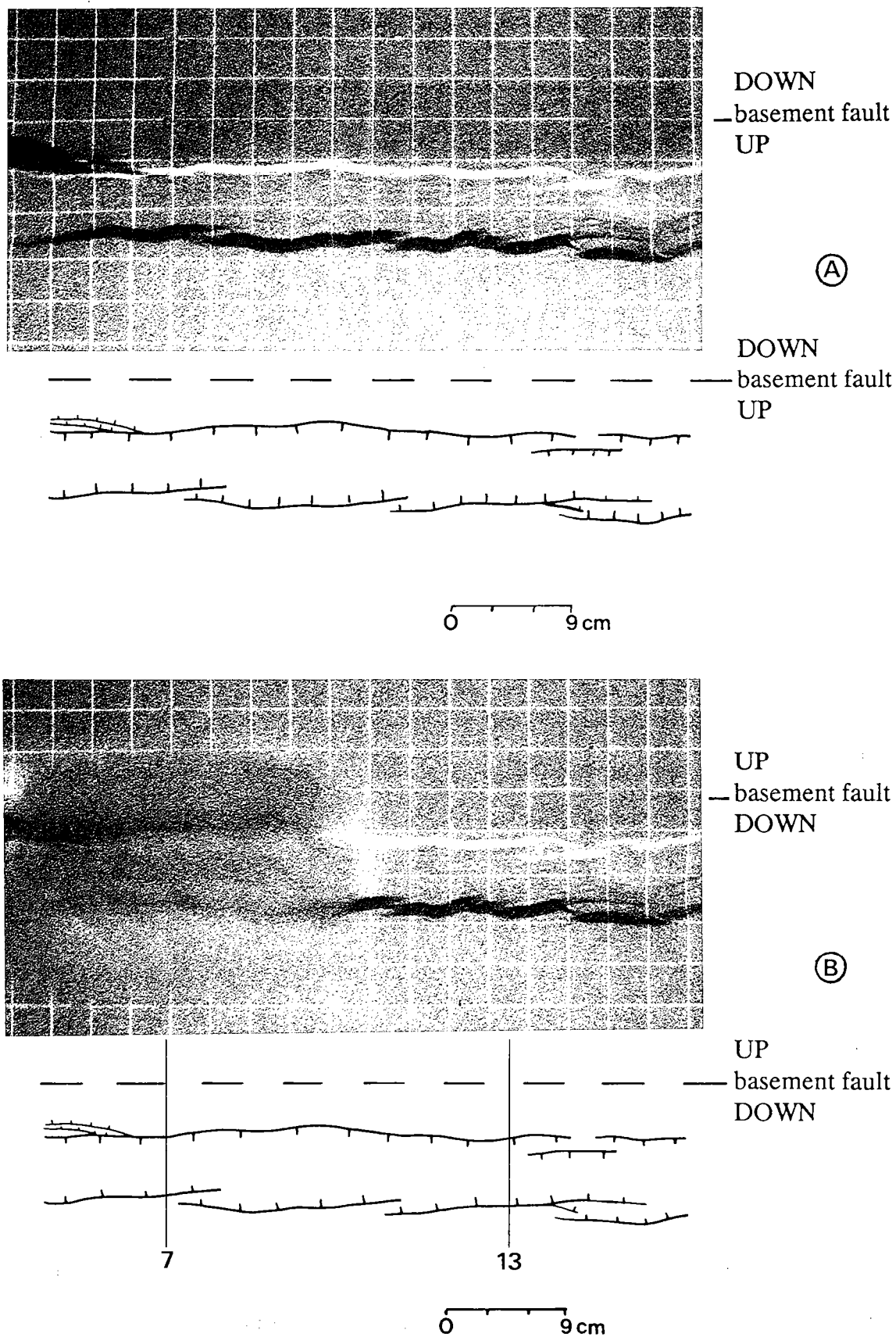
Fig. 5 - 5. Photographs and line drawings of faulted structures formed in an experiment of reactivation of normal faults in a cover sequence overlying a reactivated in pure dip-slip mode basement fault. A - intermediate stage. B - final stage.
