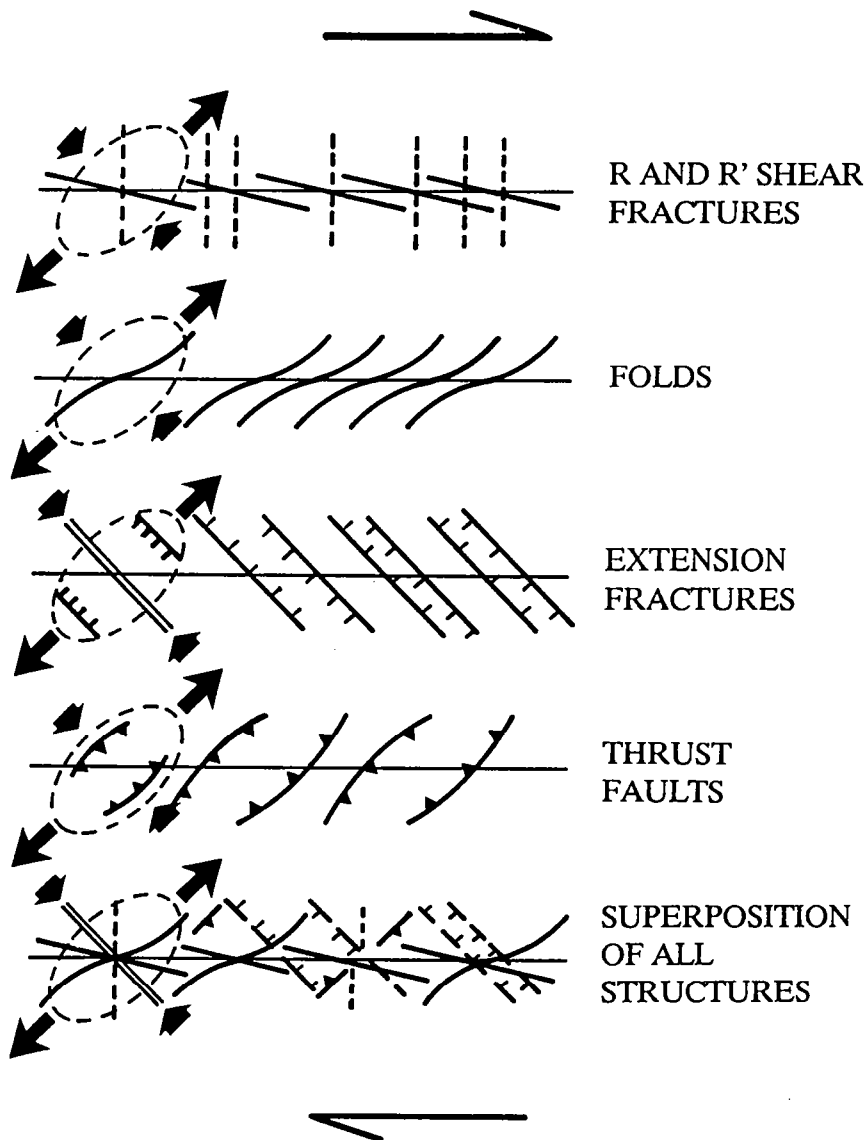
Fig. 7 - 6. Structures associated with a right-lateral wrench zone (redrawn from Sylvester, 1988).
