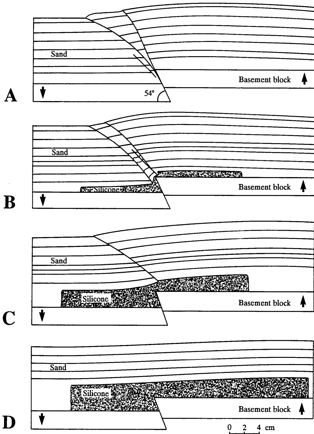
Fig. 4 - 23. Line drawings of cross sections through faulted zones formed above a 54° basement fault with the same pure reverse dip-slip (2.8 cm) and the same SS/DS = 0 ratio, with different rheologies. Sections have been located on the figure 22.
