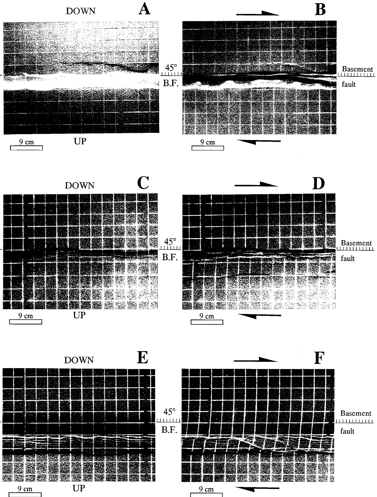
Fig. 5 - 18. Reactivation in pure strike-slip mode of a 45° normal basement fault. Photographs of top views of experiments after dip-slip stage (left) and final stage (right), for different rheologies: A,B, pure brittle model; C,D, 5 cm of sand overlying 1 cm of silicone; E,F, 4 cm of sand overlying 2 cm of silicone.
