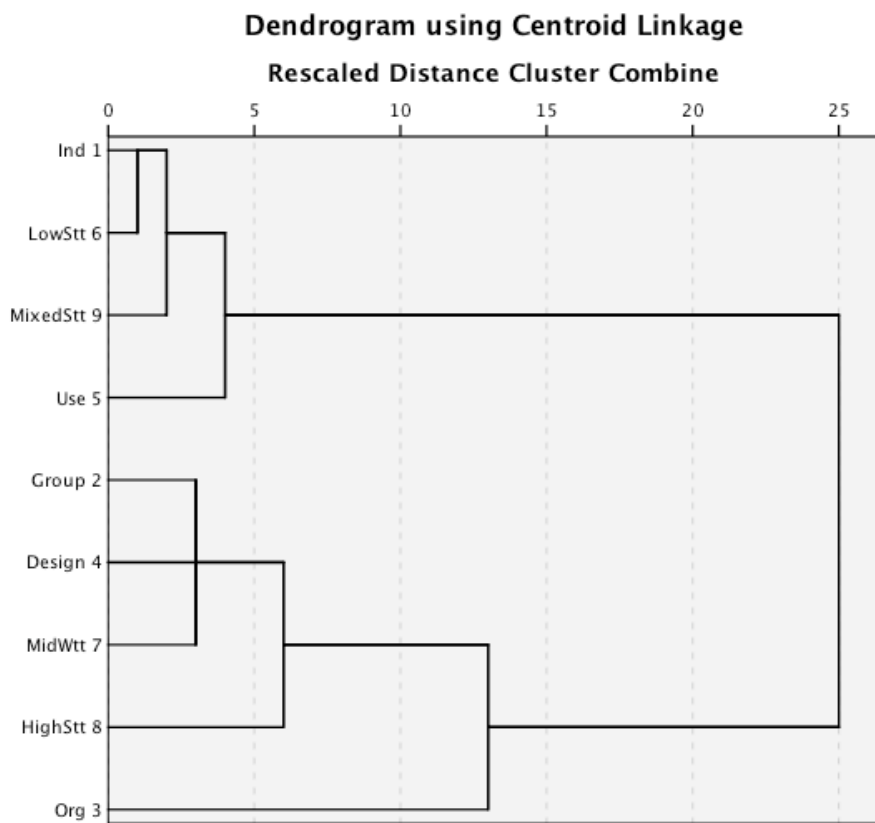
Figure 36. Highest neighborhood dendrogram
