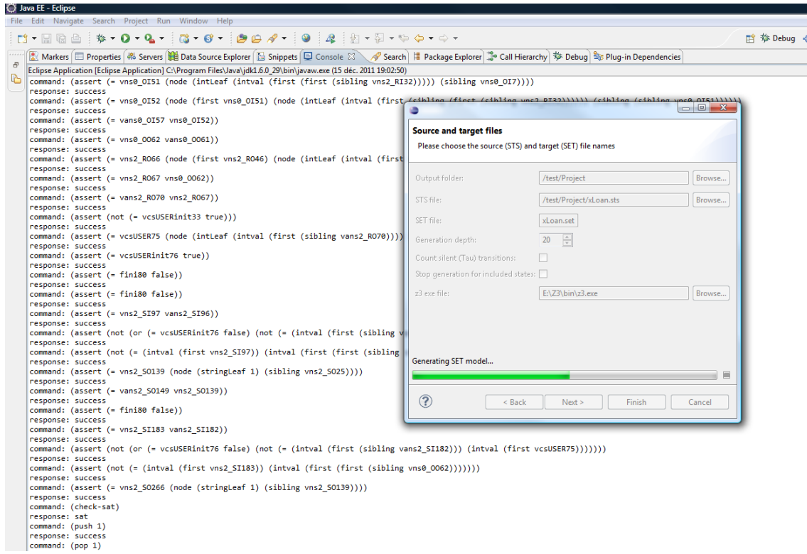
Figure A.6: xLoan Example – Symbolic Execution Tree - Overview of the STS2SET tool
