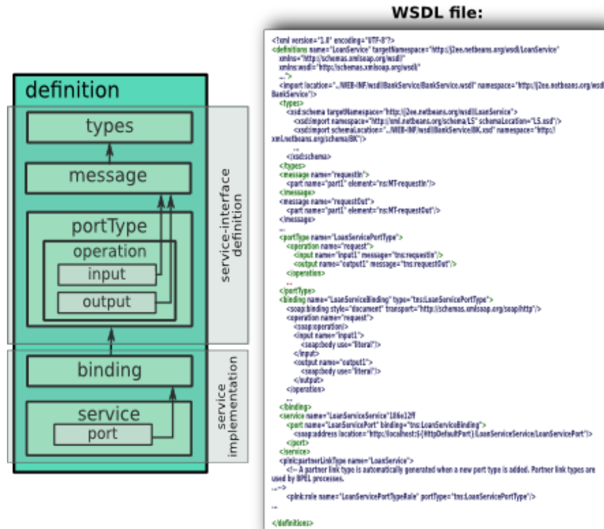
Figure 2.3: WSDL 1.1 structure
