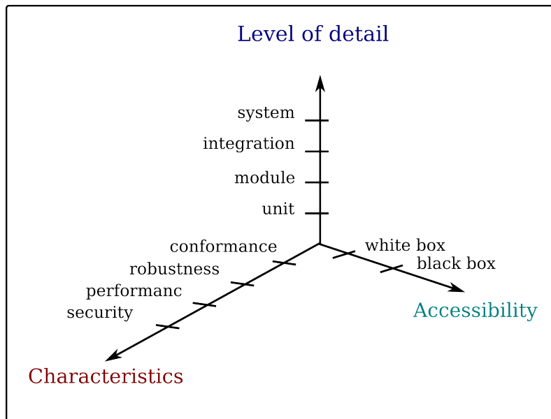
Figure 2.10: Tests classification
