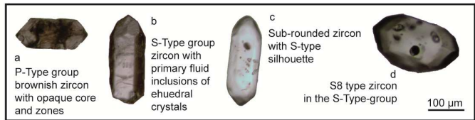
Fig. 29: Plate 12. Photomicrographs of samples from the Western Alps
