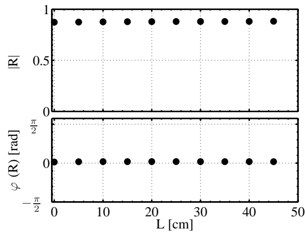
Figure 5.8: On-the-fly measurements, on the combustion rig, of the reflection coefficient of plate P8 for various cavity depths of the ICS and a SPL \geq 140 dB.
