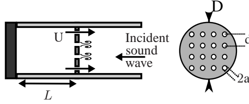
Figure B.1: Geometry of a perforated panel backed by a cavity with bias flow. d \ll \lambda , a \ll L . U bias flow velocity through the apertures, a aperture radius and d aperture separation distance.
