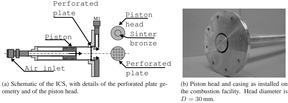
Figure 2.6: Adaptive impedance control system (ICS) schematic (a) and photo (b).
