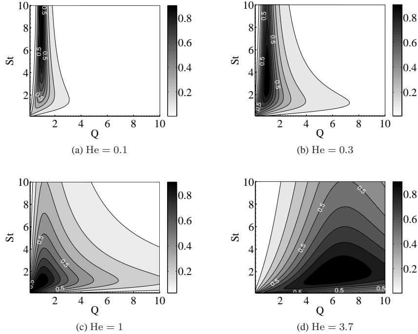
Figure B.6: Absorption coefficient for different Helmholtz numbers
