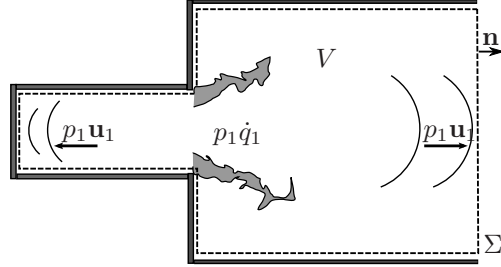
Figure 1.6: Illustration of the source term and acoustic fluxes.
