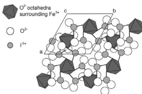
Figure I-3 : Structure cristalline de Fe(IO 3 ) 3
