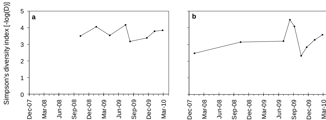
Figure 22: Temporal evolution of Simpson's diversity index. The values calculated with Statfingerprints are presented for (a) the population originating from the bloom of 2008 and (b) the population originating from the bloom of 2003.
