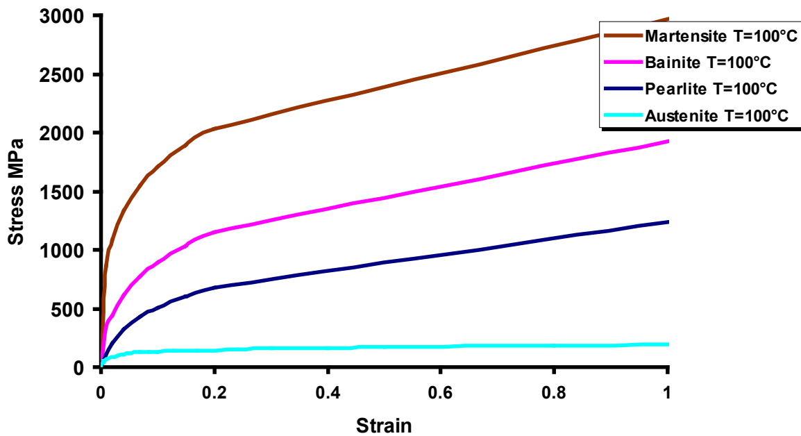
Figure 4.14 Stress-strain flow curve for each phase obtained using equation 3.2 for T=100^{\circ}\text{C}
