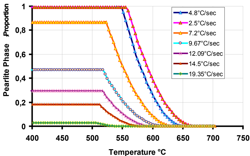
Figure 3.25 Predicted evolution and phase fraction of Pearlite after different temperature histories
