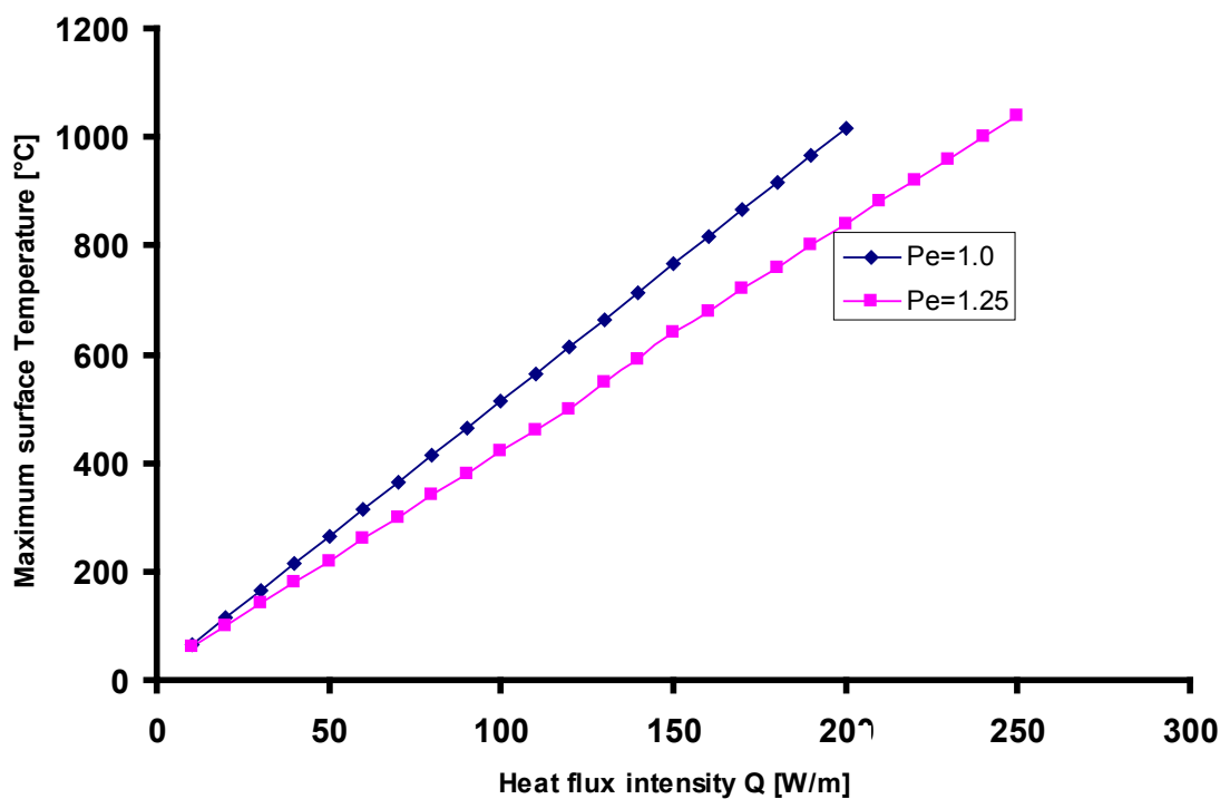
Figure 5.27 Effect of the Peclet number Pe on the maximum surface temperature function of the heat flux intensity Q
