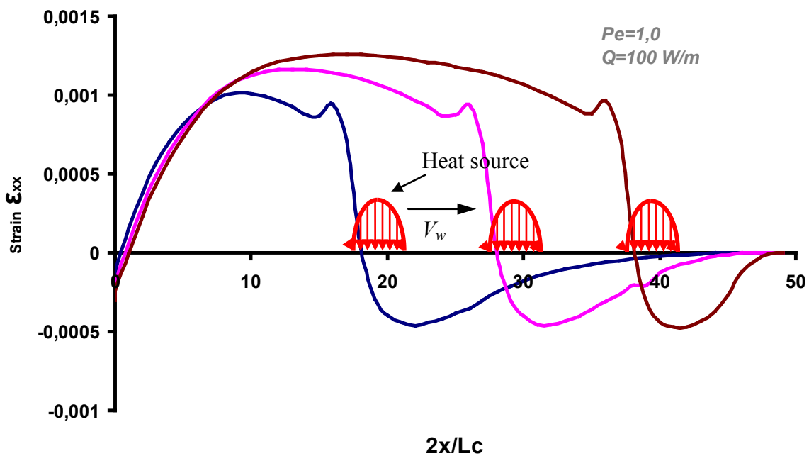
Figure 5.41 Distribution of the longitudinal strain due to the thermal loading only
