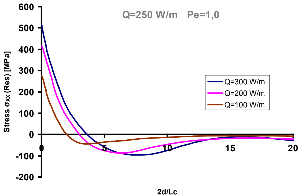
Figure 5.14 Effect of the input heat flux intensity on the longitudinal residual stress profile along depth
