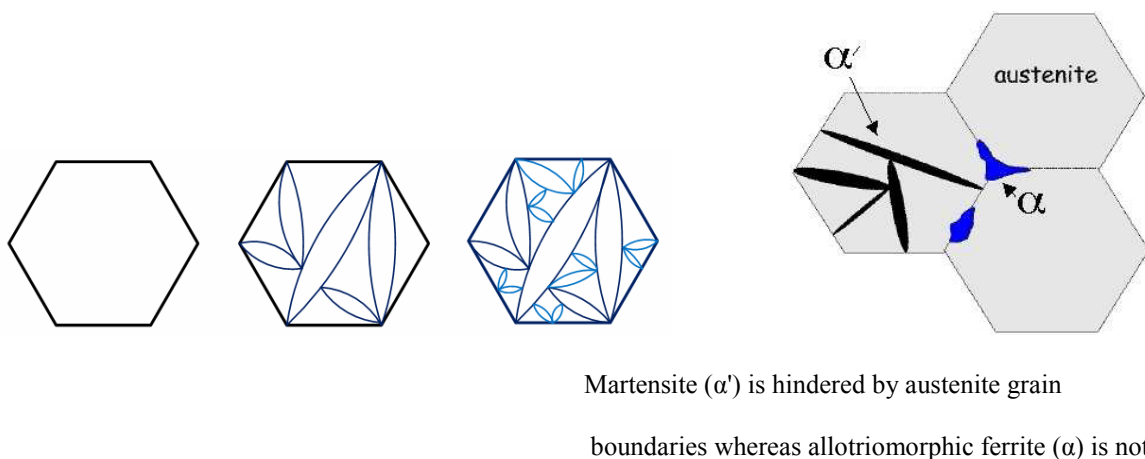
Figure 3.9 Schematics for the formation of martensite plates
