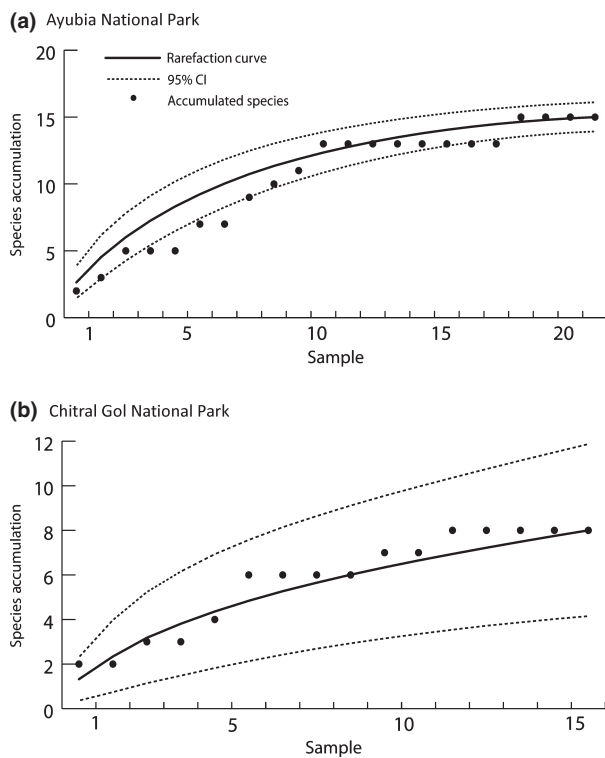
Fig. 5 Species accumulation curves based on the prey species identified in the faecal samples of leopard cat collected in ANP (a) and CGNP (b).
