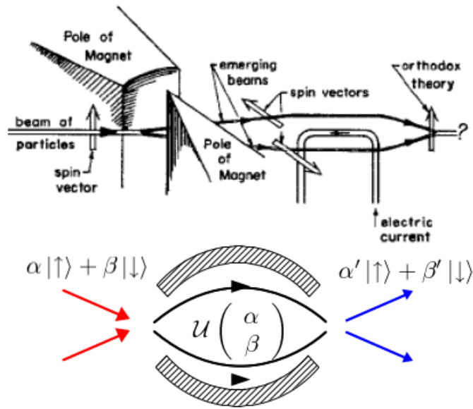
Figure 1.7: Top panel: figure adapted from Ref.[30]: the “classic” Stern-Gerlach experiment. By means of an inhomogeneous magnetic field a given spin projection is decomposed in components in a rotated basis whose relative phase is controlled. Bottom panel: Quantum Gate equivalent of a SGI: the transverse magnetic field acts as a unitary operation on the spinor (\alpha, \beta) resulting in a qubit rotation.
