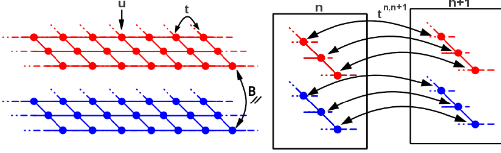
Figure 3.1: Pictorial representation of a tight-binding Hamiltonian. Left panel: spin sublattice (red,blue) where on-site energies ( u ), hopping energies ( t ) and in-plane Zeeman coupling B_{\parallel} are highlighted Right panel: symbolic structure of the coupling between Hamiltonian “slices” through the hopping matrices t^{n,n+1}
