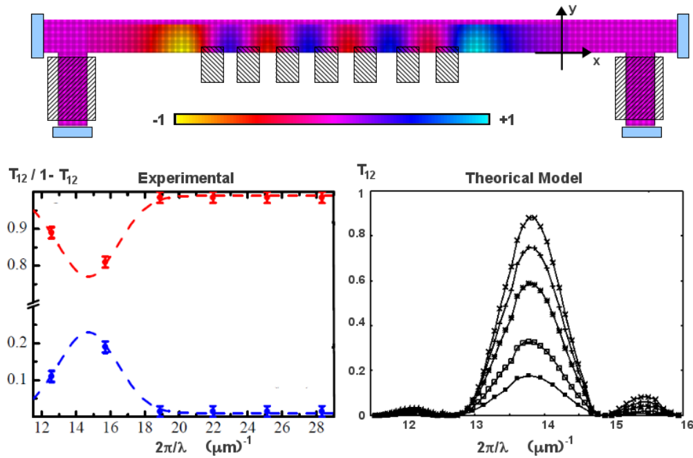
Figure 3.12: Top panel: example of a simulated Hall bar with seven fingers, where the color density corresponding to |B_x| is plotted in color-code (see also Fig.3.11). Bottom left panel: Experimental results demonstrating the selectivity of the engineered charge transfer with respect to \lambda . The dashed line represents a guide to the eye indicating a resonance occurring for a periodicity in between \lambda = 500 nm and \lambda = 400 nm. Bottom right panel: theoretical resonance pattern from RGF calculations, for different values of |B_{||}| (from B_{||} \simeq B_z/100 to B_{||} \simeq B_z/5 ). The qualitative shape of the resonance is consistent with first order perturbation theory (see Section 2.2.3).
