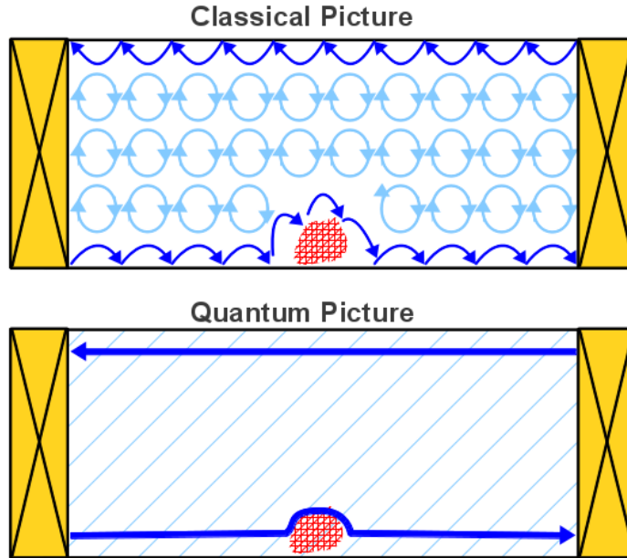
Figure 1.1: Top panel: pictorial view of the classical 2DEG when a strong perpendicular magnetic field is applied. Cyclotron orbits are closed in the bulk while they are “skipping” along the edge. The red hatching represents some localized smooth potential fluctuation. Bottom panel: quantum view of the IQH effect, chiral (unidirectional) channels connects the terminal, irrespective of the localized smooth perturbations.
