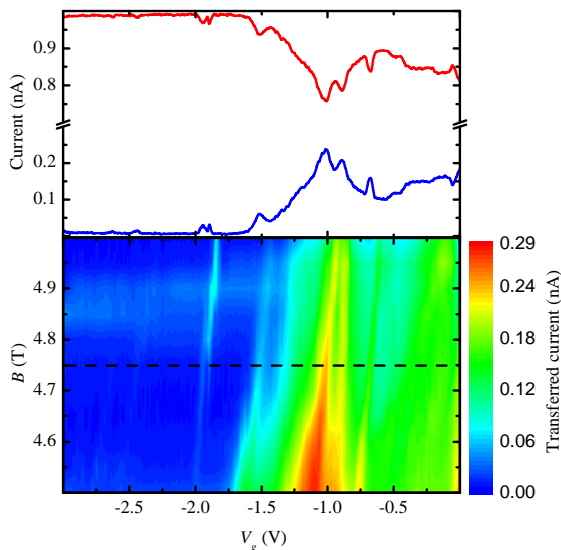
FIG. 4: Tuning of the coupling between spin-resolved edge states with gate voltage and magnetic field. Upper panel: Dependence of the transmitted current I_{\uparrow} (red curve) and transferred current I_{\downarrow} (blue curve) upon the voltage V_g applied to activated nano-finger set (data taken for the nano-finger set with \lambda = 400 nm and for B = 4.75 T). For V_g < -2.0 V the nano-finger are effectively decoupled from the edges and are not able to induce a net transferring of current (off-regime); for V_g \simeq 0 instead the edges feel the presence of the nano-fingers and a non-zero transfer of current is evident. For intermediate values of V_g a series of pronounced peaks in I_{\downarrow} are evident. Lower panel: contour plot of I_{\downarrow} upon V_g and B (again data taken for the nano-finger set of periodicity \lambda = 400 nm). The horizontal line indicates the center of the \nu = 2 plateau ( B = 4.75 T).
