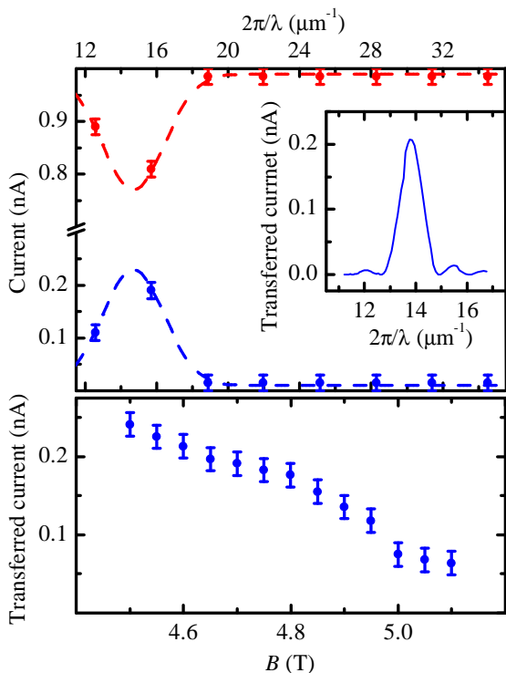
FIG. 3: Measurements of the coupling of spin-resolved edge states. Upper panel: Red data points and blue data points correspond to the transmitted currents I_{\uparrow} and transferred current I_{\downarrow} , respectively, as a function of the inverse periodicity of the activated set of nano-fingers. All data have been measured at the working point B = 4.75 T and T = 250 mK. The measured transferred current I_{\downarrow} is guided by a dashed line which demonstrates selectivity of nano-magnet at periodicity between \lambda = 400 nm and 500 nm. The inset shows the theoretical prediction of the transferred current based on the Landauer-Büttiker transport formalism (see methods). Lower Panel: measured transferred current I_{\downarrow} as a function of the perpendicular magnetic field B (here the periodicity of the activated nano-finger is \lambda = 400 nm).
