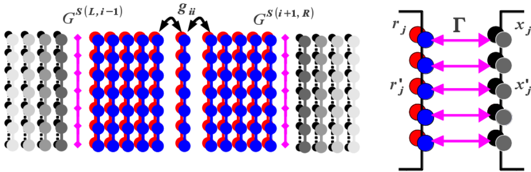
Figure 3.2: Schematics of a two-terminal system on a lattice. Left panel: pictorial view of the calculation procedure for the numerical local charge density (3.13) Right panel: pictorial view of the coupling due to system-lead matrices \Gamma_{r_j r'_j}^j (3.12)
