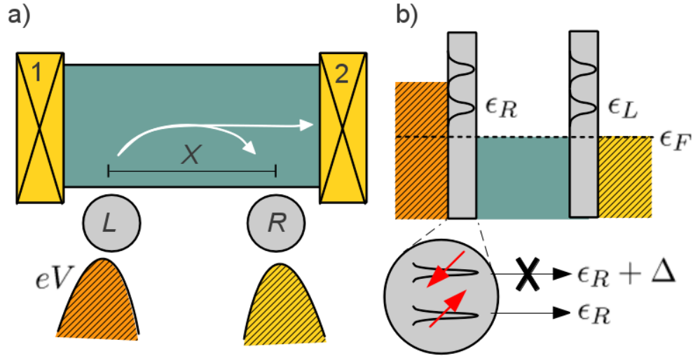
Figure 4.5: Setup of the gedanken experiment. Left panel: Planar view of the four-terminal device, reservoirs are Ohmic contacts 1,2 and the shaded regions under the quantum dots L,R are reservoirs maintained at chemical potential \mu_L and \mu_R . Contacts 1,2 are intended to be very far from L,R, ideally at infinity, and they are grounded. Only the reservoir connected to L is biased with respect to the ground. White arrows indicate the only non-compensated electronic currents. Right panel: Energy level view of the transport experiment. Transport occurs through resonances present in the quantum dots which are accessible within the transport window determined by the bias eV . Zoom inset: the tilted arrows represent the magnetic fields in the dots (see Eq.(4.34)), which allow only one spin-projection in an arbitrary basis to be transmitted in the propagation region.
