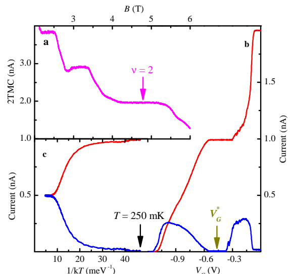
FIG. 2: Working parameters in the quantum Hall regime at filling factor \nu = 2 . a) Plot of the two terminal magneto-current (2TMC) measured at a temperature of 250 mK with an a.c. voltage excitation of V = 25.8 \mu\text{V} at 17 Hz. The value of magnetic field B = 4.75 T, indicated by an arrow, is used to place the 2DEG approximately at the center of the \nu = 2 plateau. b) Plot of the currents I_{\uparrow} (red) and I_{\downarrow} (red and blue curves, respectively) measured at the current terminals red and blue (Fig. 1b) with the voltage V_G applied to the gates G1 and G2 at \nu = 2 and with the voltage V_g applied to the array and equal to V_g = -3 V. The value of V_G is set to V_G^* , indicated by an arrow, for separately contacting the spin resolved edge channels (see Fig. 1b). c) Temperature dependence of I_{\uparrow} (red) and I_{\downarrow} (blue) currents shows enhancement of relaxation between spin resolved edge channels with increasing temperature. Thermally mediated mixing of currents becomes negligible at T = 250 mK.
