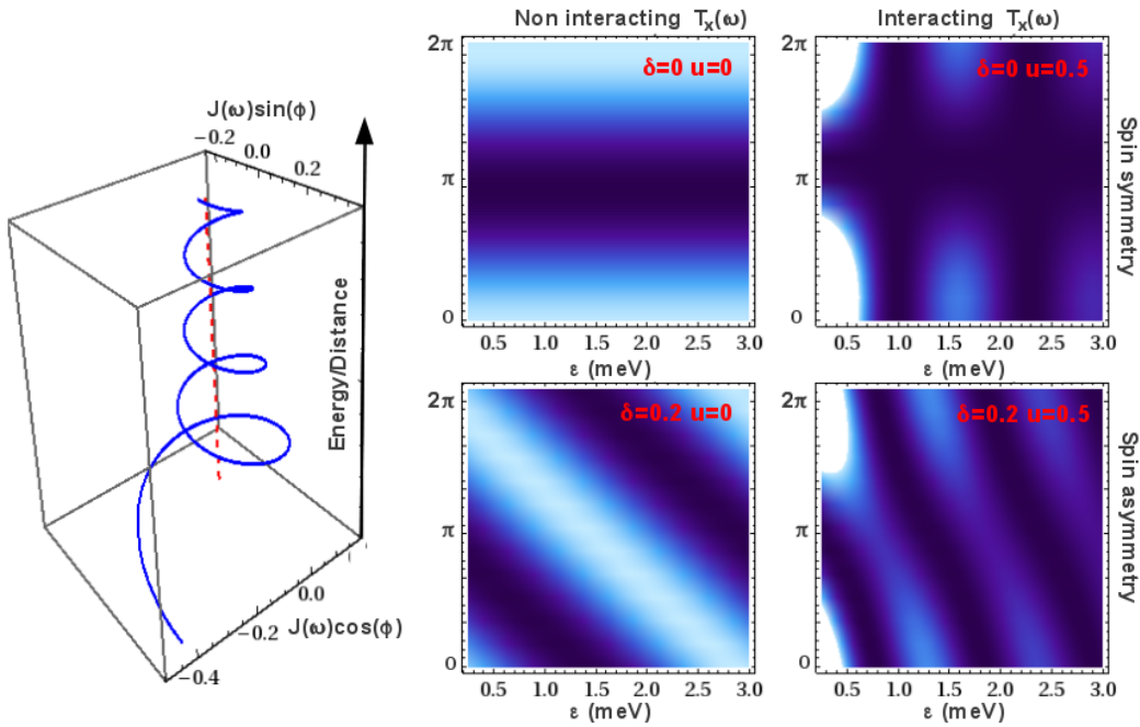
Figure 4.8: Left panel: Most-likely trajectory of the electronic state in the polar plane represented by the phase-angle \phi , as a function of the distance of detection (or equivalently the energy of detection). The trajectory is defined by the \phi which gives maximum of the current signal J(\omega) computed through Eq.(4.48) for a given \epsilon/x . Right panel: Elastic transmission coefficient for \theta_R = \theta_L = \frac{\pi}{2} (lighter colors are closer to unity, darker closer to zero), in functions of energy and the phase difference \phi = \phi_R - \phi_L . Parameters of the model are the same as Fig.4.3, and crossed contributions to the current has been neglected (the plots start at 0.3 meV of the Fermi energy, so the NCA is justified)
