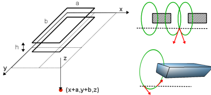
Figure 3.9: Left panel: scheme for calculation of the magnetic field of Cobalt fingers (Reference to Eqs.3.16-3.19). Right panel: pictorial view of the two components of the fringing field. Dashed rectangles are meant to be section (in the z-x plane) of the Cobalt finger.
