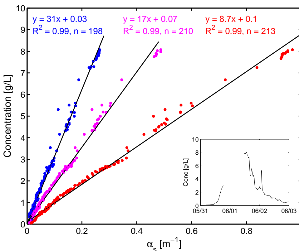
Figure 6.14: Relationship between concentration from optical turbidity and sediment attenuation measured with the 300 kHz (blue), 600 kHz (magenta) and 1200 kHz (red) H-ADCPs between May 31 and June 3, 2010 at Romans-sur-Isère. The least-squares linear regressions to the data are shown, R^2 is the correlation coefficient and n is the number of data points used for the fit.
