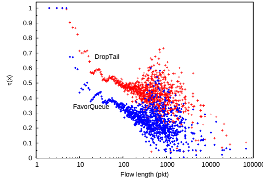
FIGURE 6.10 – RTO recovery ratio according to flow length
