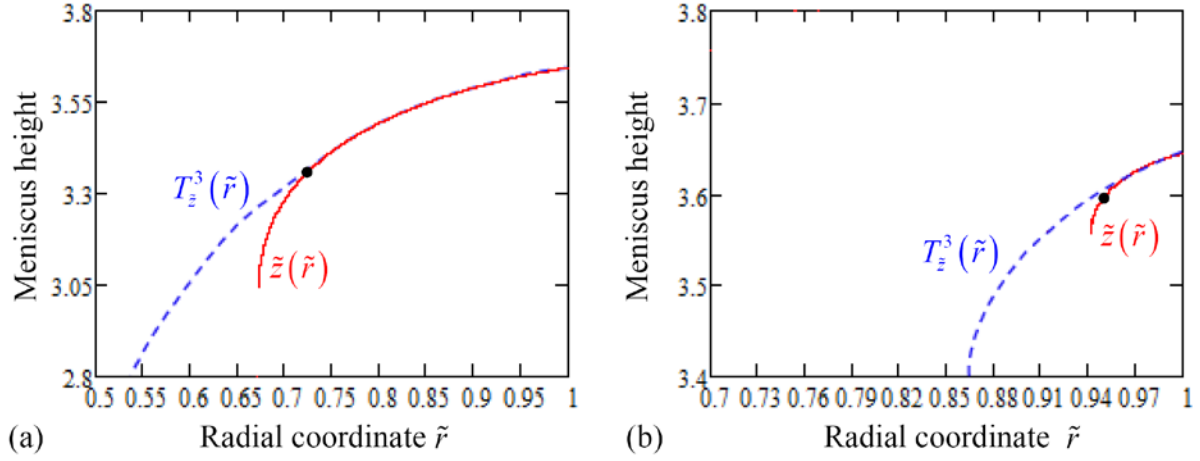
Figure 2.16 Approximated menisci T_z^3(\tilde{r}) (dashed line) and real (numerical) concave menisci \tilde{z}(\tilde{r}) corresponding to La = 51.532 (a) and La = 60 (b) for InSb , \tilde{H}_a = 14.545 . The places where the growth angle ( \frac{\pi}{2} - \alpha_e = 1.13446 rad) is achieved are shown by the black dots.
