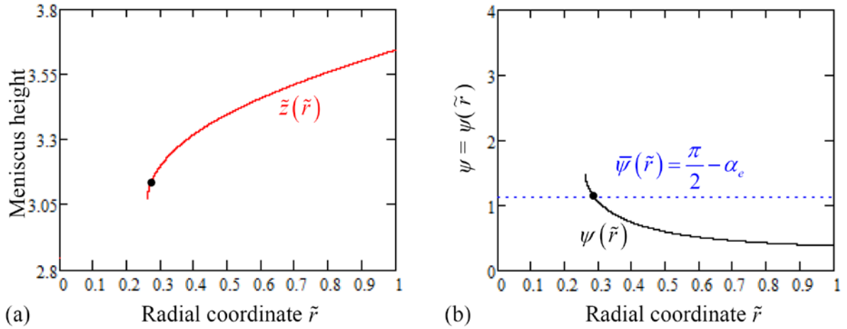
Figure 2.10 (a) Computed meniscus shape \tilde{z}(\tilde{r}) and (b) meniscus angle \psi(\tilde{r}) corresponding to
