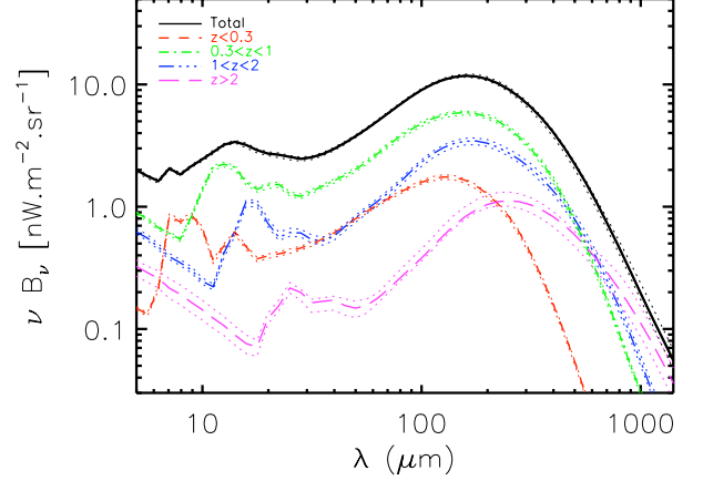
Fig. 1. CIB per redshift bins from the model of B thermin et al. (2011). The high redshift contribution increases with the wavelength.
