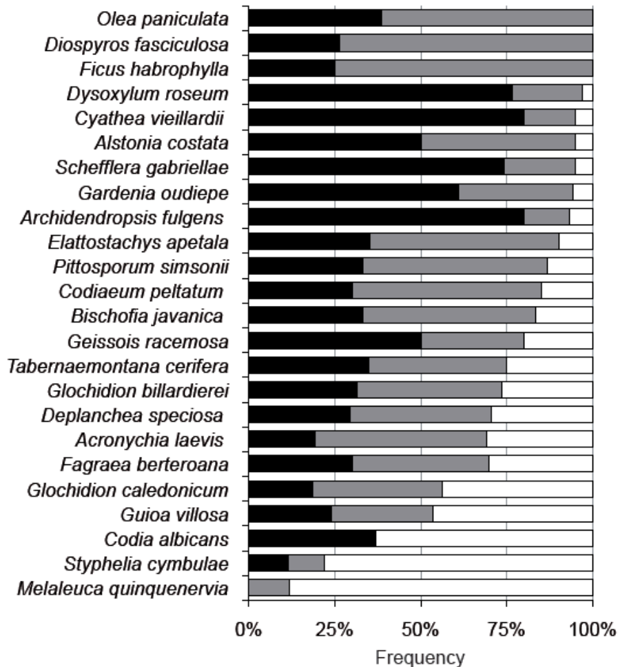
Figure 4.5 Frequency of collects of species herbarium specimens in open (white), semi-open (grey) and closed ecosystems (black). Species were classified into a decreasing order of frequency into open ecosystems and into an increasing order of frequency into closed ecosystems.
