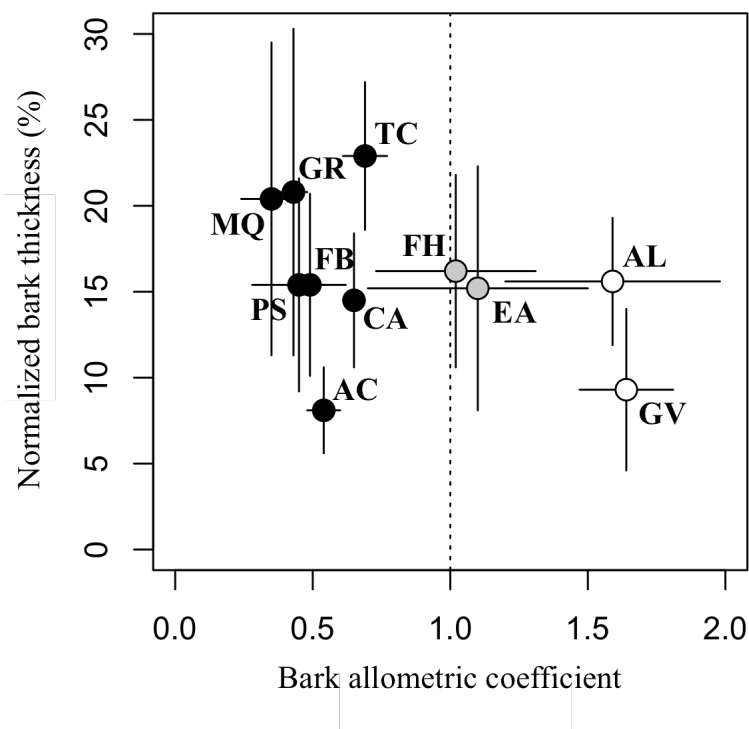
Figure 6.4 Normalized bark thickness against bark allometric coefficients (bars represent one standard-error). The two-letter codes refer to species (see Table 6.1).
