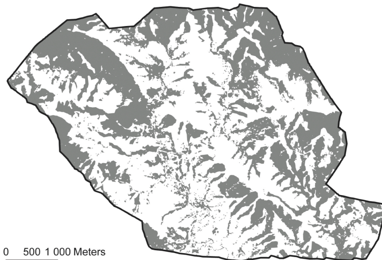
Forested areas in 2000
