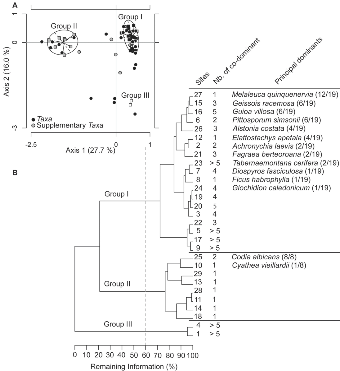
Figure 4.3 Projection of sites and species on the two first axis of the FCA (A) with 3 identified sites clusters groups (Group I, II and III) identified on the HAC dendrogram (B). For each site, the number of co-dominant species determined by the dominance analysis and for each groups the list of the dominant species (with the number of sites within the cluster groups where the species was dominant against the total number of sites of the cluster group).
