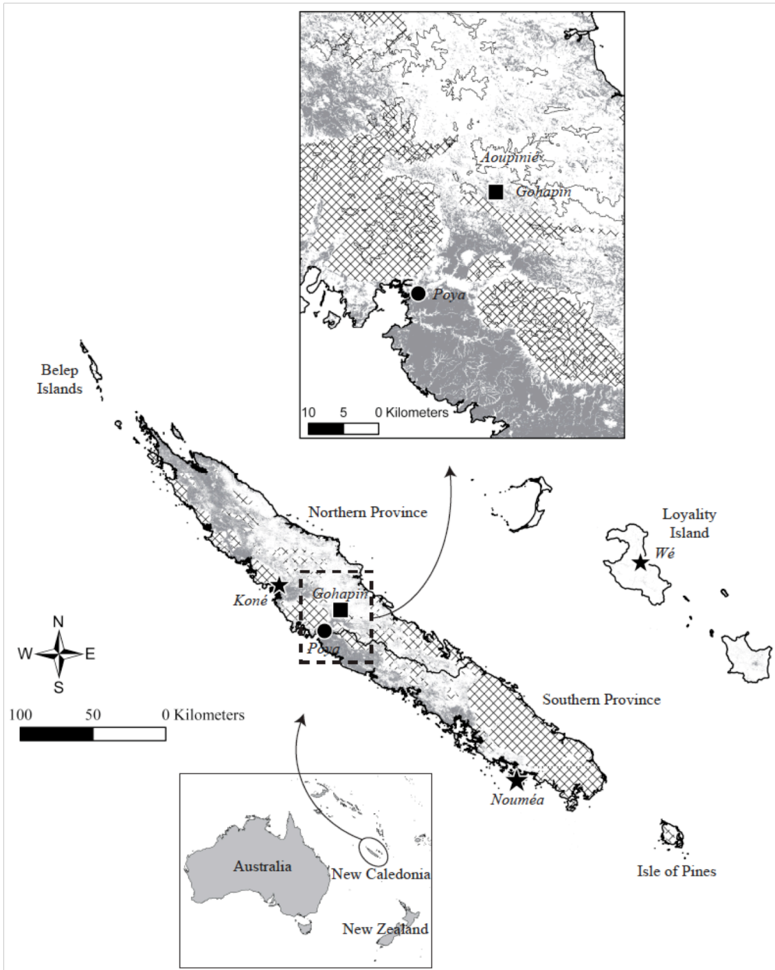
Figure 6.1 Location of the studied area. Sampling were performed on the western side of the Aoupinié (1006 m) between the Gohapin tribe and Poya in the middle of the New Caledonian main island. Grey areas represent the savannas areas (from SGT 2008) and hatched areas represent the ultramafic substrate encompassing peridotite and serpentinite (from Fritsch 2011). In the insite, contours represent the areas > 500 and 1000 m asl.
