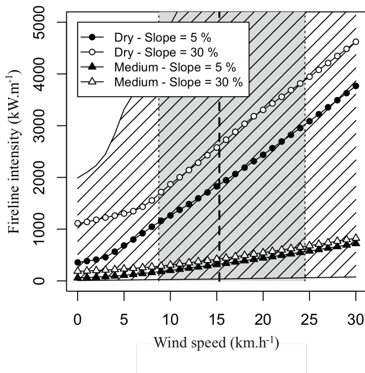
Figure 6.2 Simulated savanna fires fireline intensity ( I ) for several realistic scenarios of fuel moisture (dry and medium), slope (5 % and 30 %) and wind speed (from 0 to 30 km/h). Symbols represent the median of I for different scenarios. The hatched area represents a 95 % CI for all scenarios taken together. The vertical bold dotted line represents the median wind speed during dry season and the two vertical dotted lines represent the 0.25 and 0.75 quantiles.
