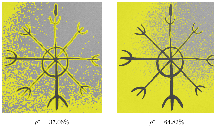
Figure 25: Negative impact of the test (53) (right) against the test (39) (left) for segmenting the image "viking-symbol2" with a TV+L^2 model. On both images, the reduced graph is superimposed in yellow on the image. In these experiments, we take the same set of parameters than those used in Table 5. Observe how the test (39) can remove a large part of nodes due to the raking light, unlike the test (53).
