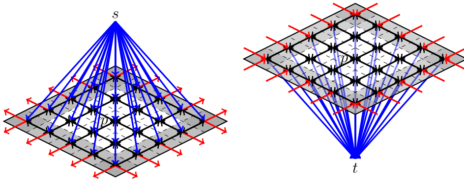
Figure 24: Illustration of the exact test (53). In both situations, we remove the central node p from \mathcal{G} since the contracted capacity of any node q \in \partial B_p is either greater than the sum of the n-links capacities in \sigma_{\mathcal{E}}(q) (left image) or less than the opposite sum of the n-links capacities in \sigma_{\mathcal{E}}(q) (right image).
