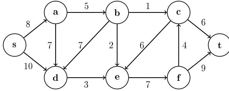
Figure 2: An example of a weighted directed graph with six grid nodes and two terminals.
