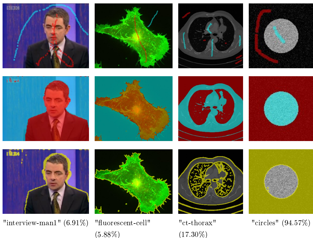
Figure 10: Segmentation results with using a Boykov-Jolly model using NH in connectivity 1. For each image, we represent the seeds (first and fourth rows), the segmentation (second and fifth rows) as well as the reduced graphs (in yellow on third and sixth rows) superimposed on the original image by transparency. The minimum relative reduced graph size \rho^* is also indicated below each sequence of images.
