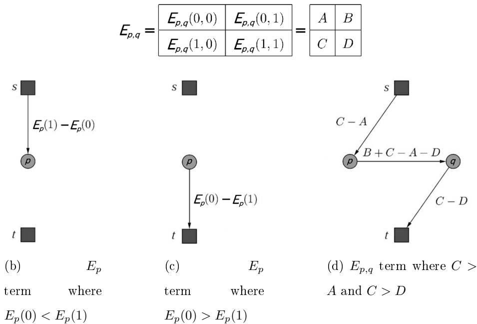
Figure 9: Graph construction in the binary case [KZ04].
