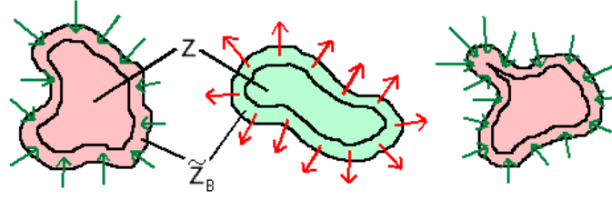
Figure 3: Principle of the reduction. Red area and arrows (resp. green area arrows) denote the flow which get in (resp. out of) Z_B . The nodes from Z are removed since Z satisfies (38). Remaining nodes are typically located in the narrow band Z_B \setminus Z .
