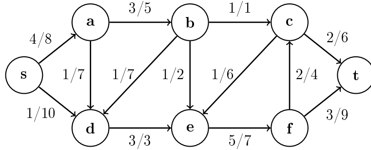
Figure 5: A valid flow on a weighted directed graph. Left numbers denote flow while right numbers denote edge capacities.
