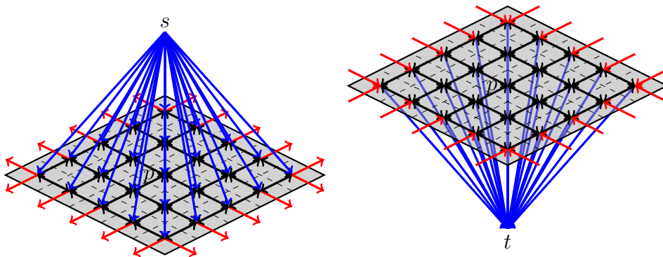
Figure 4: Illustration of the heuristic test (39). In both situations, we remove the central node p from \mathcal{G} if contracted capacities are all greater than +\delta_r (left image) or all less than -\delta_r (right image) inside the square window B^r .
