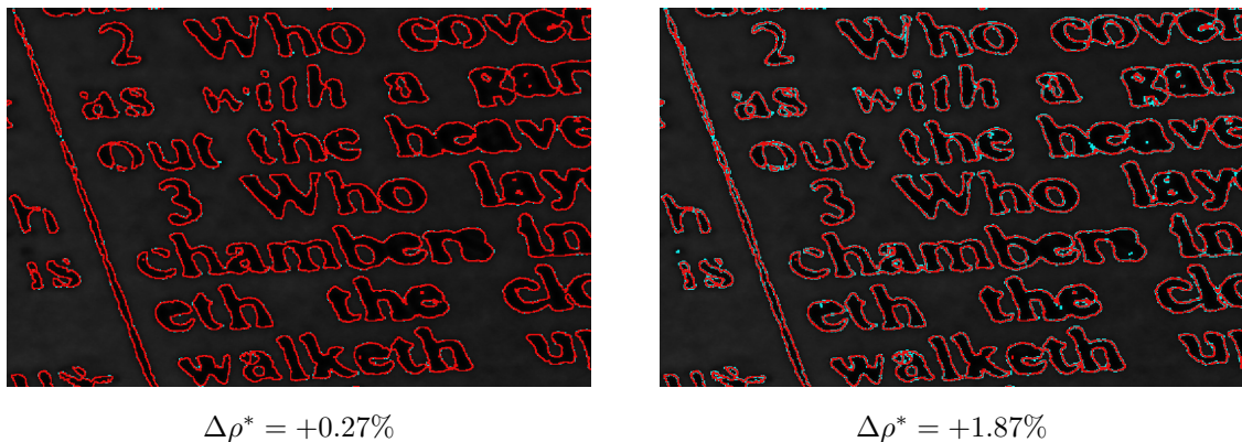
Figure 26: Positive impact of the test (53) against the test (39) for segmenting the image "book" with a Boykov-Jolly model using NH (left) and GMM (right). Notice that we take in these experiments the same set of seeds and parameters than those used in Tables 6 and 7. On both images, we represent the reduced graphs using the test (39) (cyan) and (53) (green) superimposed on a zoomed version of the original image. The intersection is drawn in red. Observe how the test (53) results in thicker bands around the object contours unlike the test (39).
