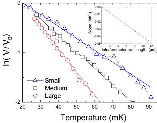
Figure 4.3: Semi-log plot of the visibility as a function of the temperature for three samples of arm lengths L = 5.6, 8, 11.3 \mu\text{m} . The visibility decays exponentially with the temperature with a rate T_\varphi^{-1} which increases linearly with L (inset) [2].
