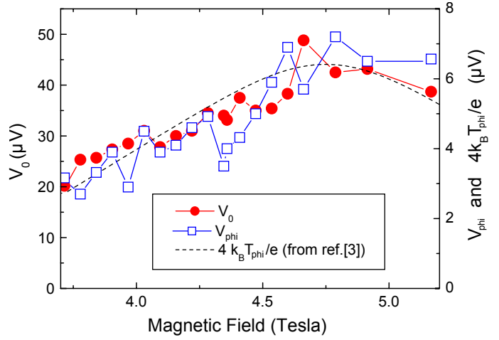
Figure 4.5: Left scale: V_0 as function of the magnetic field (full red circles). Right scale: V_\varphi (empty blue squares) and 4k_B T_\varphi/e (dashed line) as function of the magnetic field. Fluctuations of V_0 with the magnetic field are proportionnal to the ones of V_\varphi and 4k_B T_\varphi/e . V_\varphi and 4k_B T_\varphi/e fall on each other. All these quantities show a maximum at the end of the \nu = 2 plateau [1, 3].
