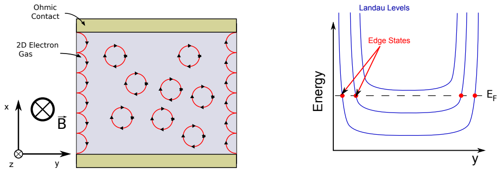
Figure 3.6.: (left) Semi-classical picture of the ES: in the bulk electrons describe circular cyclotron orbits while they drift along the edges following equipotential lines. (right) LLs as function of the position in the 2DEG. ESs form at the lines (red points on the picture) where the Fermi energy cross the LLs.
