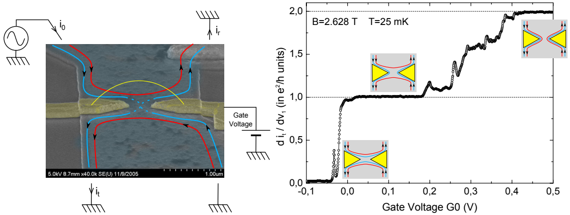
Figure 5.1.: (left) Scanning electronic microscope (SEM) view of a QPC. In false colors, the 2DEG is blue, the two gates forming the QPC are yellow. The \nu = 2 ESs are figured with the IES (in red) being fully reflected and the OES (in blue) being partially transmitted. (right) The differential conductance across the QPC is plotted as a function of the gate voltage in units of the quantum conductance G_Q = e^2/h .
