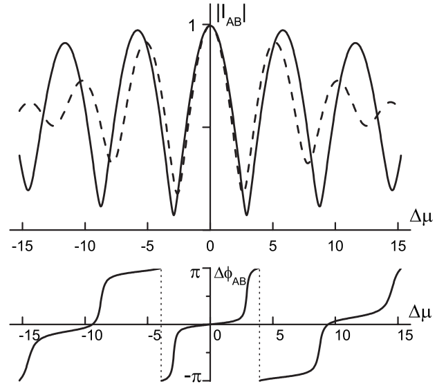
Figure 6.4: Visibility and phase shift as function of the bias computed by Levkiviskyi et al [6]. The multiple extinctions are reproduced along with the phase rigidity between them. The \pi phase jumps are recovered. However, the decay of the oscillations with the bias voltage is non-existent unless \Delta L \neq 0 .
