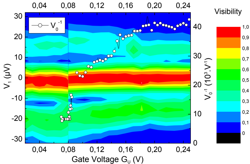
Figure 7.23.: Left scale: colorplot of the normalized visibility as function of the gate voltage V_{G_U} on the x-axis, and the bias voltage V_1 on the y-axis. Right scale: V_0^{-1} as function of V_{G_U} .
