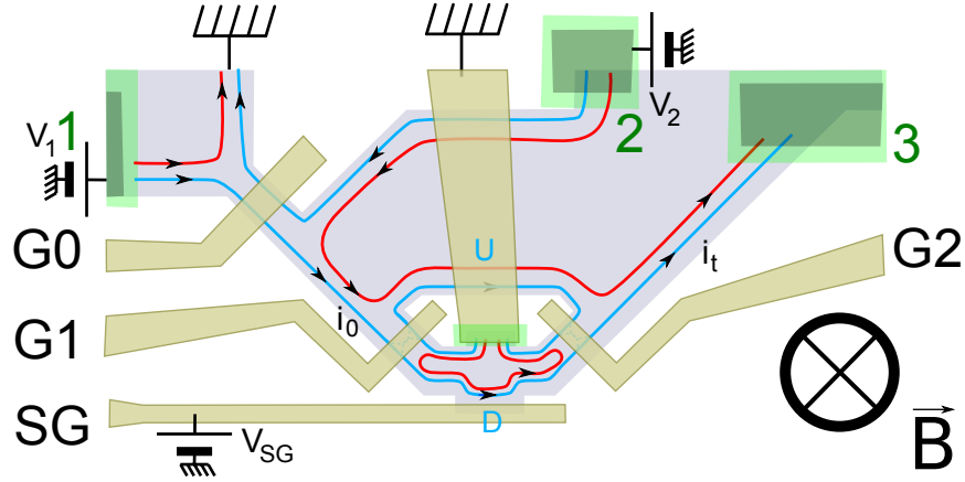
Figure 6.1.: Schematic of the Mach-Zehnder interferometer at \nu = 2 . The injecting QPC, G0 is set as to fully reflect the IES. The interfering electrons are injected at contact n°1 with the energy E_F + eV_1 , where V_1 is the dc voltage applied to contact n°1. Interferences are revealed by sweeping the gate voltage V_{SG} applied to the side gate SG or by using the IES in the upper arm like a gate polarized with the dc voltage V_2 applied to contact n°2. The latter method gives access to the coupling between the IES and the OES in the upper arm (¶ 4.3.3).
