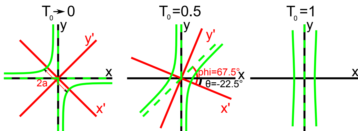
Figure B.9.: On this figure, we schematized the evolution of the hyperbola representing the zeros of the visibility in the V_1 - V_2 plane for different values of \mathcal{T}_0 . The original coordinate system x - y is in black. The new system of coordinates x' - y' is in red and has been rotated by the angle \theta compared to the old one. The asymptots have an angle \pm\varphi with respect to (Ox') and are represented in by green dashed lines. The hyperbola is a green solid line. (left) \mathcal{T}_0 \rightarrow 0 : the new coordinate system is rotated by an angle \theta = -\pi/4 . The asymptots are the axes of the old system. (center) \mathcal{T}_0 = 0.5 : the new coordinate system is rotated by an angle \theta = -\pi/8 . The hyperbola's opening angle is 2\varphi = 3\pi/4 . (right) \mathcal{T}_0 = 1 : the new coordinate system is identical to the previous one, the hyperbola is reduced to two verticals at x = \pm a .
