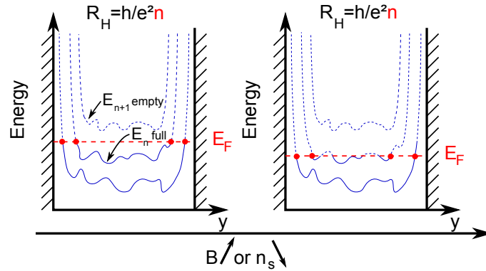
Figure 3.8.: (left) The n^{\text{th}} energy level is full and the n+1^{\text{th}} is empty ( \nu = n is an integer). The Hall resistance is quantized: R_H = h/\nu e^2 . (right) As B increases, the Fermi energy decreases relatively to the energy levels. The n^{\text{th}} level empties progressively into the regions below the Fermi level. The quantization of R_H holds as long as the number of ESs remains equal to n e.g. on a wider range of B than when there is no disorder.
