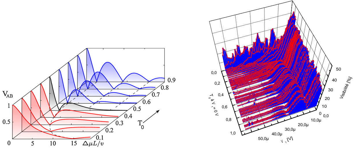
Figure 6.5.: (left) Prediction on a quantum phase transition induced by non gaussian noise at \mathcal{T}_0 = 0.5 from a multiple side lobe structure to a single side lobe structure [16]. (right) 3D plot of the visibility as function of the bias voltage V_1 for various values of the transmission \mathcal{T}_0 at zero bias. The final picture resembles the prediction of Levkiviskiyi et al. .
