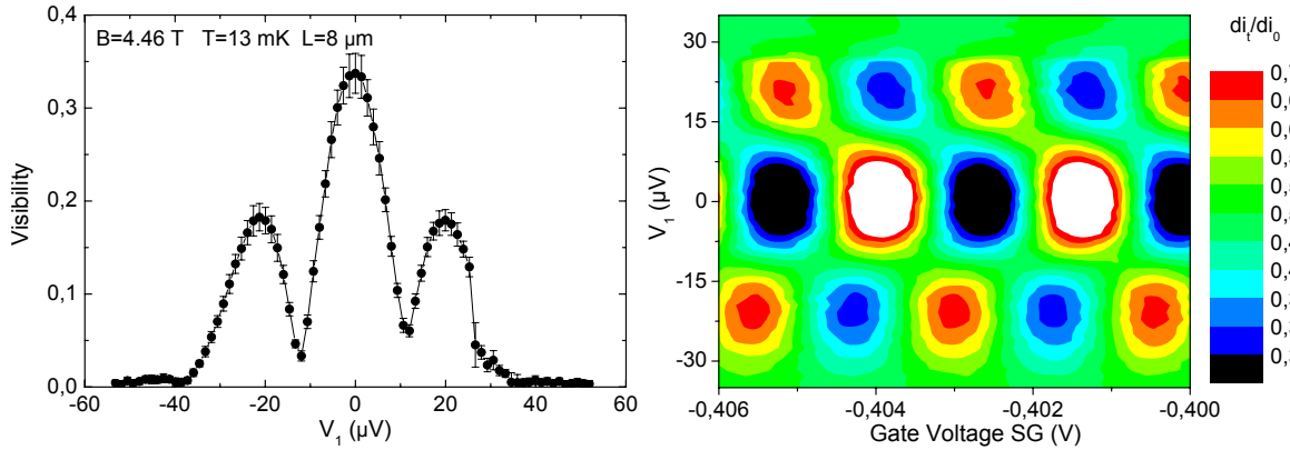
Figure 4.6.: (left) Visibility as function of the bias voltage V_1 showing oscillations with multiple extinctions, for a sample of arm length L = 8 \mu\text{m} , at B = 4.46 T and T = 13 mK. The oscillations are damped. One can distinguish two lobes on each side of the central lobe. (right) Colorplot of the differential transmission of the interfering OES as function of the side gate voltage V_{SG} along the x-axis, and the bias voltage V_1 on the y-axis. The oscillations of the differential transmission as function of V_{SG} are extinguished at V_1 \sim \pm 13 , \pm 37 \mu\text{V} (periodicity \Delta V_1 \sim 25 \mu\text{V} ). Within a lobe the phase of the visibility is rigid, and undergoes \pi -jumps at extinction points.
