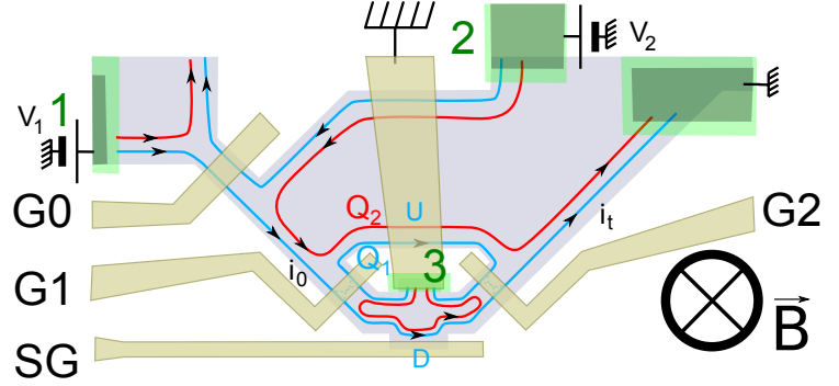
Figure A.1: Schematic representation of the charge injectivity: we have to consider three sources. We are interested in the charge Q_1(Q_2) in the outer(inner) ES.
