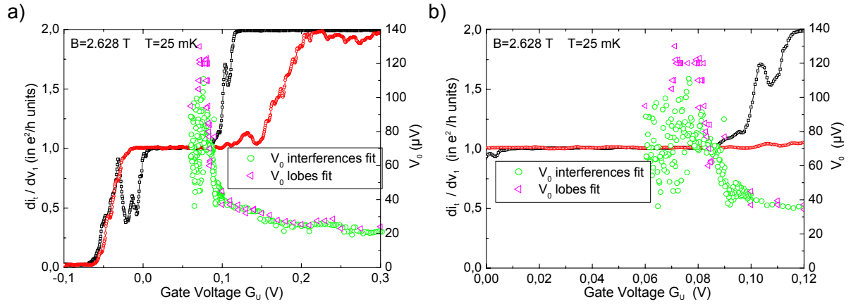
Figure 7.9.: On all graphs G_U transmission through the upper (red curve) and the lower arm (black curve) are figured on the left scale. On the right scale, as function of V_{G_U} : (a) V_0 rises slowly from 25 \mu V to 60 \mu V as T_U decreases from 1 to 0.5 because of the deformation of the IES. It increases sharply at T_U = 0.5 when the IES is disconnected from contact n^{\circ}2 . (b) Zoom. At localization of the IES, V_0 rises sharply and then stabilizes to 120 \mu V.
