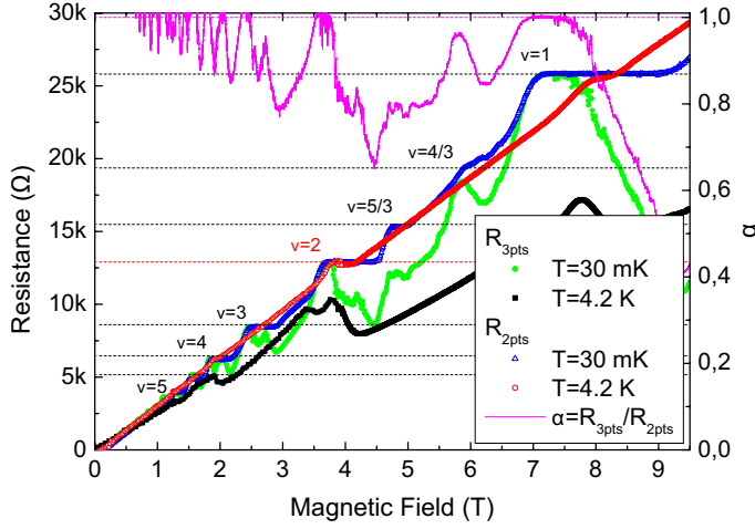
Figure 5.4: Plateaus in R_{2\text{points}} shrink and R_{3\text{points}} lowers as the temperature rises because of variable range phonon-assisted hopping between localized states [18] inducing backscattering. At 30 mK for \nu = 1 , backscattering is absent at the beginning of the plateau ( \alpha = 1 ) and appears as the magnetic field is increased ( \alpha < 1 ). Wires and contacts resistances ( \sim 600 \Omega ) have been subtracted from R_{2\text{points}} .
