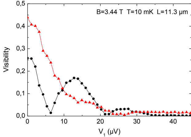
Figure 6.3: Visibility as function of the bias voltage V_1 for two different dilutions of the incoming current in the OES. \mathcal{T}_0 \sim 1 (black curve), \mathcal{T}_0 \sim 0.1 (red curve). The multiple side lobes structure seems to transform into a single side lobe structure and the shape of the visibility as function of V_1 is strongly affected by \mathcal{T}_0 : the width of the central lobe goes from \sim 7 \mu V when \mathcal{T}_0 \sim 1 to \sim 25 \mu V for \mathcal{T}_0 \sim 0.1 .
