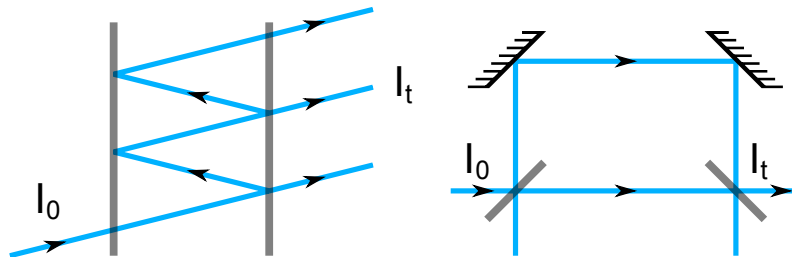
Figure 4.2.: (left) Fabry-Pérot interferometer. These interferometers are more sensitive to thermal smearing because interferences occur between paths of different lengths by construction. (right) Mach-Zehnder interferometer. This is a two-path interferometer: if the two paths have the same ‘optic length’, there is no thermal smearing (§ 5.4.2).
