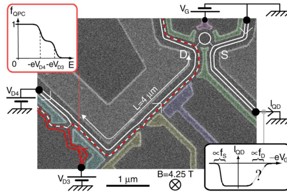
Figure 4.9.: Sample e -beam micrograph. ESs propagate along lines, dashed lines correspond to out of equilibrium distributions. A double step distribution f_{QPC} is created in the OES outside of the QPC in the lower left corner and propagates on a tunable length L . The resulting distribution f_D is probed by the quantum dot (white circle). Colorized QPCs allow to vary the propagation length. The gates not colored are grounded.
