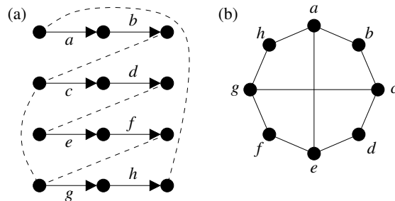
Figure 1.4: A set of P = 4 paths (a), with dashed lines indicating all node pairs representing off-path interference. The resulting graph G is shown in panel (b). Depending on the schedule \mathcal{S} it is possible to obtain equalities in all of Eqs. (1.3)–(1.5). The schedules that achieve this while implying strict inequalities in Eq. (1.6) are: \mathcal{S} = \langle \{a, d, g\}, \{b, f, h\}, \{c, e\} \rangle for Eq. (1.3), with T^1(\mathcal{S}) = 4/3 \approx 1.33 ; \mathcal{S} = \langle \{a, d, f\}, \{b, e, g\}, \{c, f, h\}, \{a, d, g\}, \{b, e, h\}, \{a, c, f\}, \{b, d, g\}, \{c, e, h\} \rangle for Eq. (1.5), with T_{\text{int}}^*(\mathcal{S}) = 4/(8/3) = 1.5 ; and \mathcal{S} = \langle \{a, c, f\}, \{b, e, g\}, \{c, e, h\}, \{a, d, g\}, \{b, d, f, h\} \rangle for Eq. (1.4), with T^*(\mathcal{S}) = 4/(5/2) = 1.6 .
