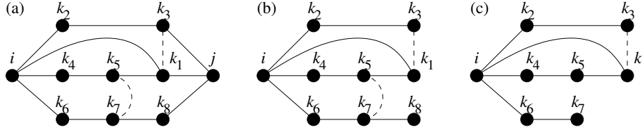
Figure 4.3: The reduction of G_{ij} from the given path set \mathcal{P}_{ij} = \{\{i, k_1, j\}, \{i, k_2, k_3, j\}, \{i, k_4, k_5, k_1, j\}, \{i, k_6, k_7, j\}\} . In panel (a), the graph G_{ij} based on \mathcal{P}_{ij} , where the dashed edge k_1k_3 and k_5k_7 represents the interference (through Step 1, G'_{ij} = G_{ij} ). Step 2 remove j and all edges that touch it (b). Panel (c) presents Steps 3 and 4 (the last one removes only the edge k_5k_7 ).
