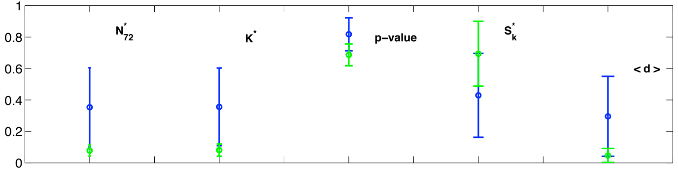
Figure 1.18: Average rate, p -value, K^* -value, aftershock size, aftershock density of thrust (blue) and strike slip (green) mechanism. note that each value is being normalized by its maximum value.
