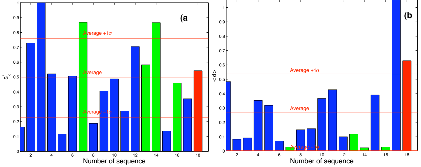
Figure 1.14: Aftershock sequences size and density (a) Normalized aftershock zone length S_k^* (\frac{S_k}{L}) (b) Average density \langle d \rangle = \frac{\text{Total number in aftershock zone}}{S_k} .
