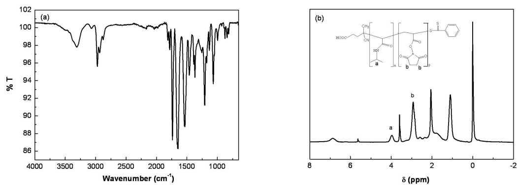
Figure 2.5: IR (a) and 1 H NMR (b) spectra of Cpa-RAFT-PNIPAM-co-NASI copolymer.
