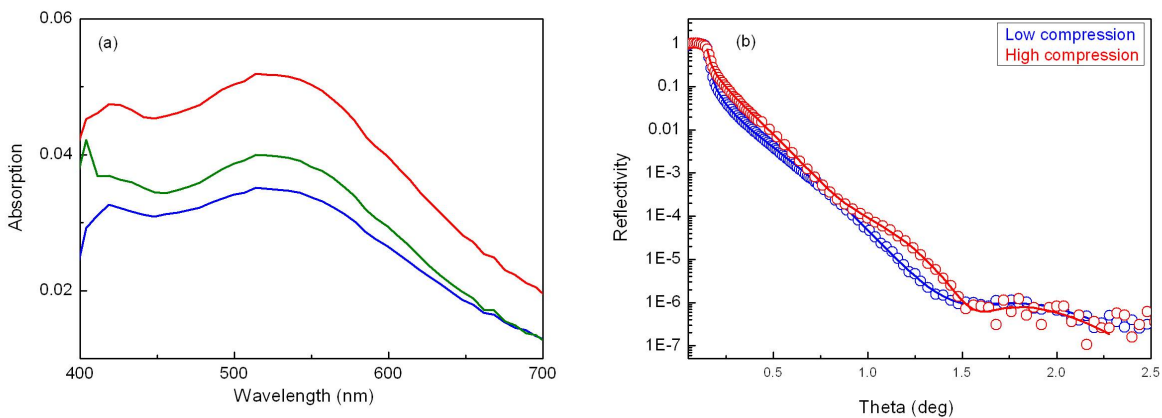
Figure 6.7: Absorption spectra of Au-PNIPAM 24 -PS 28 film at 20°C at different surface compressions (a) the X-ray reflectivity curves.
