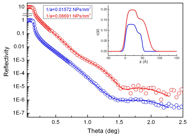
Figure 5.21: X-ray reflectivity curves of Au-PNIPAM 24 -PS 28 surface layer at two different surface compressions (curves are separated vertically for better visualization) (H 2 O, T = 20°C). The solid lines are theoretical best-fit curves with corresponding gold core concentration profiles shown in the inset.
