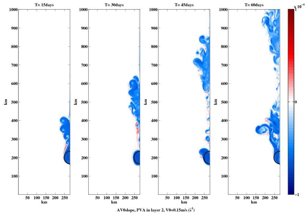
FIG. 3.42: PVA in layer 2 for a Northward current V_0 = 0.15m/s in the coastal, sloping bottom configuration after 15, 30, 45 and 60 days. Notice the plumes of mixed water periodically detaching from the ZMP (the first plume detaches between 15 and 30 days while a second plume grows between 45 and 60 days).
