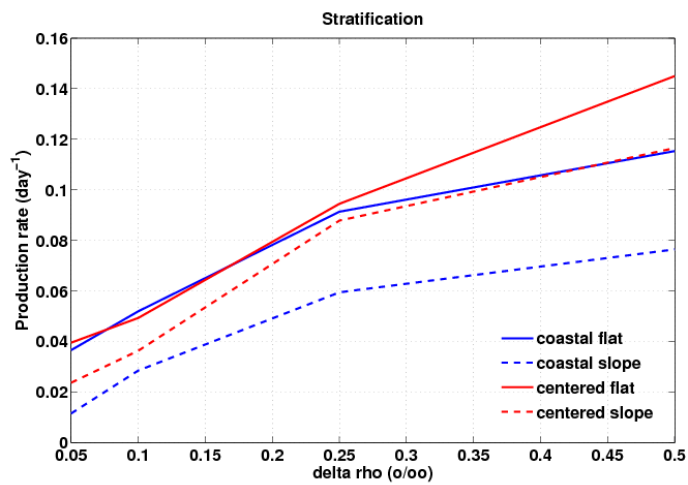
FIG. 3.37: Mean production rate \bar{\tau}_{prod} as a function of the stratification drho for different configurations : centered (red curves) and coastal (blue curves), with and without a sloping bottom (respectively dashed and plain lines).
