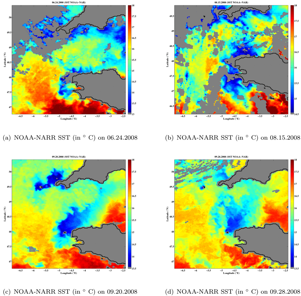
FIG. 3.3: NOAA-NAAR SST maps at different times showing different patterns of the Ushant front. 3.3(a) : The front follows the coast and instabilities develop cross-shore. 3.3(b) : The front extends Northward and Southward and also exhibits instabilities meanders. 3.3(c) : The front detach from the coast and extends in the North-East direction, roughly following isobaths. 3.3(d) : The front is displaced Westward a few days after 3.3(c).
