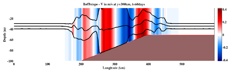
FIG. 3.22: Cross section of the velocity field after 60 days for the centered sloping bottom configuration.
