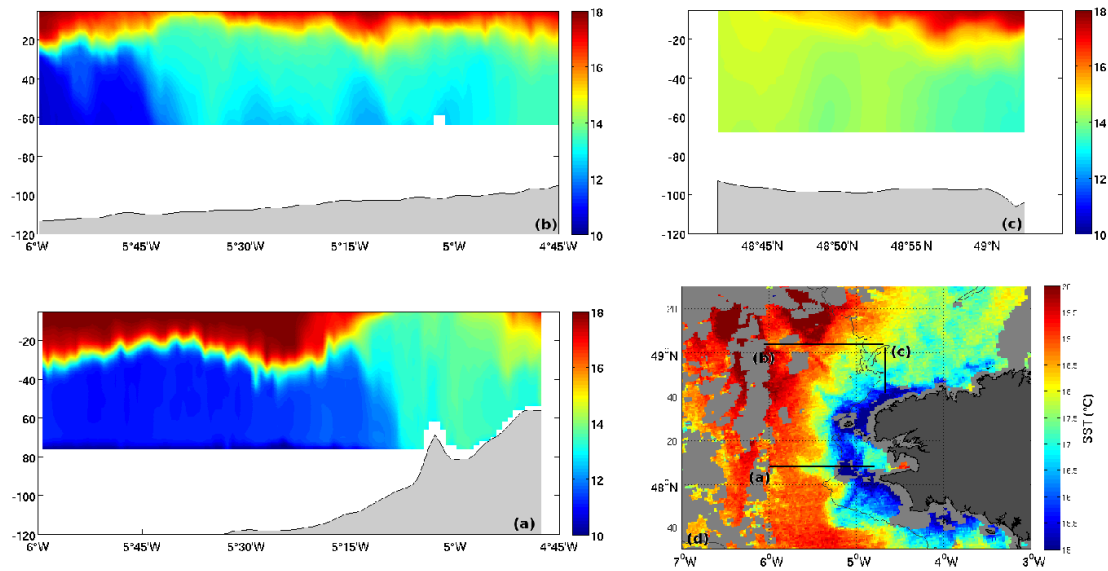
FIG. 3.1: (a), (b) and (c) : Temperature cross-sections obtained during the FROMVAR2010 campaign, between 06.08.2010 and 08.08.2010. (d) : SST measured by satellite on 08.08.10 and cross section positions.
