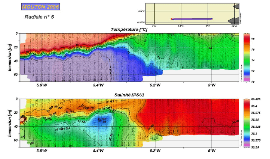
FIG. 3.2: Temperature and salinity cross sections obtained on the 16 th of August 2005 (MOUTON2005 campaign).
