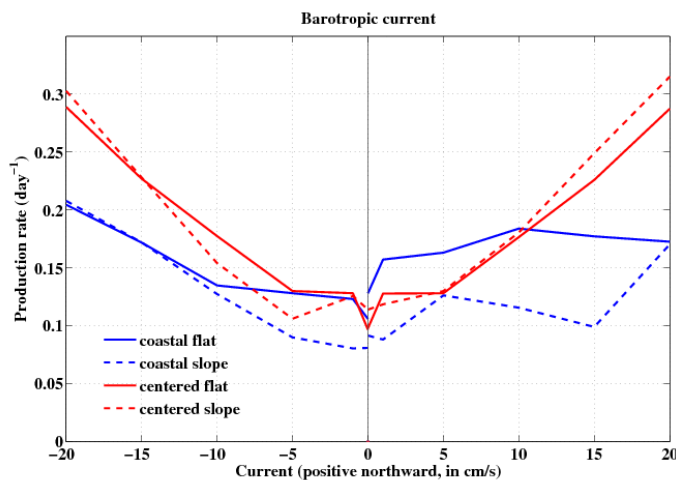
FIG. 3.39: Mean production rate \bar{\tau}_{prod} as a function of negative and positive (Northward) barotropic current V0 for different configurations : centered (red curves) and coastal (blue curves) , with and without a sloping bottom (respectively dashed and plain lines).
