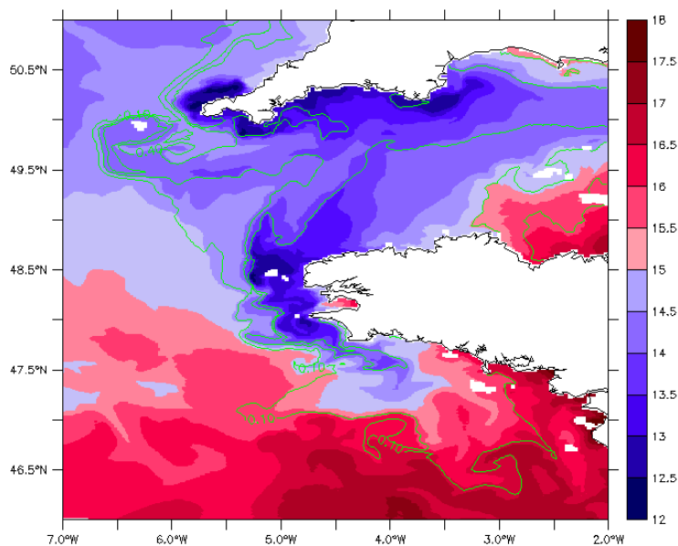
Temperature T=21799, Surface
