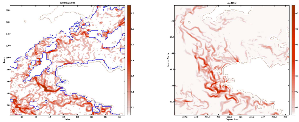
(c) NOAA-NARR SST, limites frontales, le 21.09.2009
