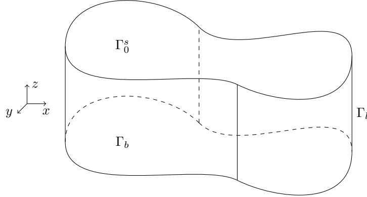
Figure 4.1: The domain \Omega_0 for \alpha > 0 .
