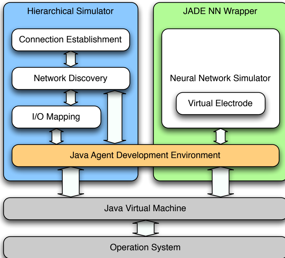
Figure 4.11: Hierarchical Simulator Architecture.
