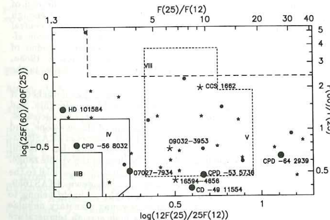
Figure 1: IRAS colour-colour diagram for all observed sources. Large filled circles represent detections with spectra uncontaminated by CO emission from interstellar clouds, large stars represent detections where the spectra also include emission from interstellar clouds, and the small circles and stars are the corresponding non-detections. Fluxes ( J_y ) are taken from the IRAS-PSC catalog without colour correction. The units are \nu F_\nu ratios. For reference, we have drawn van der Veen and Habing's (1988) regions boundaries, the location of most HII regions and galaxies (long dash), and the area containing the major part ( \sim 75\% ) of IRAS-PSC sources identified as planetary nebulae in the PK catalog (short dash).
