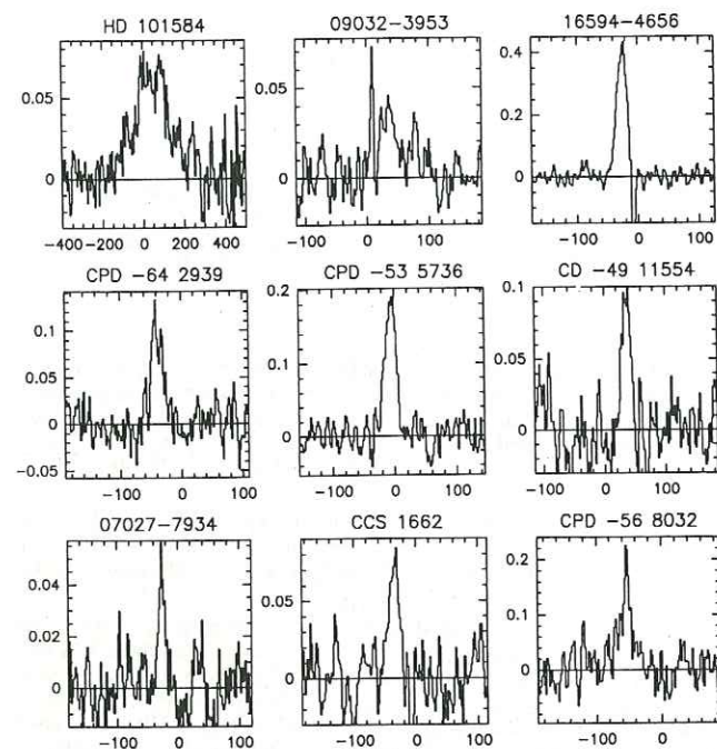
Figure 2 : ^{12}\text{CO}(1-0) spectra for the detected sources, in units of main beam brightness temperature ( T_{MB} ). IRAS09032-3953 is only tentatively detected. The observational results are listed in Table 1.
