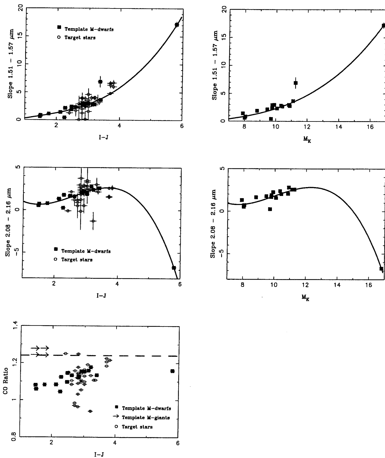
FIG. 2.33 - (1.51 - 1.57)\mu\text{m} and (2.08 - 2.16)\mu\text{m} slope as a function of I-J colour for our target and template sample and as a function of M_K for the template. CO ratio as a function of I-J colour
