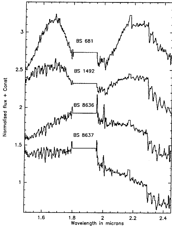
FIG. 2.30 – IRIS HK echelle spectra for the giant template objects of Table 2.11. The spectra are normalized by their flux between 2.22 and 2.25 \mu\text{m}
