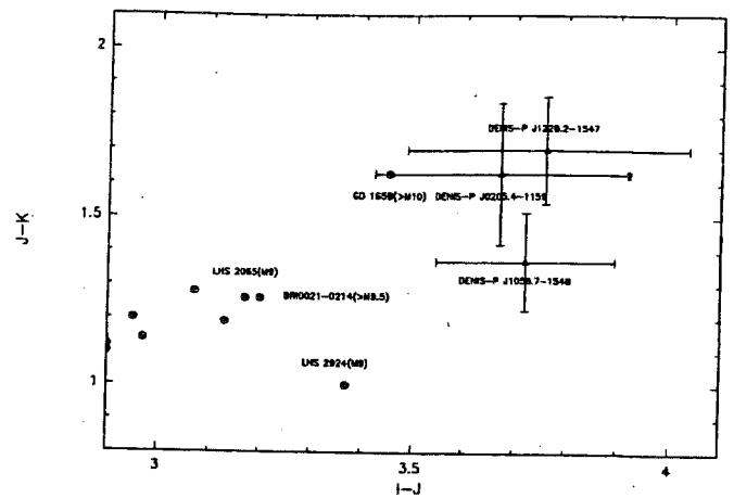
Fig. 1. The I–J/J–K diagram for the three redder DENIS objects. Symbols are: circle: previously known very low mass-stars, triangle: new DENIS objects
