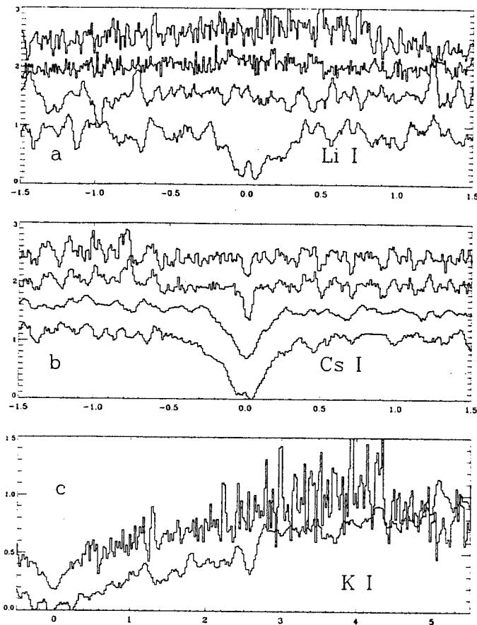
Fig. 1. a The resonance Li I line 670.8 nm region in (from top to bottom with offsets of 0.5) Gl 406 (dM6), LHS 2924 (dM9), DENIS 10-15 and DENIS 12-15. Wavelengths are in nm from line center. The DENIS-P objects are boxcar smoothed by 5 pixels. b Same as above but for Cs I 852.1 nm. Note the progression in the strength of the Cs I feature towards cooler T_{\text{eff}} . c The KI 769.9 nm line of Gl 406 and DENIS 10-15 normalized at 770.5 nm (no offset). The width of this line is so large that it exceeds the coverage of the echelle order.
