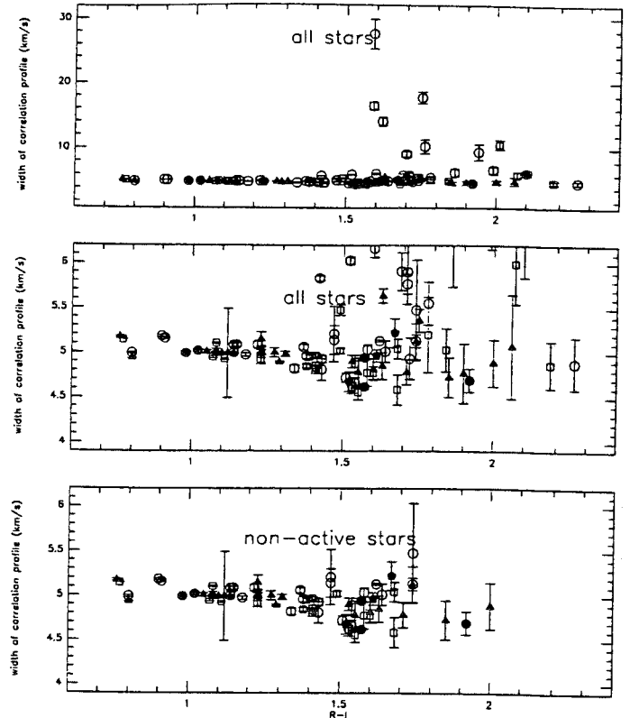
Fig. 1. 1/e half-width of the correlation profile as a function of the (R - I)_c color index for a) and b) all stars, and c) the non-active stars (no H_\alpha emission) only. Symbol codes are: open circles for the young disk, open squares for the young/old disk, filled triangles for the old disk, filled circles for the halo. Known or possible short period binaries ( P < 30 days) have been excluded in these plots.
