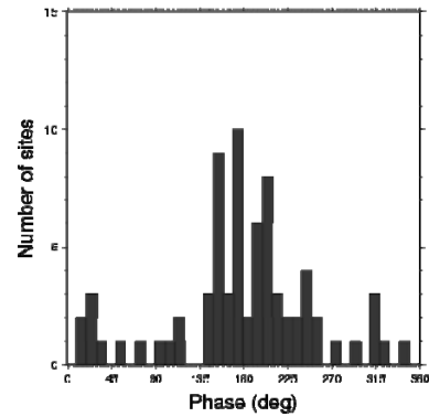
Fig. 9. Histogram of the annual phases observed in the up component time series in Europe with our global network.
