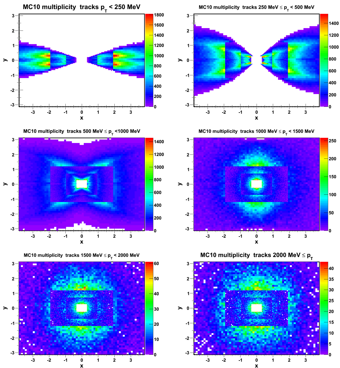
Figure B.1: Track multiplicity map for different transverse momentum ranges with a MC10 minimum bias sample.
