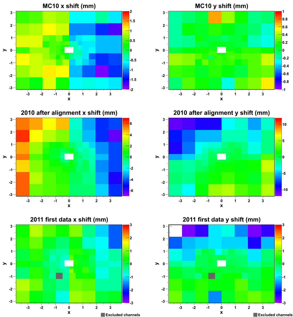
Figure 4.50: Misalignment of the board of PRS respect to the tracking system of LHCb for different measurements. The left column – misalignment in x axis. The right column – misalignment in y axis. The rows from the top: simulation MC10, 2010 data after realignment, 2011 data.
