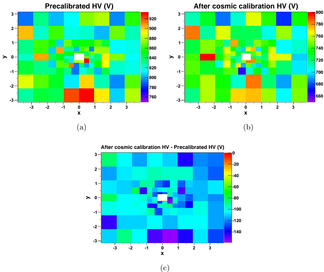
Figure 4.33: High voltage settings before the calibration with cosmic rays (a) – pre-calibration, and after the calibration with cosmic rays (b) – the detector prepared for the first collisions in 2009 with the MPV of 20 ADC counts for MIP. The difference between two is shown in the bottom plot (c).
