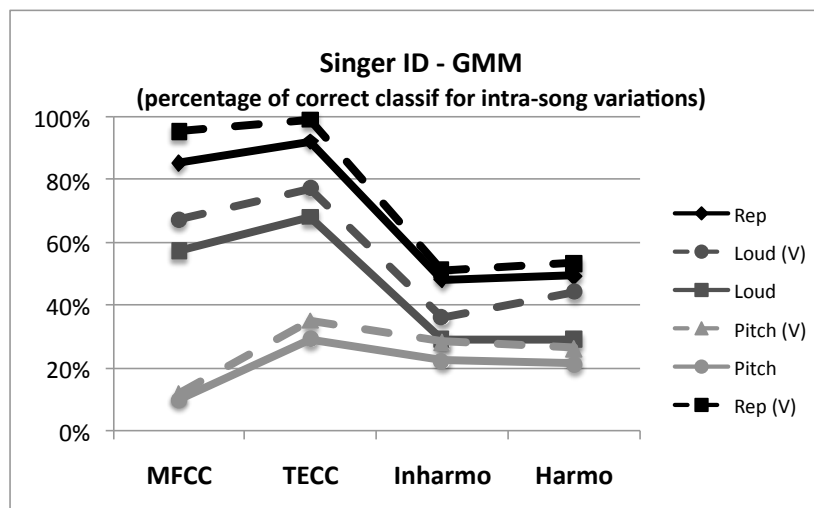
Figure 6.2: Classification accuracy for pitch and loudness variations for GMM. Results obtained after voting (V) are plotted with dashed lines
