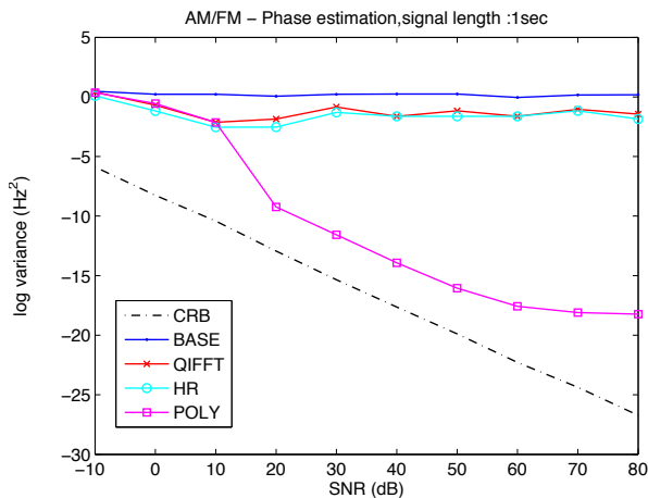
Figure 4.16: CRB - S2 - \phi_0 - (1sec)
