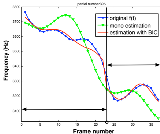
Figure 4.21: Vibrated notes linked + portamento
